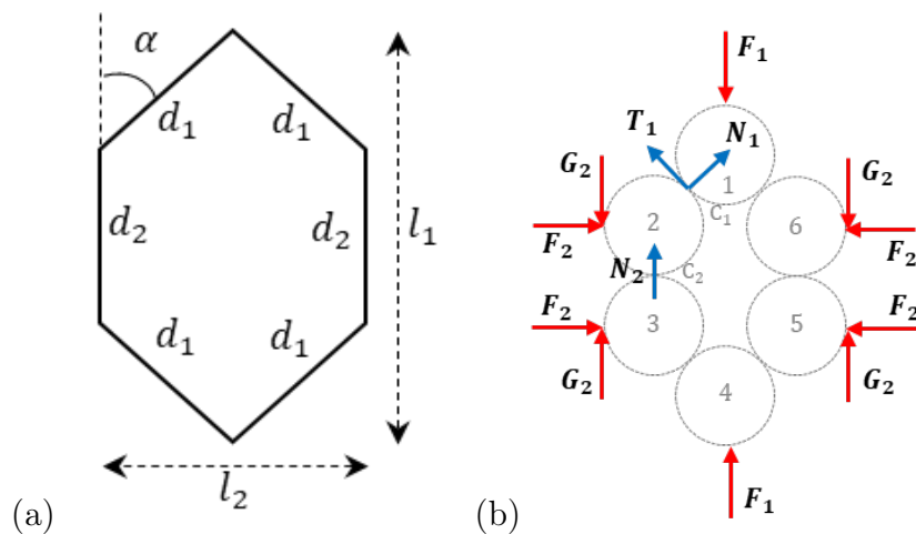
Figure 5.2: The symmetrical description of geometry (a) and forces (b) at the elementary hexagonal pattern of adjoining particles (H-cell). There are two types of contact c_1 and c_2 , the corresponding contact branches are d_1 and d_2 .
