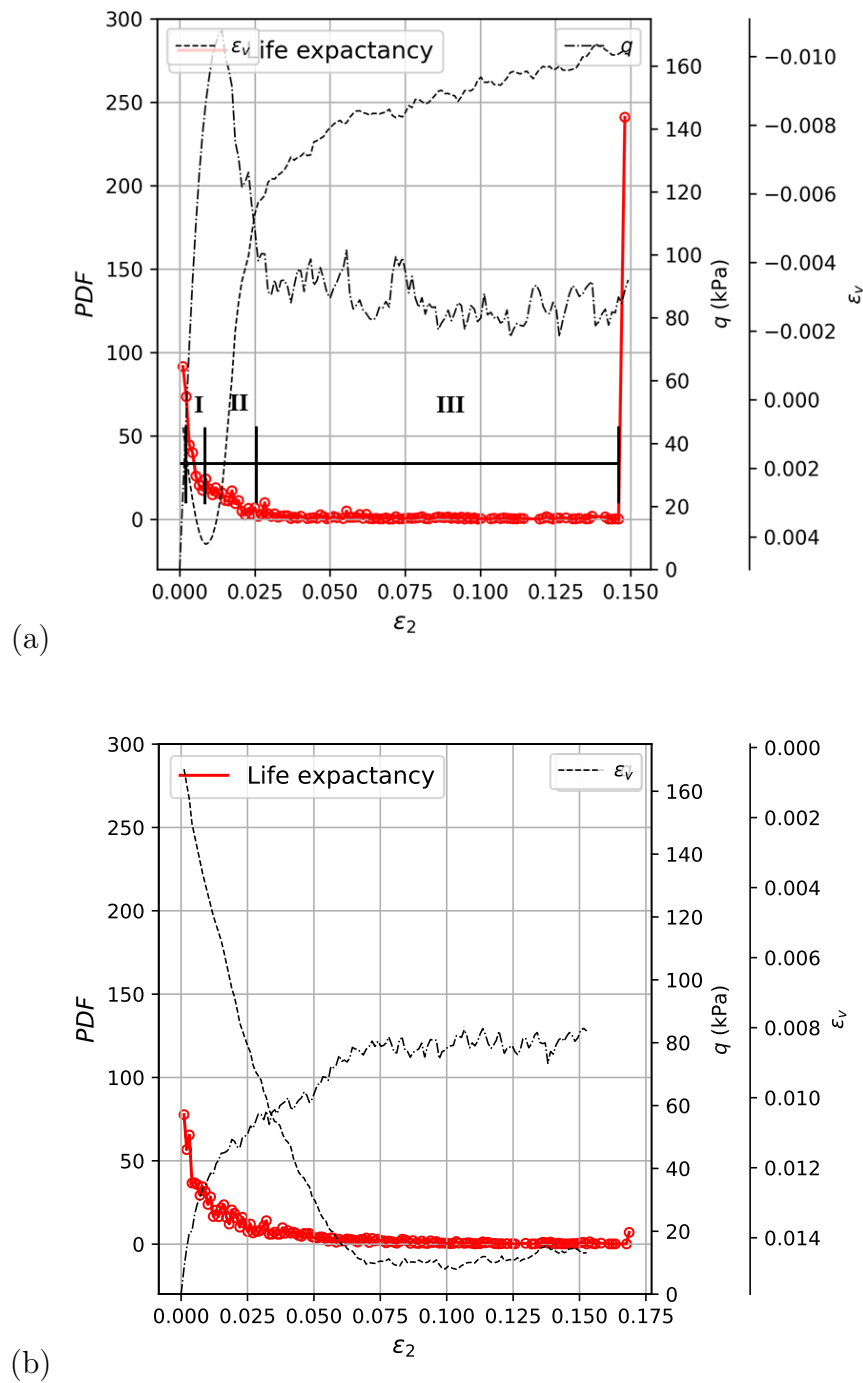
Figure 4.19: Life expectancy PDFs (probability density functions) of chained particles at the initial state of the whole sample in the dense (a) and loose (b) cases. The deviatoric stress curve (dot-dashed line) and the volumetric strain (dashed line) curves are recalled.
