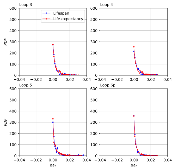
Figure 4.25: The absolute value of PDFs for Lifespan and life expectancy of grain loops under the dilatant proportional strain loading within the domain of the shear band.
