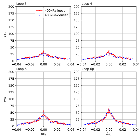
Figure A.2: PDFs for grain loops under two confining pressures: (a) 40kPa, PDFs from the 40kPa-dense are stretched by strain magnitude ratio 1.9; (b) 400kPa, the 400kPa-dense stretched by 3.2.
