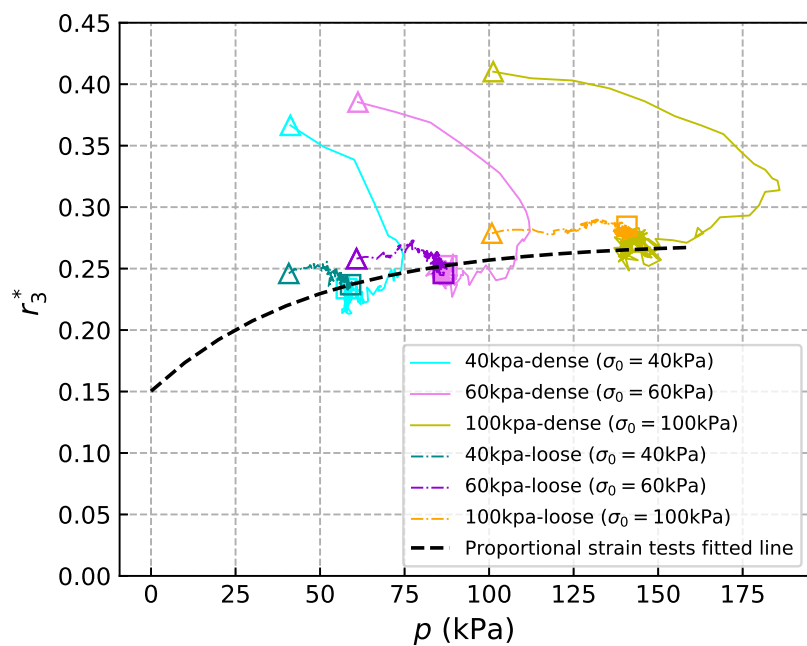
Figure 3.11: p - r_3^* for proportional strain (a) and biaxial (b) test. The start and end points are marked by triangles and squares, respectively. An exponential fit is shown for the dilatant proportional strain tests and repeated on the biaxial tests, as all the proportional strain tests converge towards a master curve.
