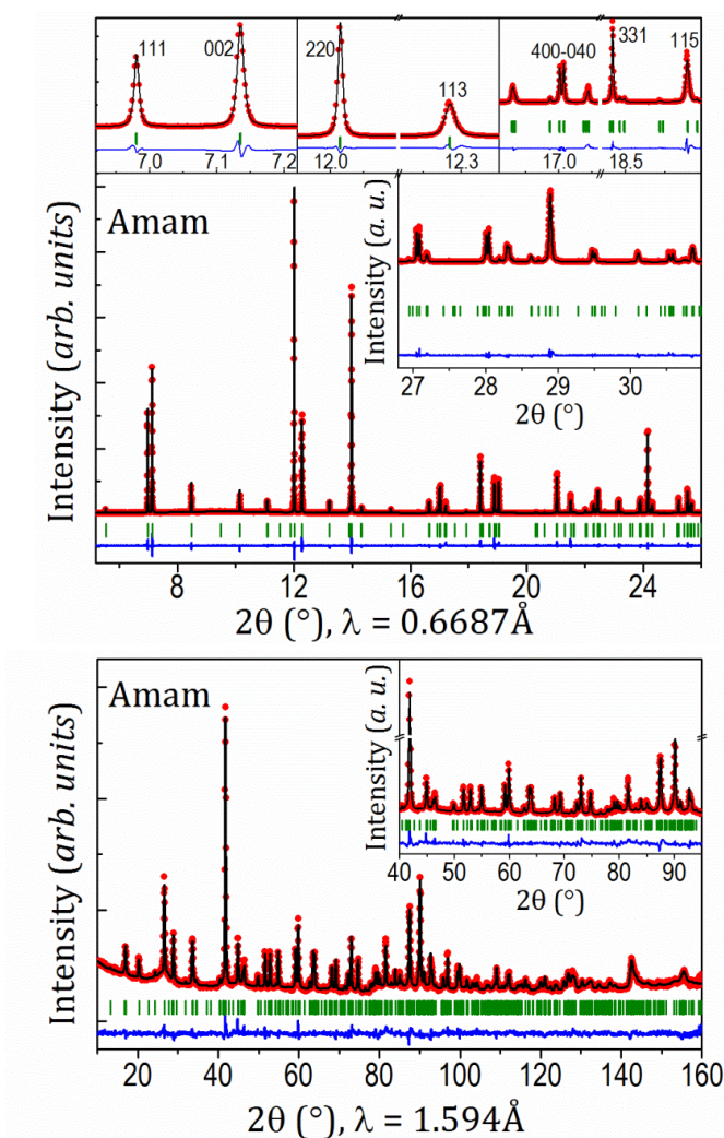
Figure 5.10: Combined Rietveld refinement of synchrotron radiation (top) and neutrons (bottom) diffraction data of \text{Na}_3\text{V}_2(\text{PO}_4)_2\text{F}_3 in the \text{Amam} space group. Insets zoom on significant peaks in the structure.
