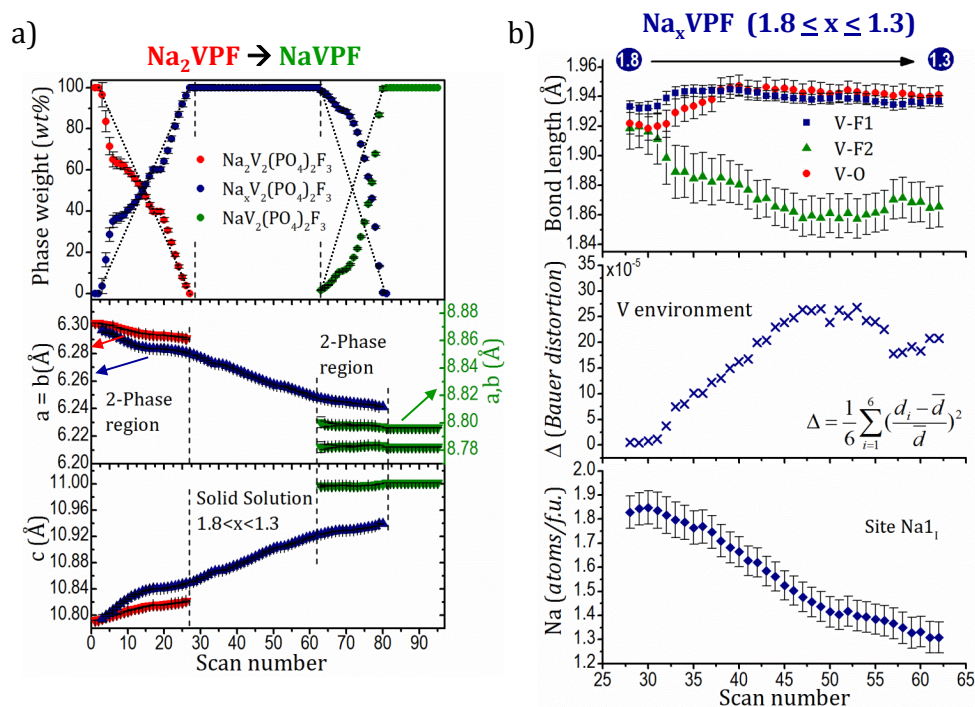
Figure 5.28: a) Parameters obtained from Rietveld refinement during the high-voltage-composition plateau (electrode reacting from composition \text{Na}_2\text{VPF} to \text{NaVPF} ). Unit cell parameters of the different phases and relative percentage in weight are presented. All the phases were described in the space group I4/mmm , except \text{NaVPF} in \text{Cmc}2_1 . b) Parameters obtained from Rietveld refinement (S.G. I4/mmm ) during the solid solution reaction occurring in \text{Na}_x\text{VPF} ( 1.8 < x < 1.3 ). Top: vanadium's bond lengths obtained from refinement of fractional atomic coordinates. Middle: Bauer distortion calculated for \text{VO}_4\text{F}_2 octahedra. Bottom: amount of sodium per f.u. obtained from the refined site occupancy factor in site \text{Na}_{1I} .
