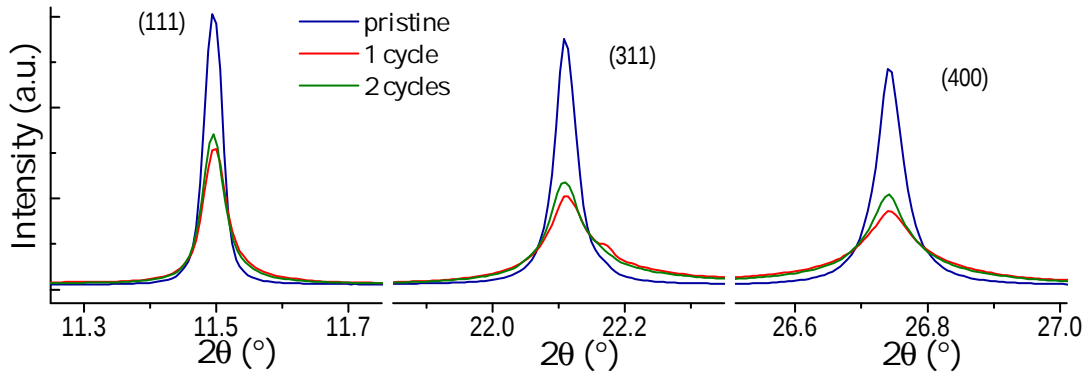
Figure 3.17: (111), (311) and (400) Bragg reflections of LiMn 2 O 4 in the pristine state and after the 1 st and 2 nd electrochemical cycle from operando synchrotron XRPD data. The curve after 1 cycle (red) shows a shoulder on the right side of the (311) peak, due to a reflection of the experimental setup of variable intensity (also seen in Figure 3.15). Note that the cell rotates on its axis during the measure to obtain a better powder averaging.
