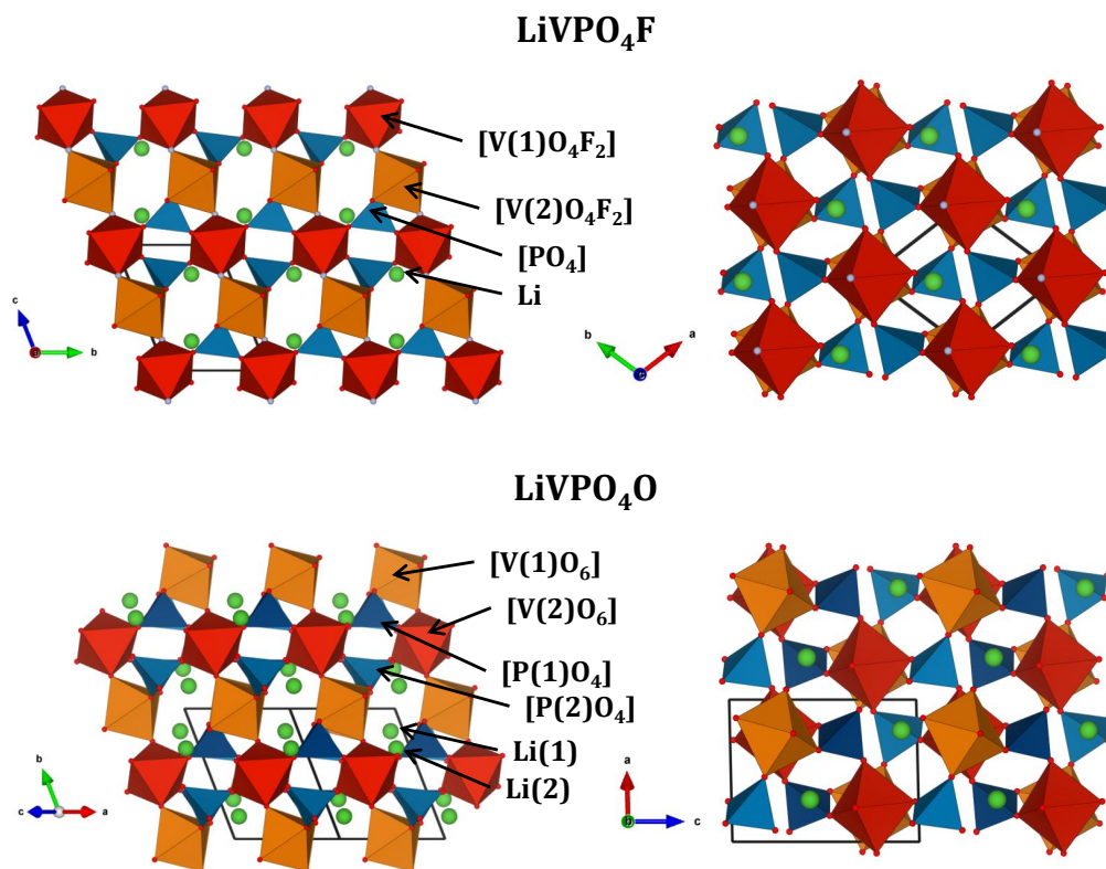
Figure 4.5: Representation of the crystal structures of \text{LiVPO}_4\text{F} and \text{LiVPO}_4\text{O} .
