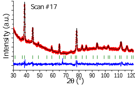
Figure 3.28: Rietveld refinement of scan #17 corresponding to the maximum value of the refined B_{iso} . Wavelength is \lambda = 1.54 \text{ \AA} . Composition is Li 0.68 Ni 0.4 Mn 1.6 O 4 and the respective structural parameters are in Table 3.4.
