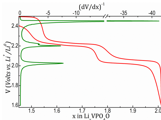
Figure 4.14: Galvanostatic cycling for a mixture of 80 wt% \text{LiVPO}_4\text{O} and 20 wt% Csp (SPEX ball-milled for 30 minutes). Focus on the low voltage region between compositions \text{Li}_{1.5}\text{VPO}_4\text{O} and \text{Li}_2\text{VPO}_4\text{O} .
