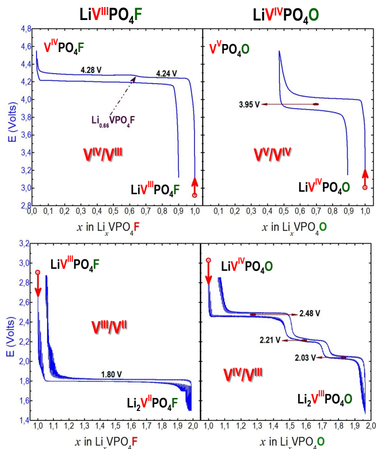
Figure 4.7: Top: Lithium extraction from the structure of \text{LiVPO}_4\text{F} (left) and \text{LiVPO}_4\text{O} (right) upon galvanostatic cycling between 3 V and 4.55 V vs \text{Li}^+/\text{Li} . Bottom: Lithium insertion into the structure of \text{LiVPO}_4\text{F} (left) and \text{LiVPO}_4\text{O} (right) upon cycling (GITT: galvanostatic intermittent titration technique) between 3 V and 1.50 V vs \text{Li}^+/\text{Li} . Adapted from [271] .
