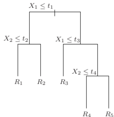
Figure 2-7: Decision tree corresponding to the partition in figure 2-6. Figure adapted from [111].
