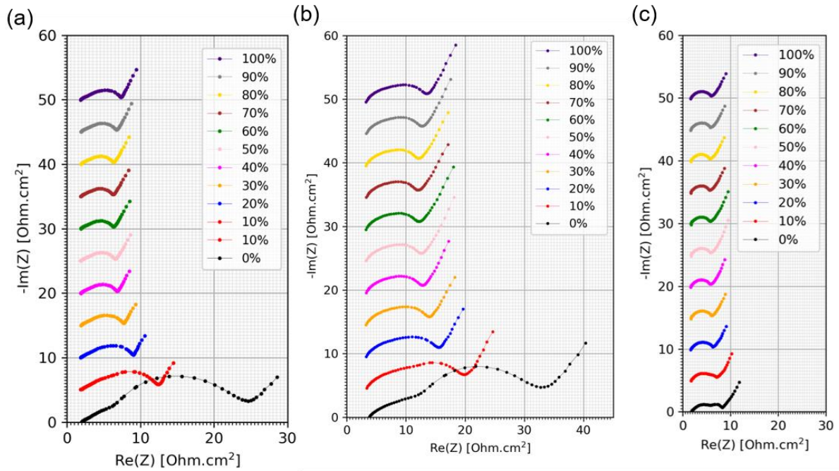
Fig. 25: EIS spectra of the 4-electrode pouch cell in Nyquist plot at different SOC: (a) negative electrode (graphite), (b) full cell and (c) positive electrode ( \text{Ni}_{0.6}\text{Mn}_{0.2}\text{Co}_{0.2}\text{O}_2 ), with a shift of 5 ohm.cm 2 between two successive SOC
