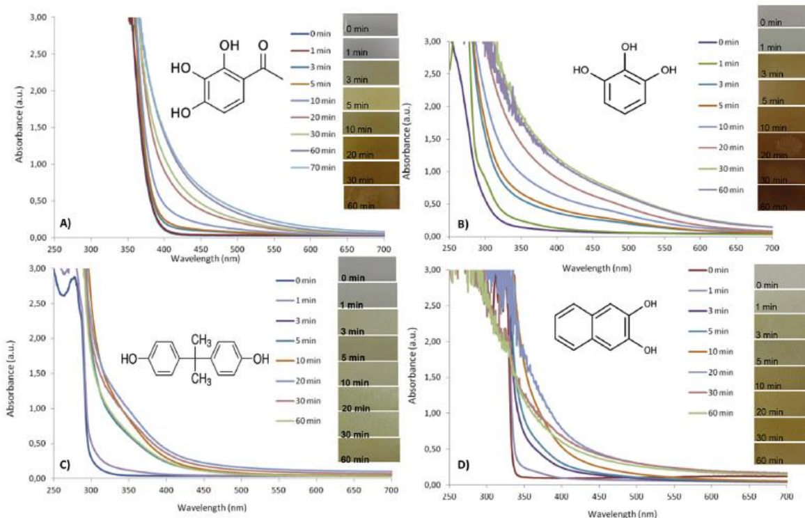
Fig. 1. Evolution of the UV-VIS spectra of the reactants mixtures with UV irradiation time for the different organic precursors: A) Gallactephenone (GA); B) pyrogallol (PG); C) bisphenol A (BP), and D) 2,3-dihydroxynaphthalene (DN). (A colour version of this figure can be viewed online.)
