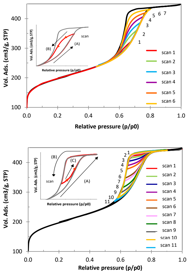
Figure 3.7. Scanning N 2 adsorption/desorption isotherms at -196 °C of sample C-PG. (a) primary desorption scanning curves (partial pore filling); (b) secondary adsorption scanning curves (partial pore emptying). Inset: schematic representation of the emptying/filling mechanisms in both cases.
