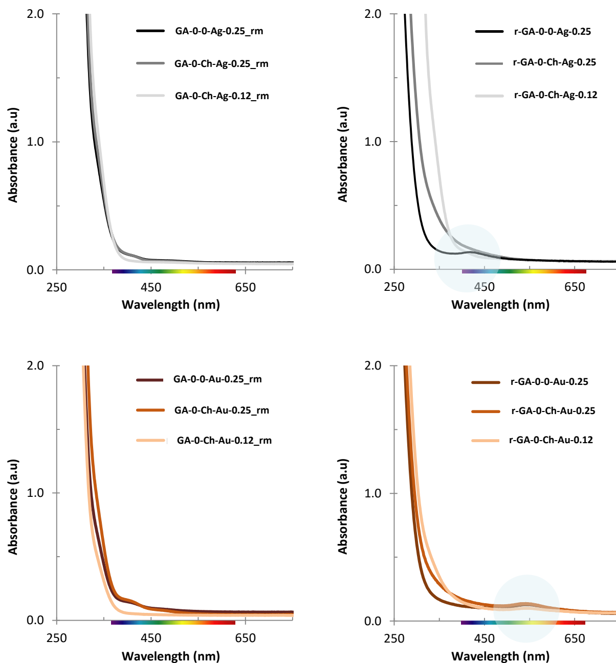
Figure 6.2.2 UV-VIS spectra of metal-containing GA reactant's mixtures before (series rm) and after 60 minutes of UV irradiation (series r).
