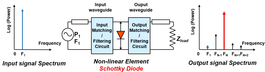
Figure 1.8: A schematic view of a frequency multiplier
