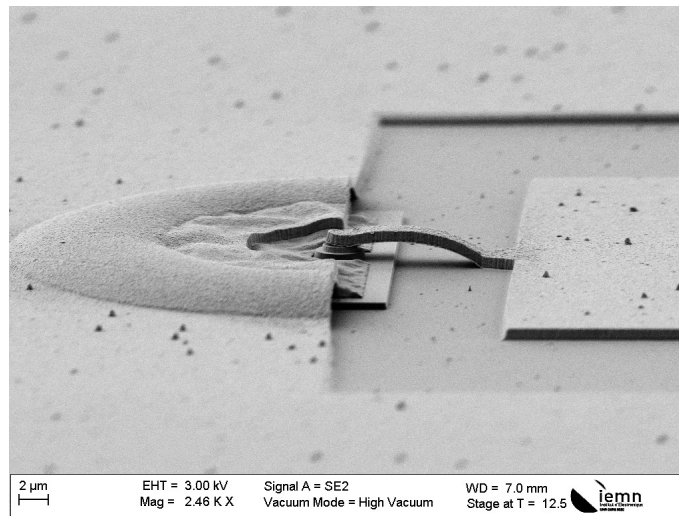
(a) GaN Schottky diode with diameter of 2 μm
