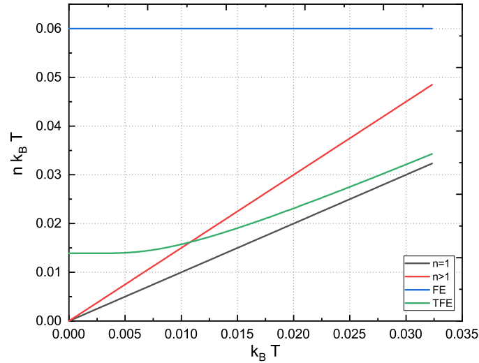
Figure 3.4: Theoretical nk_B T vs k_B T plot, detailing the case of ideal thermionic emission ( n = 1 ), non-ideal thermionic emission ( n > 1 ), FE and TFE
