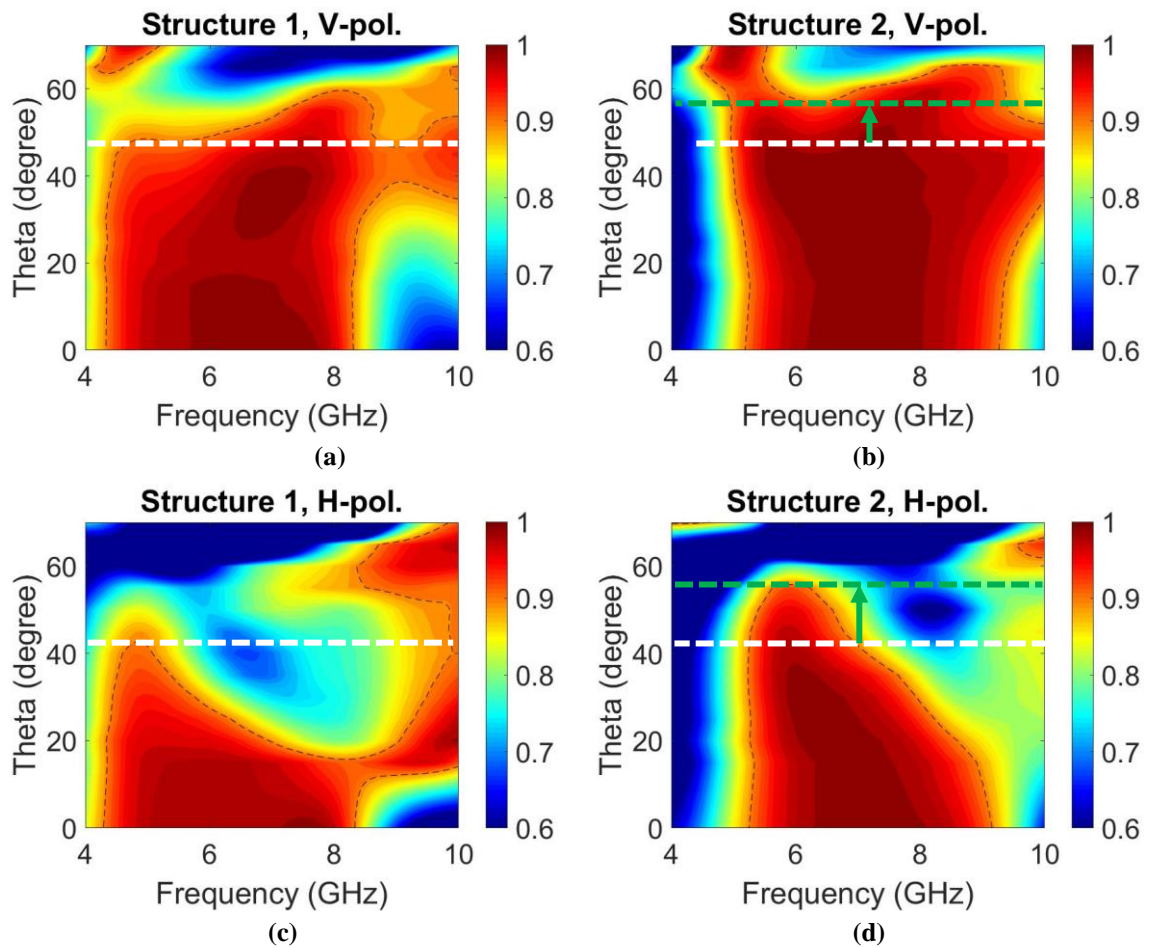
Figure 71. Measurements (with the new setup at TRT) comparison of frequency and theta dependences of the absorptance for Structure 1 for (a) vertical polarization (V-pol.) and (c) horizontal polarization (H-pol) and for Structure 2 for (b) V-pol. and (d) H-pol.. For V-pol., Structure 2 has a 1.7 stronger dielectric, which is 30% more robust than Structure 1. For horizontal polarization, the overall response of Structure 2 is more robust than for Structure 1. The black dashed line corresponds to an absorptivity value of 0.9. The dashed horizontal lines correspond to the maximum angle at which the absorptivity is greater than 90% for Structure 1 (in white) and Structure 2 (in green).
