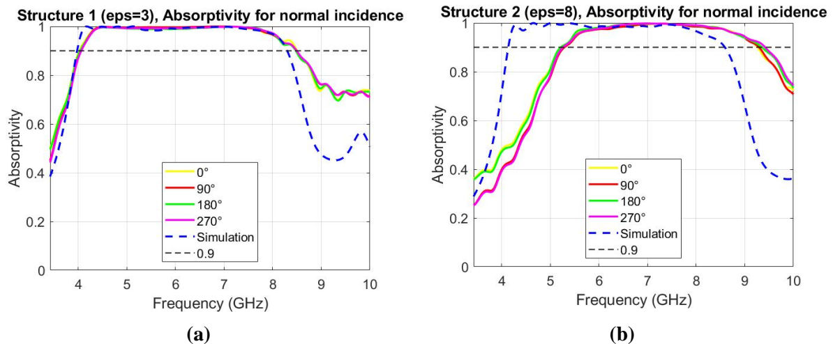
Figure 60. Comparison between simulations and characterizations at DMS for (a) Structure 1, where 0^\circ to 270^\circ are \varphi -rotations of the absorber along its normal, and for (b) Structure 2 with the same \varphi -rotations of the absorber along its normal.
