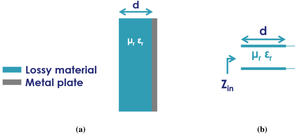
Figure 77. (a) Schematic of the absorber composed of a lossy material of thickness d (in blue), with \varepsilon_r = \varepsilon_r' - j \varepsilon_r'' and \mu_r = \mu_r' - j \mu_r'' , and a PEC (Perfect Electric Conductor) (in gray), and (b) the corresponding transmission line with input impedance Z_{in} , the substrate with its characteristic impedance ( \eta = (\mu_0 \mu_r / \varepsilon_0 \varepsilon_r)^{1/2} ) loaded by a short circuit that corresponds to the metal plate.
