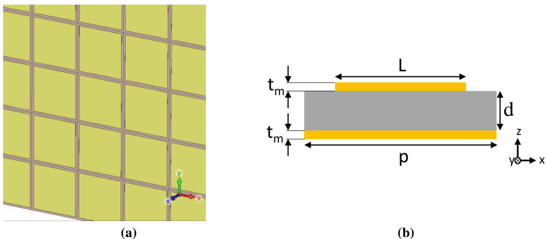
Figure 25. (a) Metamaterial MIM absorber composed of several periods, and (b) schematic cross-section of a MIM unit cell composed of a copper (in yellow) ground plane, a dielectric (in grey) FR4 spacer, and a square copper patch on top.
