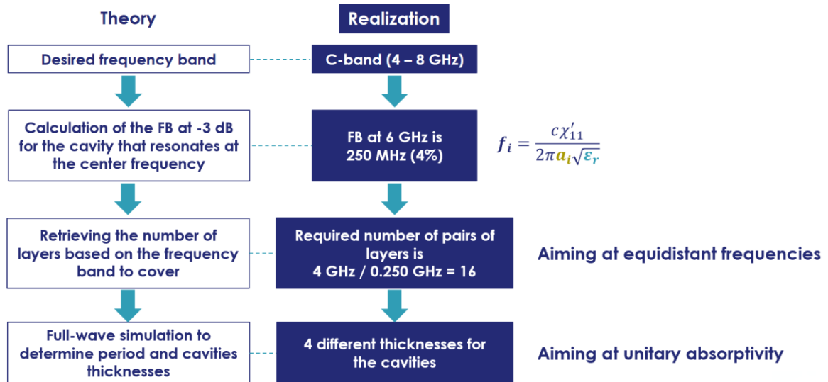
Figure 50. Methodology to follow to design SL absorbers. On the left, the theory while on the right the practical example followed to design the structures of this chapter.
