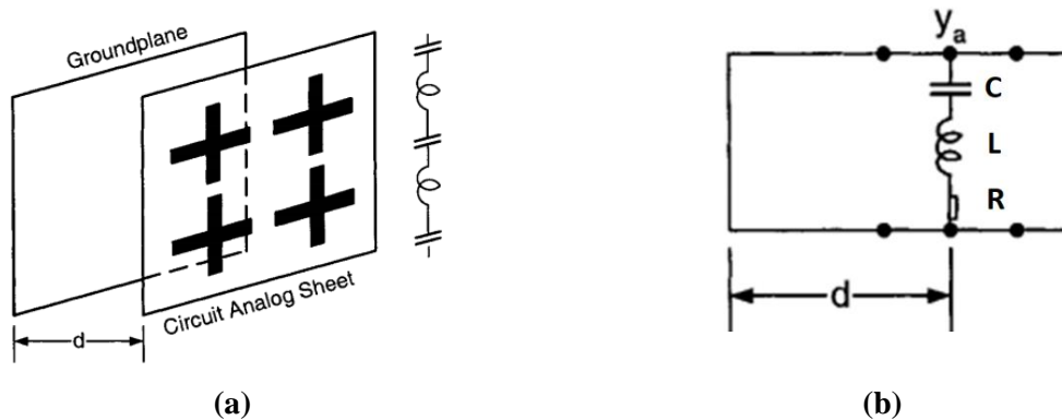
Figure 12. Example of a circuit analog absorber (CAA): (a) Design composed of a ground plane, a dielectric spacer with thickness d < \lambda_g/4 , and the FSS circuit analog sheet with its equivalent circuit. (b) Model of the equivalent transmission line loaded by a short circuit and at the distance d the equivalent circuit of the FSS composed of capacitance (C), inductance (L), and resistance (R) [13].
