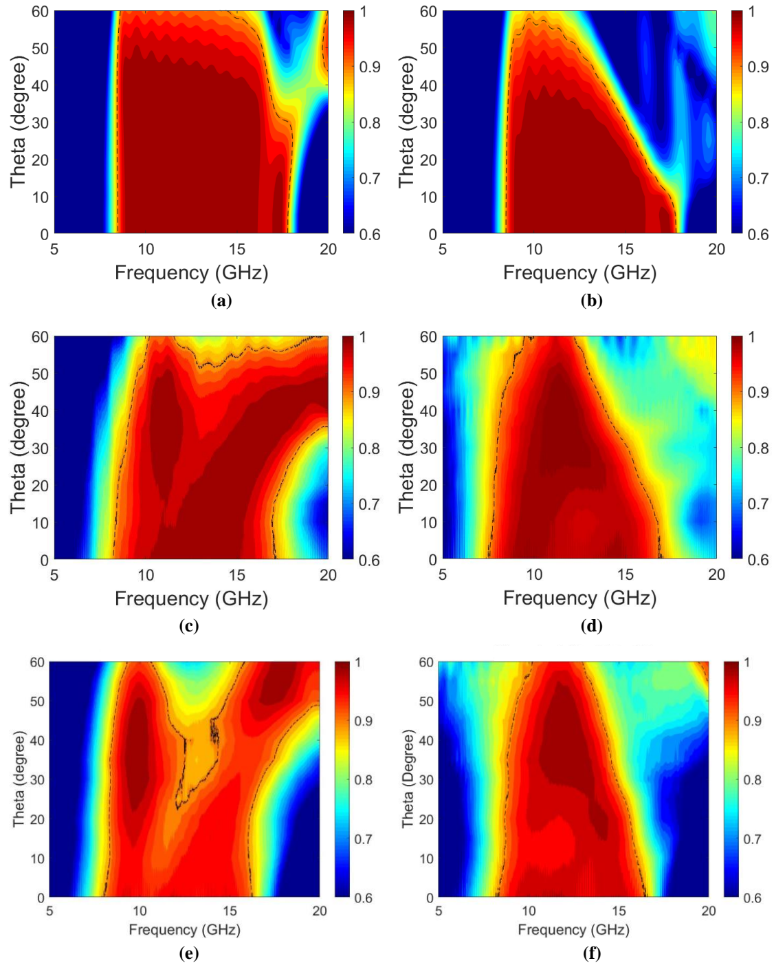
Figure 49. Measurements cartography in NAC (TRT) for different \theta angles from 0^\circ to 60^\circ . (a), (c) and (e) represent simulation, characterization for \phi = 180^\circ and for \phi = 30^\circ , respectively, for vertical polarization. (b), (d) and (f) represent simulation, characterization for \phi = 180^\circ and for \phi = 30^\circ , respectively, for horizontal polarization.
