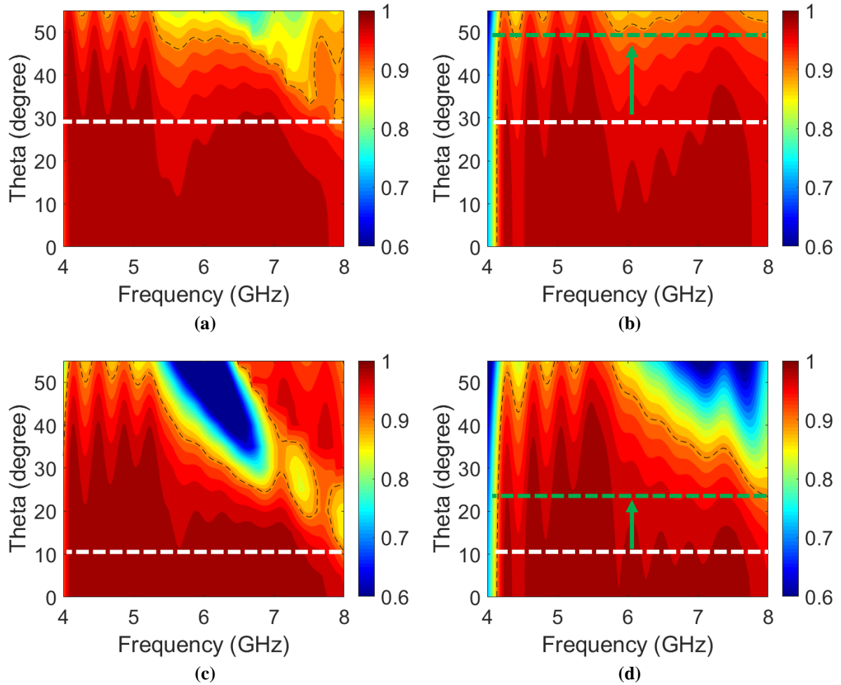
Figure 55. Simulations of frequency and theta dependences of the absorptance for vertical polarization (V-pol.) for (a) Structure 1 ( \epsilon_r = 3.0 ) and (b) Structure 2 ( \epsilon_r = 8.0 ), and for horizontal polarization (H-pol.) for (c) Structure 1 ( \epsilon_r = 3.0 ) and for (d) Structure 2 ( \epsilon_r = 8.0 ). The dashed horizontal lines correspond to the maximum angle at which the absorptivity is greater than 90% for Structure 1 (in white) and Structure 2 (in green).
