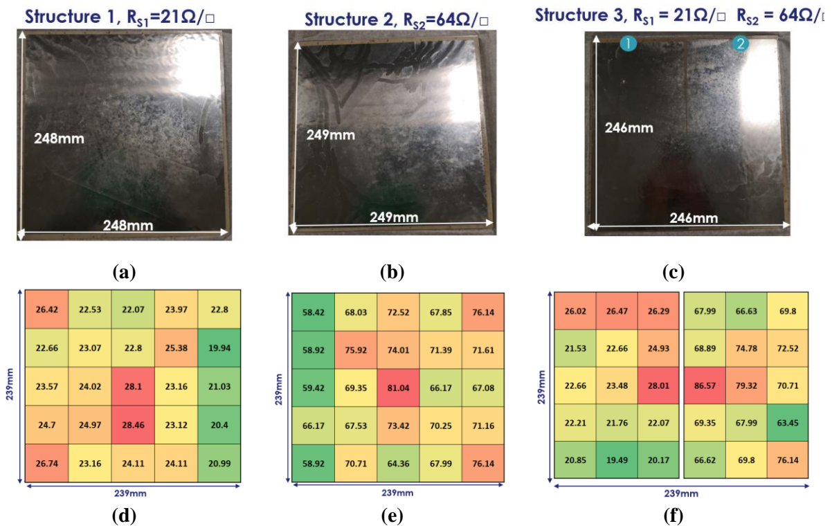
Figure 120. Prototypes fabricated with the electron beam evaporation process. (a) corresponds to Structure 1 with a surface resistance of 21 \Omega/\square , (b) to Structure 2 with a surface resistance of 64 \Omega/\square , (c) to Structure 3 with side 1 and side 2 having the same resistances of Structure 1 and Structure 2, respectively. Cartography of the cells surface resistance values. For each structure, the green color corresponds to the minimum resistive value characterized while the red corresponds to the maximum resistive value.
