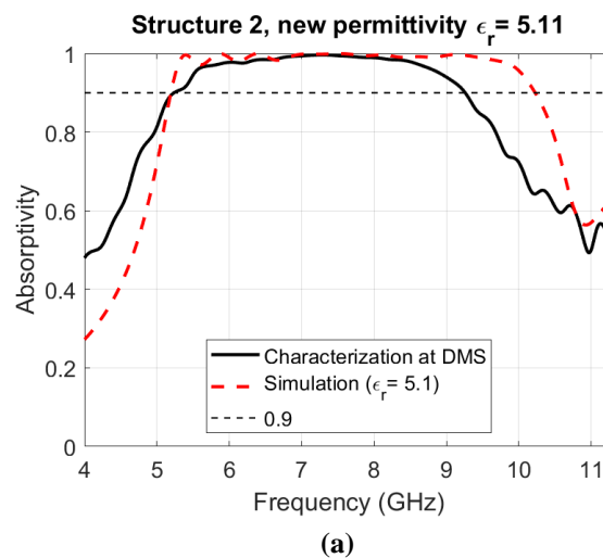
Figure 63. Retro-simulation for Structure 2 with the new permittivity value of the dielectric disks of 5.1 (in red dashed line) and the characterization at DMS (in black solid line) from normal incidence.
