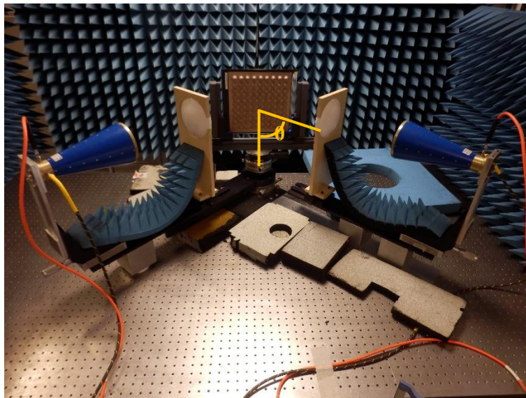
Figure 65. (a) Schematic of the new measurement setup considering one single antenna for simplicity and the labels for the distances reported in Table 6. (b) Bistatic setup picture with two Satimo QR2000 horn antennas and two lenses. Theta \theta definition is reported for clarity.
