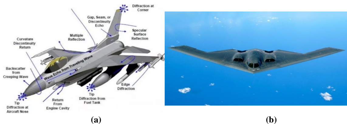
Figure 89. (a) Various types of diffractions from an airplane, (b) stealth-bomber Northrop B-2 Spirit able to reflect the energy of an incoming wave toward the specular direction with its flat surfaces.
