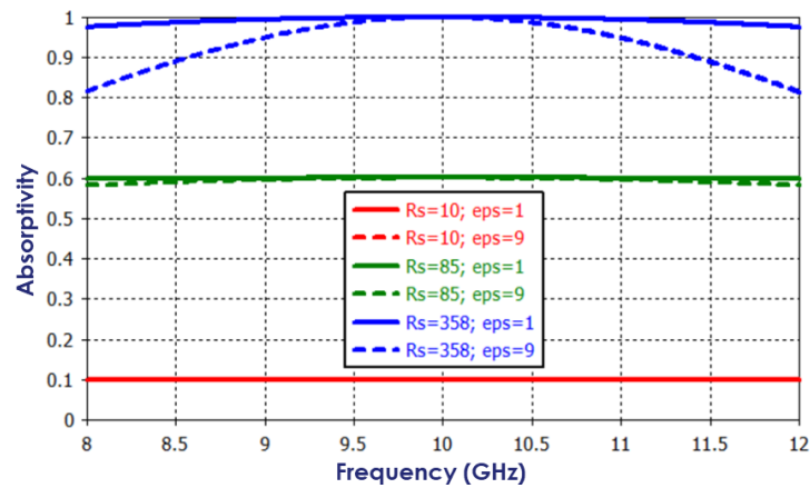
Figure 96. Frequency dependence of the absorptance for three different surface resistances, of 10 \Omega (in red), 85 \Omega (in green) and 358 \Omega (in blues). The solid lines correspond to a permittivity value of 1 (air), while dashed lines correspond to a permittivity value of 9. Increased permittivity enables thinner structure but more frequency selective.
