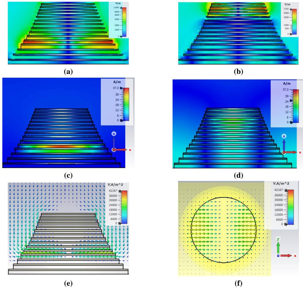
Figure 52. Designs of the two stair-like Structure 1 with a circular shape. Electric field ( \mathbf{E} ) magnitude at (a) 5.5 GHz and (b) 8.5 GHz. Magnetic field ( \mathbf{H} ) magnitude at (c) 5.5 GHz and (d) 8.5 GHz. Poynting vector ( \mathbf{S} ) at 5.5 GHz for (e) vertical cross-section, and (f) horizontal cross-section corresponding to the 5 th bilayer center ( a_{1,5} ).
