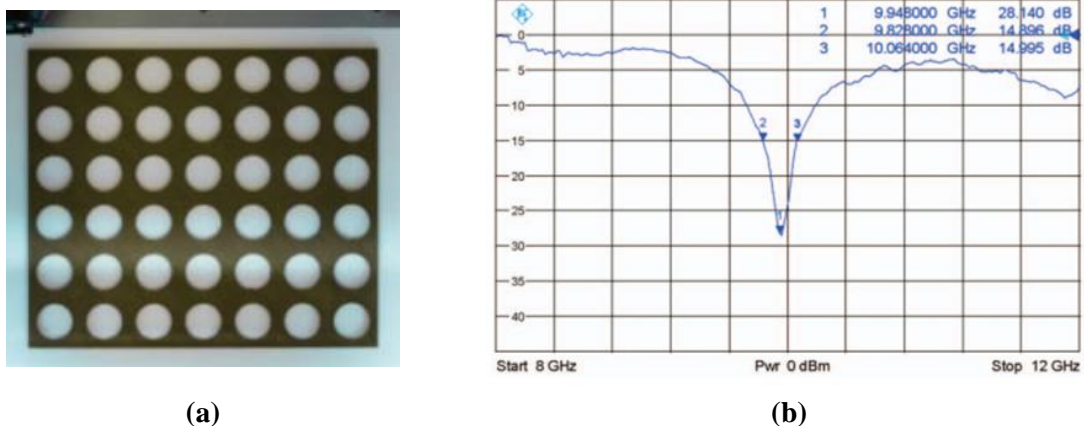
Figure 22. (a) 3D-printed absorber manufactured with Brassfill filament, (b) Modulus of the reflectivity over the frequency for normal incidence [73].
