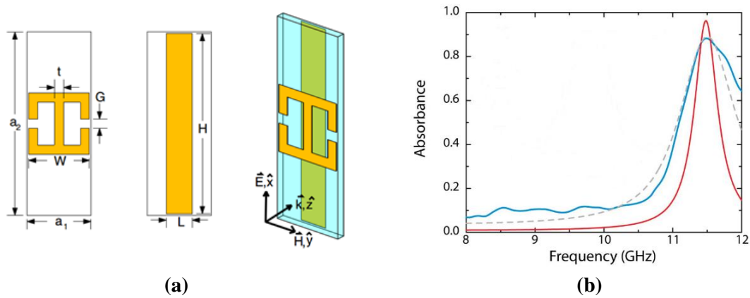
Figure 16. Perfect metamaterial absorber (PMA) (a) basic cell geometry that resonates at 11.5 GHz. (b) Frequency dependence of the absorbance over the range 8 GHz – 12 GHz (measurements in blue and simulations in red). The gray dashed absorbance curve is a Gaussian weighted average that approximates assembly error of the metamaterials absorber, as described in [38].
