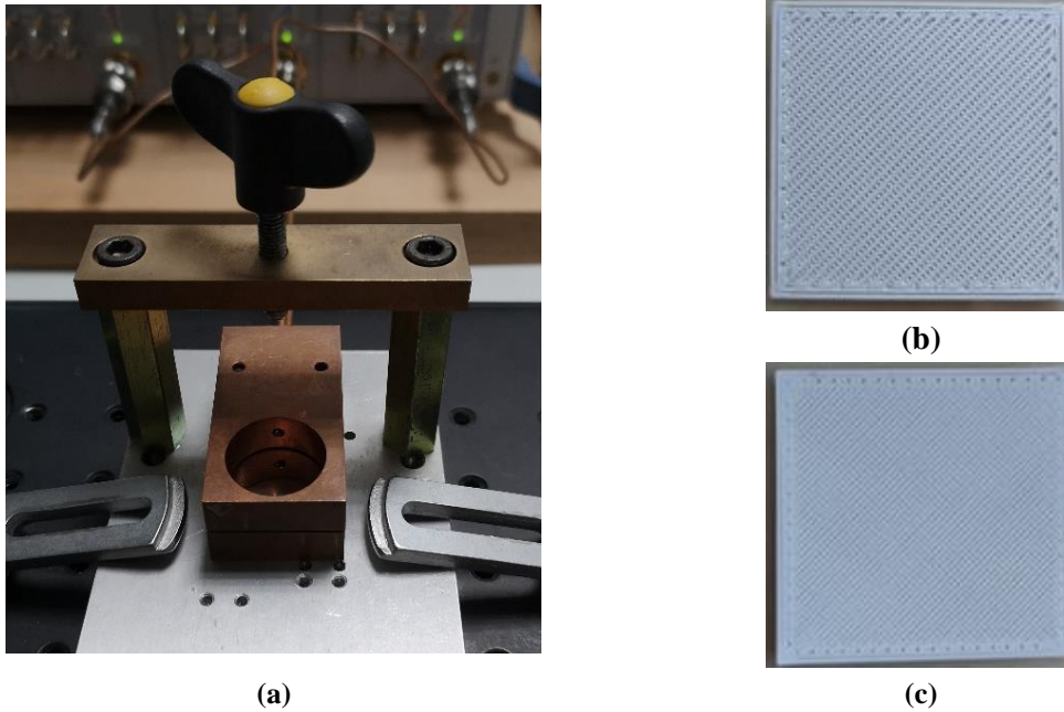
Figure 62. (a) Cylindrical cavity used to measure the permittivity, and (b) front and (c) back sides of the square 25 x 25 mm 2 Preperm DK800 sample.
