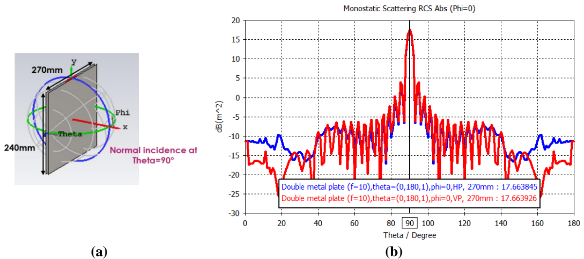
Figure 113. (a) Reference structure composed of two metallic plates of 240 \times 270 \text{ mm}^2 and spaced of 7.5 mm and description of the incident angles \theta and \varphi . (b) simulations of the RCS over the incident angles for vertical polarization (VP) in red, and horizontal polarization (HP) in blues for the reference structure.
