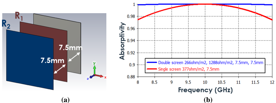
Figure 107. (a) the geometry of the double screen used for the simulation and (b) comparison of the frequency dependence of the absorptance between a single screen of 377 \Omega/\text{m}^2 and two screens with R_1 = 266 \Omega/\text{m}^2 and R_2 = 1288 \Omega/\text{m}^2 , which corresponds to an equivalent impedance of 377 \Omega/\text{m}^2 , over the frequency range 8 - 12 \text{ GHz} corresponding to a FB of 0.4.
