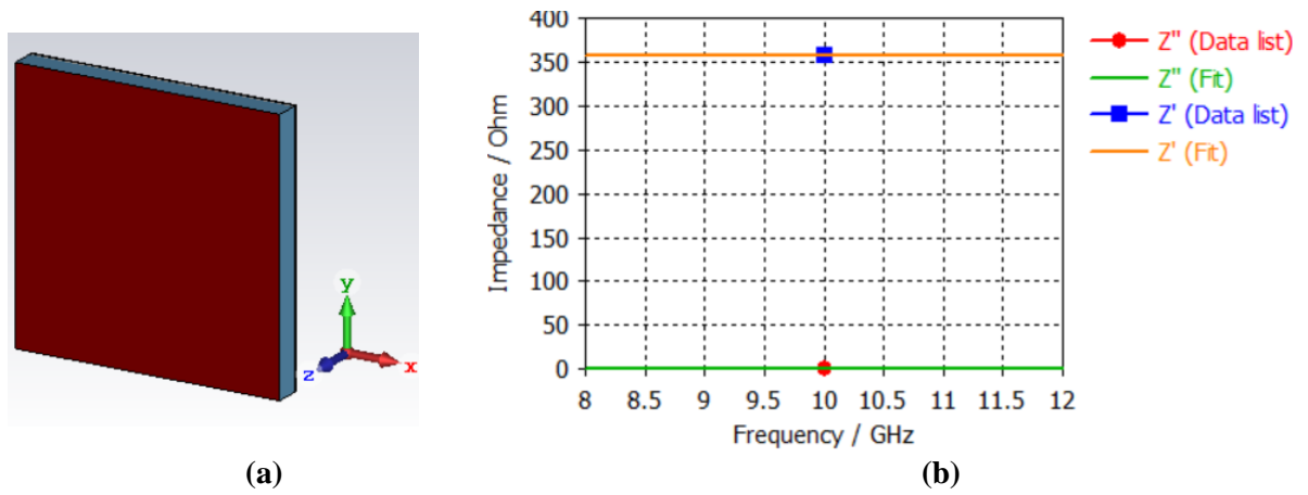
Figure 94. (a) The geometry of the simulated structure with a metal plate at the bottom, air substrate (in blue) in the middle and a resistive screen (in brown) on top of it. (b) Properties of the resistive screen over the frequency with the real part of the impedance Z' (in orange), corresponding to the resistance of 358 \Omega , and the imaginary part Z'' (in green), corresponding to the reactance of 0.1 \Omega .
