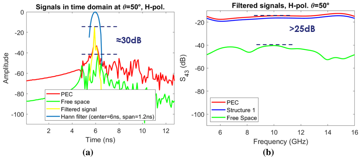
Figure 124. Reflection coefficient of PEC and free space with:(a) signals in the time domain and (b) signals in the frequency domain at the incident angle of 50^\circ . Both have a dynamics of more than 25dB satisfying the criteria of maximum incident angle.
