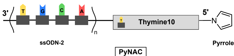
FIGURE 3.27: Model of the PyNAC architecture composed by a ssODN-2 sequence bearing a pyrrole group at the 5'-end separated by a thymine sequence (T10).
