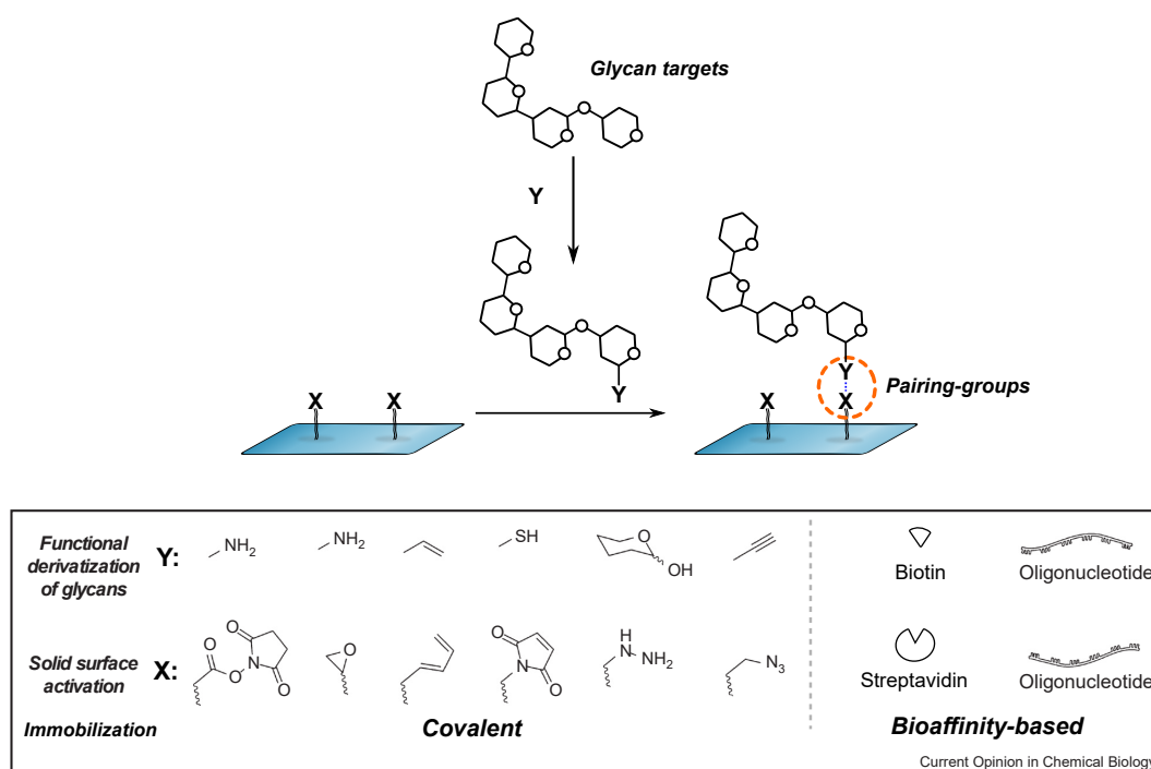
FIGURE 4.6: Immobilization approaches for glycoarrays. Some chemical pairing-groups (X and Y) are depicted. On the top, the functional groups to derivate the glycan structure are depicted (Y). At the bottom, the activated groups on the surface complementary to the glycan derivative (X). Square taken from Song et al. 163
