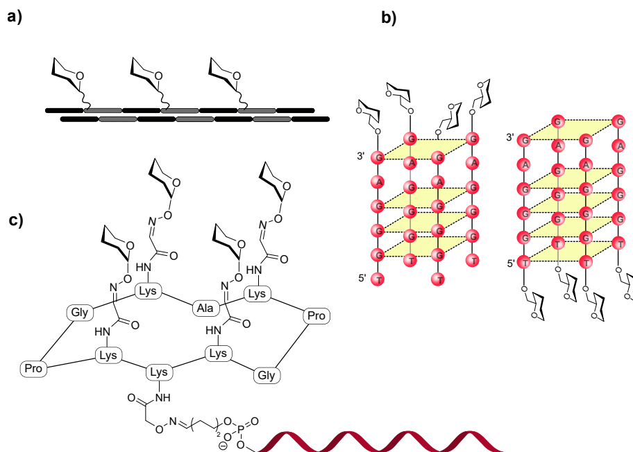
FIGURE 3.1: General approach of different COCs scaffolds. a) COC formed by concatenation of dsDNA scaffold. 82 b) COC using parallel G-quadruplex scaffolds couple with sugars at 5'-end and 3'-end. 80 c) RAFT Glycocluster formed around a cyclic peptide template 79
