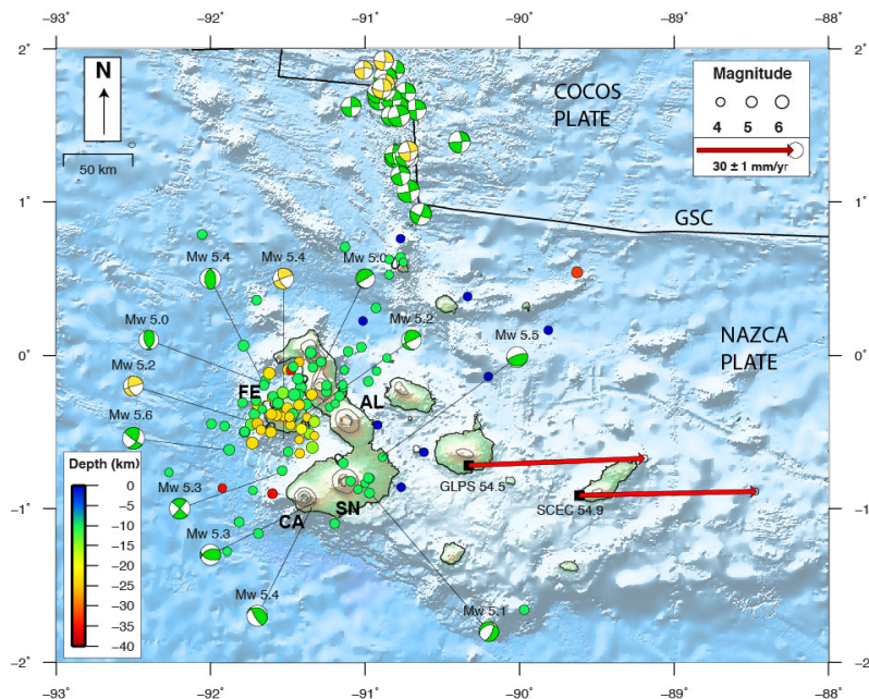
Figure 3.7 – Seismic activity in the Galapagos Archipelago. Mb > 4.0 earthquake reviewed catalog restricted to 40 km depth between 1976 and 2018 is from the International Seismological Centre (ISC) (Engdahl et al. 2020) and Mw ≥ 4.5 focal mechanism solutions are from the Global Centroid Moment Tensor (gCMT) (Ekström et al. 2012). Earthquake depths and focal mechanism depths are depicted by the color scale (bottom left). Red arrows are GPS velocities with respect to stable South America reference frame (SOAM). Ellipses show 95% confidence. SN: Sierra Negra, FE: Fernandina, CA: Cerro Azul, and AL: Alcedo volcanoes. GSC: Galapagos Spreading Center.
