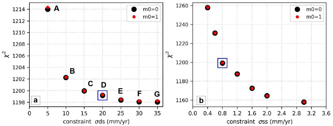
Figure 5.5 – L-curve shows the \chi^2 values with respect to \sigma constraints for a priori models m_{0ss}=m_{0ds}=0 (null coupling) and m_{0ss}=m_{0ds}=1 (full coupling). a) L-curve imposing constraints for a dip slip component ( \sigma_{ds} ) between 5mm/yr and 35mm/yr with fixed values for \sigma_{ss}=0.8 mm/yr, D_{c_{ss}}=1000 km, and D_{c_{ds}}=30 km. b) L-curve imposing constraints for a strike slip component ( \sigma_{ss} ) from 0.4 mm/yr to 3 mm/yr with fixed values for \sigma_{ds}=20 mm/yr, D_{c_{ss}}=1000 km, and D_{c_{ds}}=30 km
