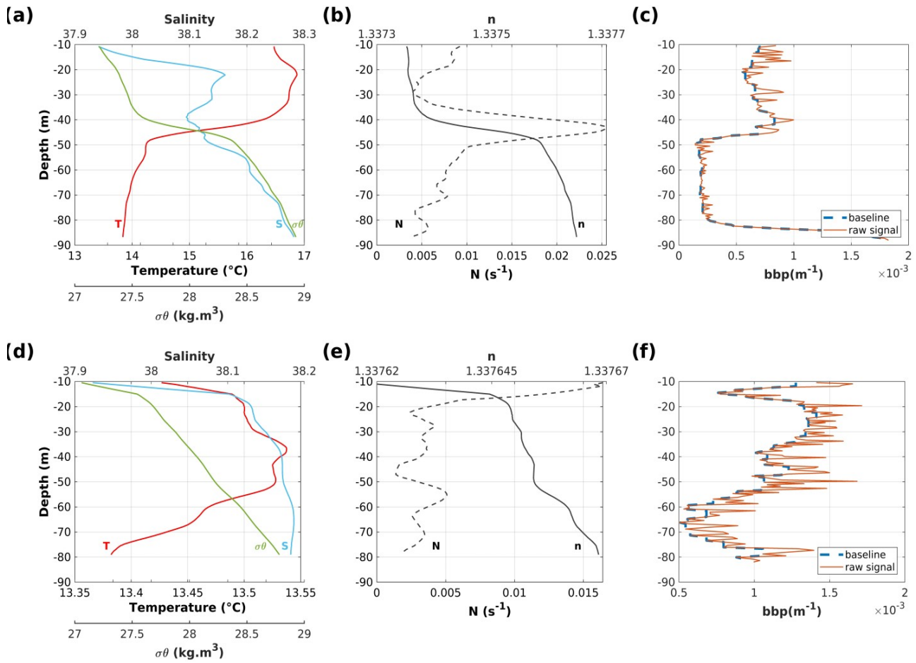
Figure 4.2: (a,d) Water-column profiles of salinity (S), temperature (T), and density ( \sigma_\theta ); (b,e) index of refraction of seawater (n) and Brunt–Väisälä frequency profiles (N); and (c,f) backscattering profiles of \text{bbp}_{700} of Wetlabs BBFL2 (raw-signal) and the baseline extract from a filter 5-point running minimum followed by a 5-point running maximum applied on the \text{bbp}_{700} measurements. The top panels correspond to the autumnal season (November, 2016) showing a seasonal thermocline around 50 m depth characteristic of the coastal area surrounding the Rhone region of freshwater influence (ROFI) area. The lower panels correspond to the winter season, with a homogeneous water column (15–80 m depth), except in subsurface waters due to the Rhone River plume.
