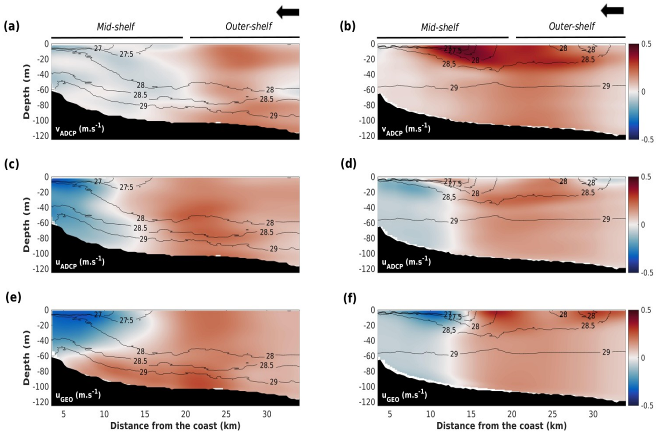
Figure 4.8: Hydrodynamical variables: (a,b) northward velocity, (c,d) eastward velocity, (e,f) and eastward geostrophic velocity. The left panels correspond to the autumnal season, from November 11 to 13, 2016. The right panels correspond to the winter season, from February 5 to 7, 2017. The black arrow at the top of each panel indicates the direction of the glider's motion.
