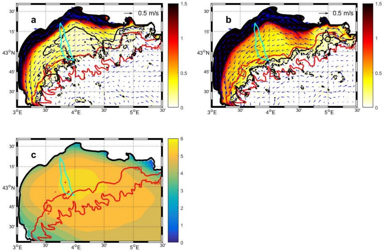
Figure 5.9: (a) and (b) background color: wave-current bottom shear stress ( \text{N m}^{-2} ) averaged between 00:00 and 03:00 h on 1 March 2018 from the simulations using a roughness of 10^{-4} (a) and 10^{-3} m (b). Note that the colorbar has been saturated on the inner shelf to focus on the deeper areas. The black lines correspond to the 0.2 (solid line) and 0.1 (dashed line) \text{N m}^{-2} isolines. The depth-averaged currents are superimposed. (c) Significant wave height (m) calculated by Wavewatch 3 averaged over the same period. For the three maps, the red lines correspond to the 100 m and 500 m isobaths, and the cyan line corresponds to the glider path.
