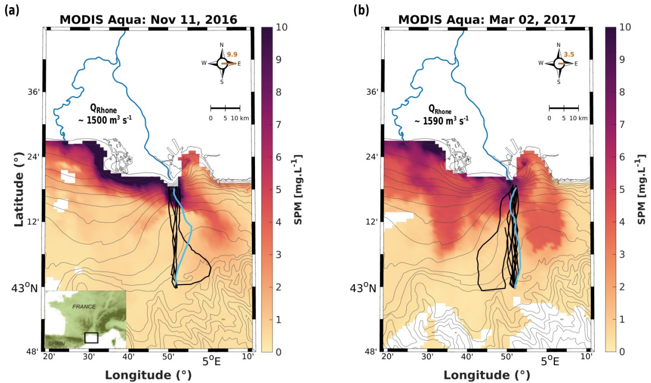
Figure 4.1: Moderate Resolution Imaging Spectroradiometer (MODIS) Aqua images of suspended particulate matter (SPM) concentration for (a) November 11th 2016, with a flow from the Rhone River of about 1500 \text{ m}^3 \text{ s}^{-1} and (b) March 2nd 2017, with a flow of about 1590 \text{ m}^3 \text{ s}^{-1} . Clouds are shown as white patches and wind speed (in \text{m s}^{-1} ) and direction are specified. Depth contours are shown in gray and represent the 10 m isobaths from the coast. The glider track and sections of interest are shown as thick black and blue lines, respectively, for each deployment.
