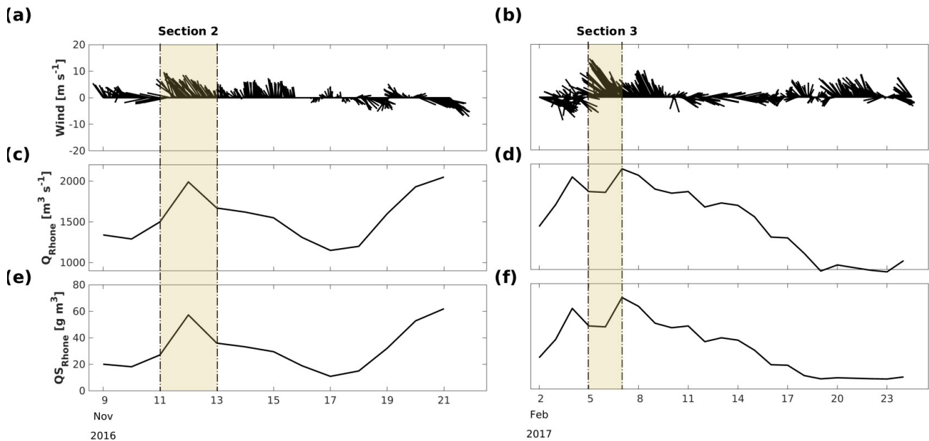
Figure 4.5: Time-series of atmospheric conditions at Cap-Couronne station ( 40^{\circ}20.23'\text{N} ; 5^{\circ}01.38'\text{E} ) for (a) autumnal and (b) winter conditions. Black lines correspond to hourly (10-min burst average) wind speed and direction. By convention, wind direction indicates its origin. The shaded area corresponds to the sections chosen to illustrate hydrological, hydrodynamical, and biogeochemical features.
