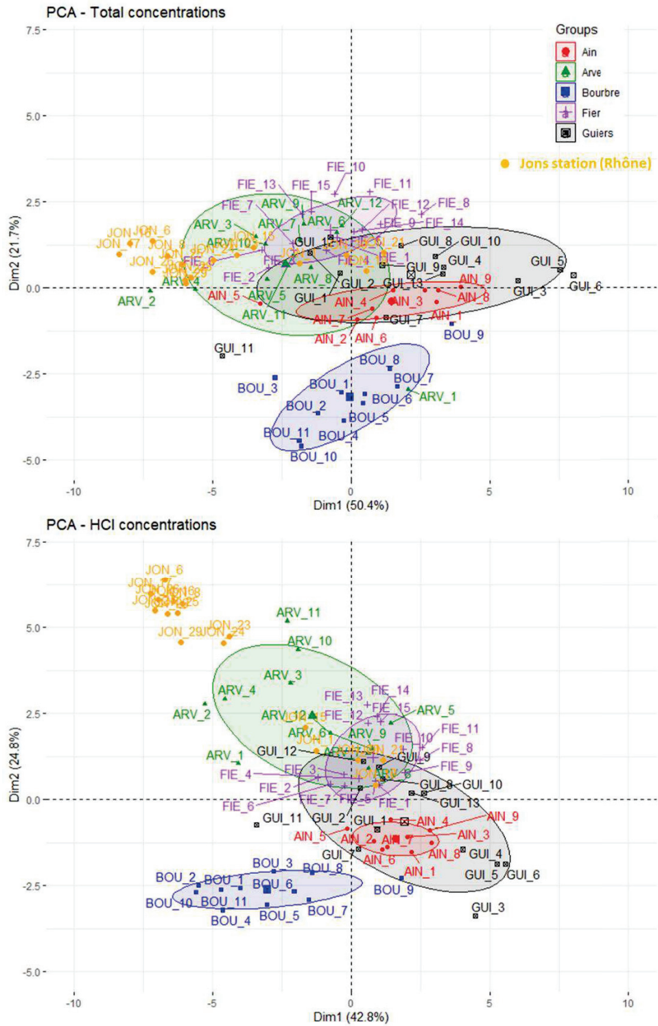
SI 3. Principal component analysis (PCA) of element concentrations in total and 1M HCl-extracted fractions of SPM.
