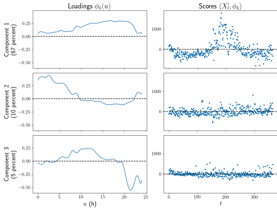
Figure 2.8: fPCA loadings and scores. Each row corresponds to one functional principal component.
