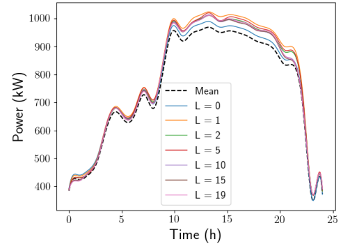
(a) Evolution of \sum_{\ell=-L}^L \|\varphi_{k,\ell}\|_{\mathcal{H}_0}^2 with the number L of lags. (b) Reconstruction with the first harmonic principal component, i.e. \hat{\mu}_{W_i}(u) + \sum_{\ell=-L}^L Y_{1,t+\ell} \varphi_{1,\ell}(u) , with different number L of lags.
