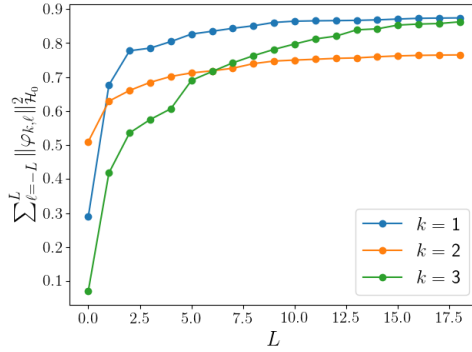
(a) Evolution of \sum_{\ell=-L}^L \|\varphi_{k,\ell}\|_{\mathcal{H}_0}^2 with the number L of lags. (b) Reconstruction with the first harmonic principal component, i.e. \hat{\mu}_{W_i}(u) + \sum_{\ell=-L}^L Y_{1,t+\ell} \varphi_{1,\ell}(u) , with different number L of lags.
