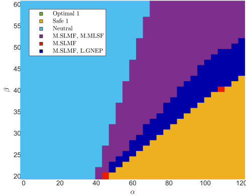
Figure 3.4: Illustrated result of Theorem 3.4.1 for input \mathcal{I}_1 with replacing w_3 = 0.15 .
