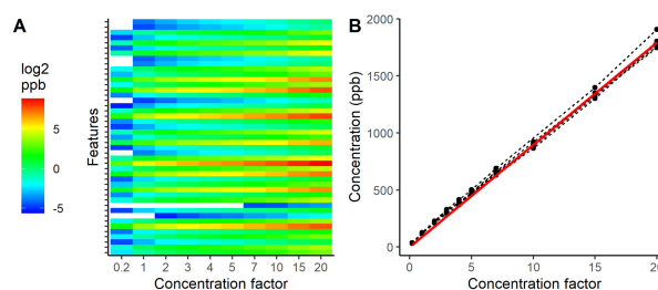
Fig. 2. ptrairMS analysis of a reference VOC mixture. (A) Heatmap of the \log_2 concentrations in ppb of the 45 selected VOCs before the imputation step. (B) The sum of the 45 compounds concentrations for each replicate (dashed line) as a function of the concentration factor. The expected total concentration is shown as a red line
