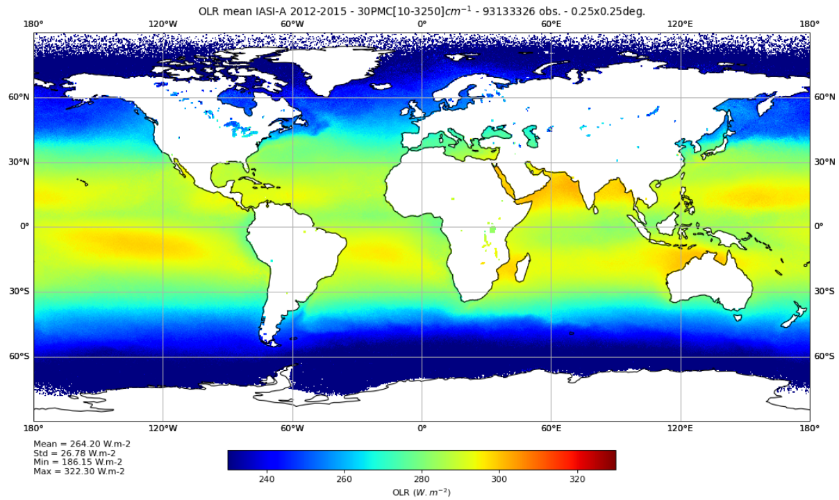
(a) OLR moyen IASI-A
