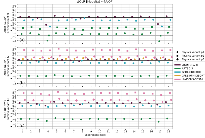
Figure A1. Means and standard deviations of OLR differences (model minus 4A/OP) in \text{W.m}^{-2} , as a function of the experiment index. The five models compared to 4A/OP are represented by colors. The three forcing indices f1, f2 and f3 are represented on individual sub-figures respectively (a), (b) and (c). The different physics variants are differentiated with marker shapes.
