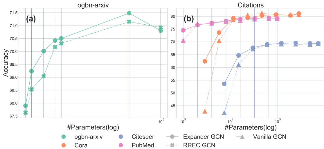
Figure 5.2: (a,b): Accuracy vs. Number of parameters plot on a logarithmic x-axis on (a) ogbn-arxiv for GCN models with different sparsifiers and (b) on CORA/CITSEER/PUBMED for vanilla and Expander GCN under the same parameter budget.
