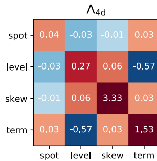
Figure II.3: Four dimensional Kyle cross-impact model on options.
