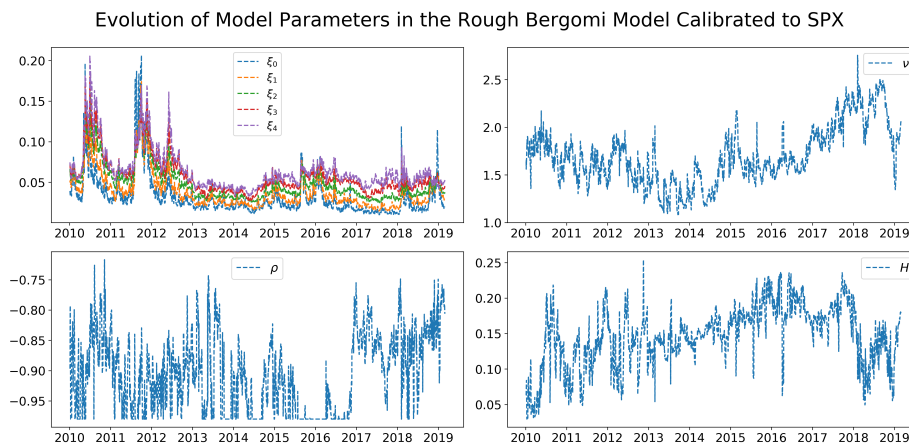
Figure .10: Historical parameter calibration in the grid-based approach.
