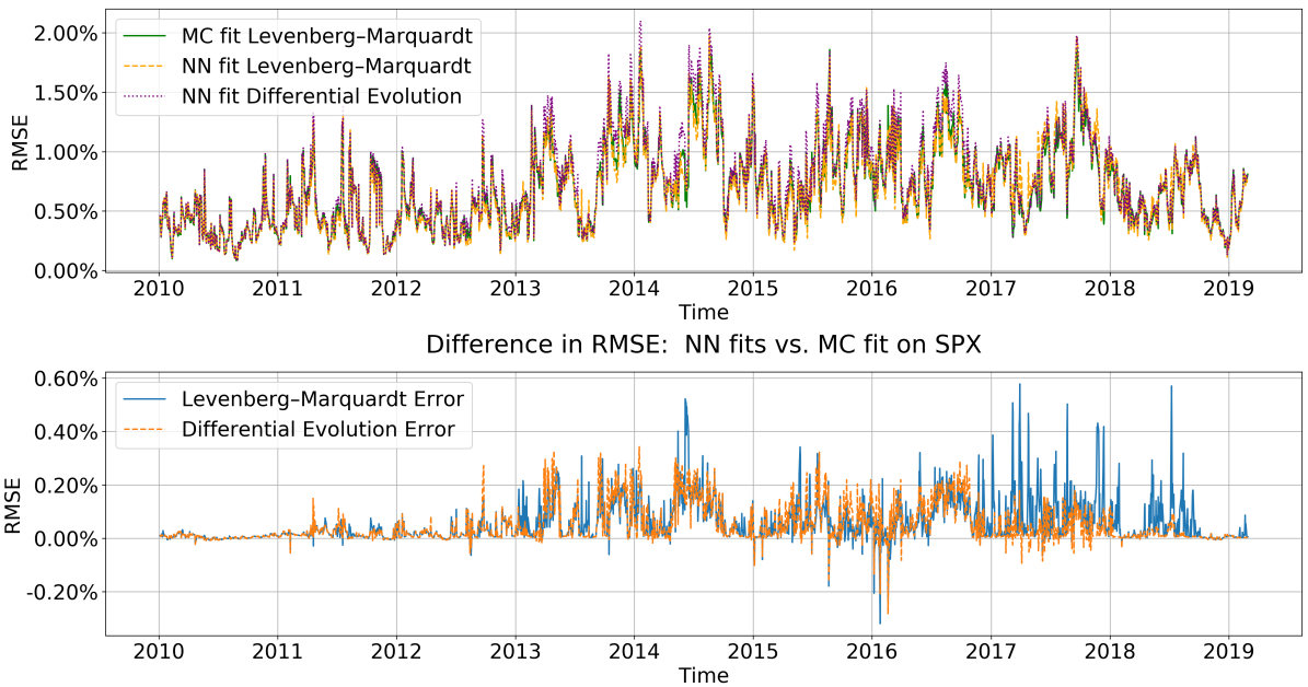
Figure VIA.12: Comparison of quality of fit of different calibration approaches.
