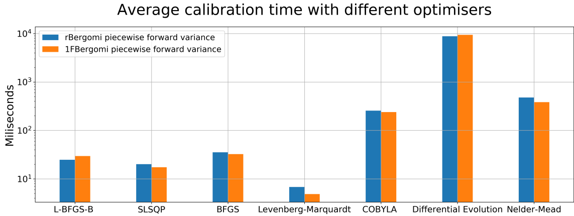
Figure VIA.8: Average calibrations times for all models using a range of optimizers.
