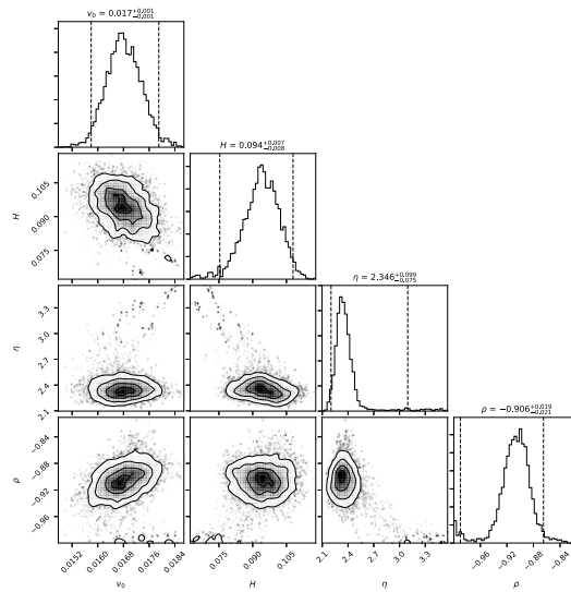
Figure .9: Historical parameter calibration in the pointwise approach.
