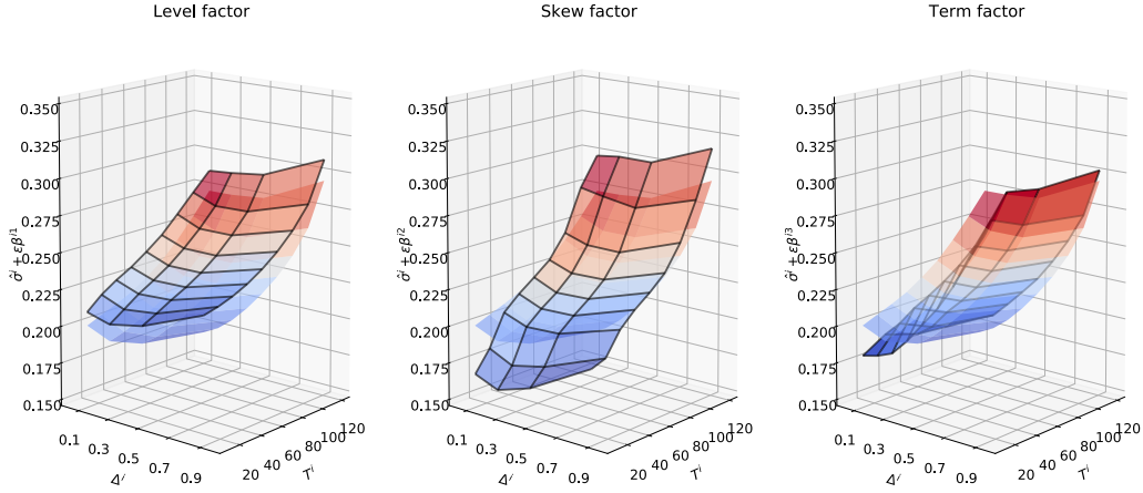
Figure .1: Effect of the different volatility factors on the implied volatility surface. Starting from a historical implied volatility surface ( \hat{\sigma}^i ), we show the modified implied volatility surface ( \hat{\sigma}^i + \varepsilon\beta^i q ) after adding a contribution of size \varepsilon from the volatility factor q . The original (non-modified) implied volatility surface is shown in light opacity for reference.
