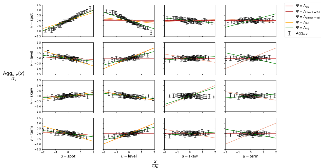
Figure II.5: Normalized cross aggregate impact curves.
