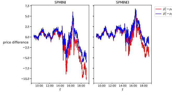
Figure III.5: Example of predicted prices from K^1 and K^2 .
