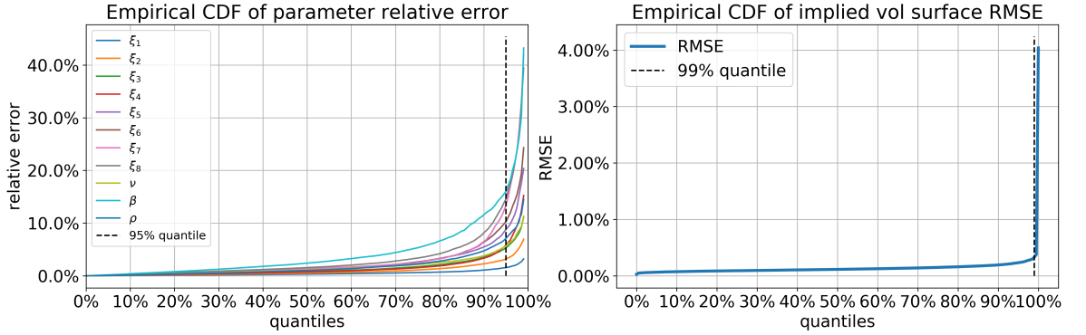
Figure VIA.10: Synthetic parameter and implied volatility surface error of the neural network based calibration for the 1 Factor Bergomi model.
