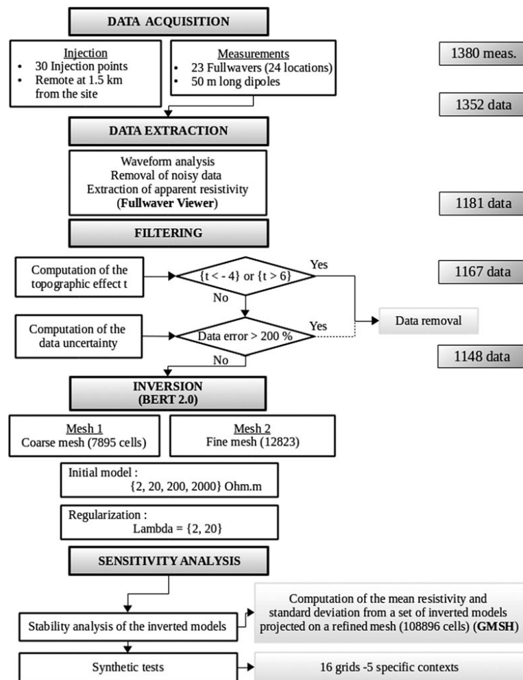
Figure 6. Methodological flowchart.
