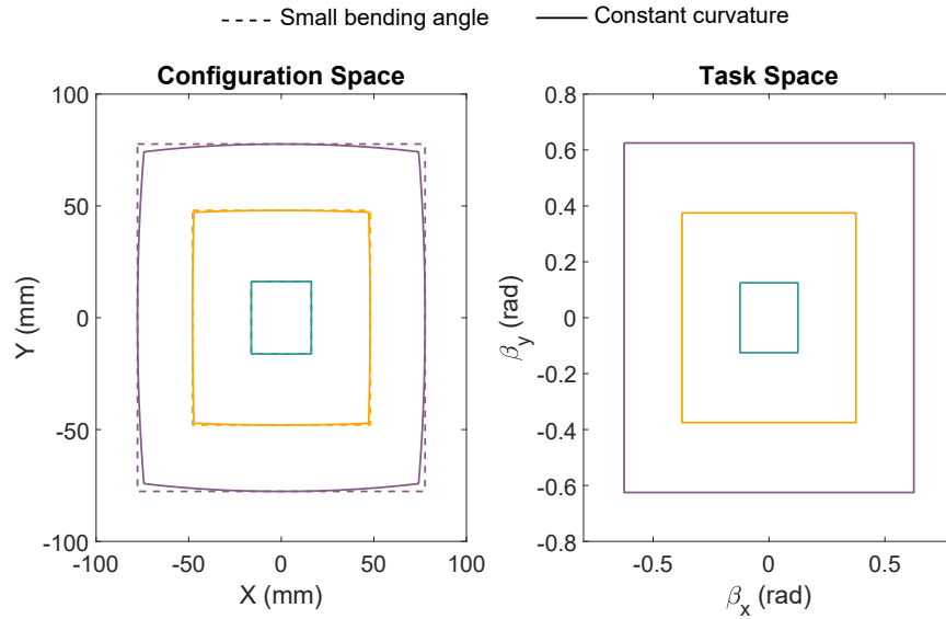
Figure 4.4: Comparison between the configuration space and cartesian space.
