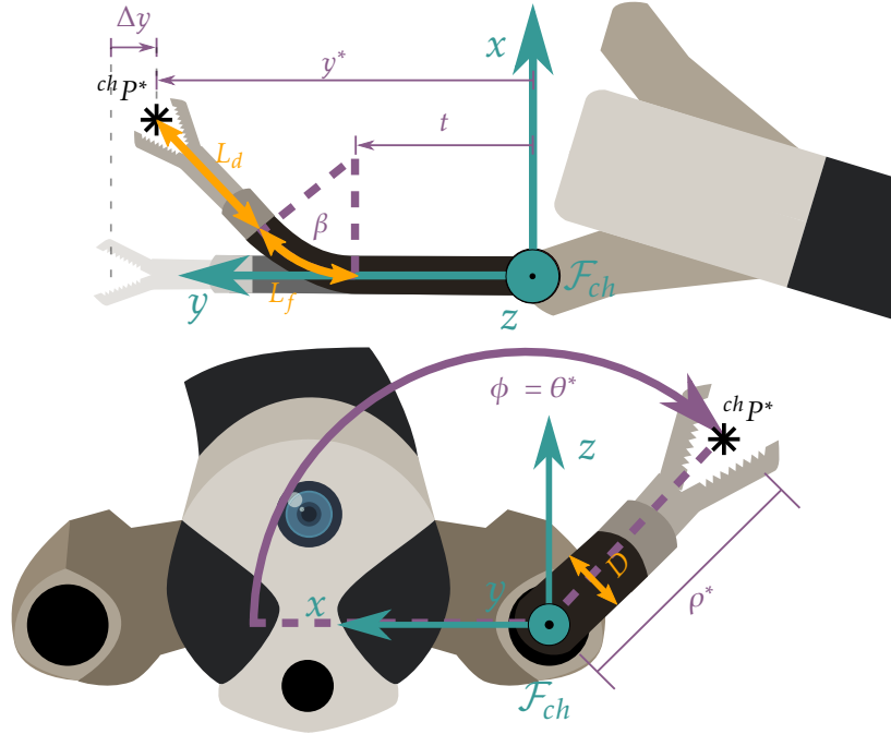
Figure 3.2: The considered cable-driven instrument passing through the left channel of the STRAS system. Top: top view, bottom: face view. Figure shows left channel frame, the degrees-of-freedom of the instrument, configuration variables and important construction parameters [Porto et al., 2019d].
