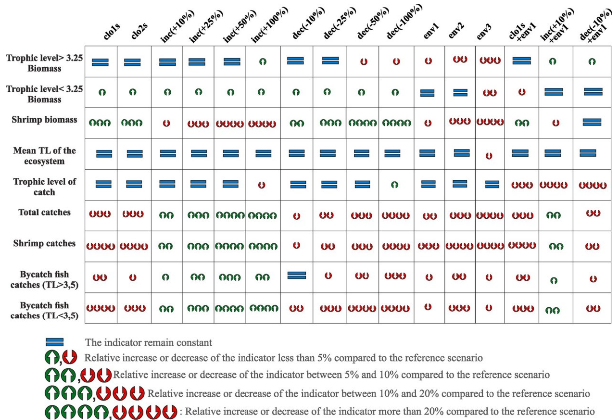
Fig. 9. Summary of the projected responses in fishing management scenarios and environmentally driven provisions in terms of conservation and exploitation indicators. For more detail about each scenario, see Table 1.
