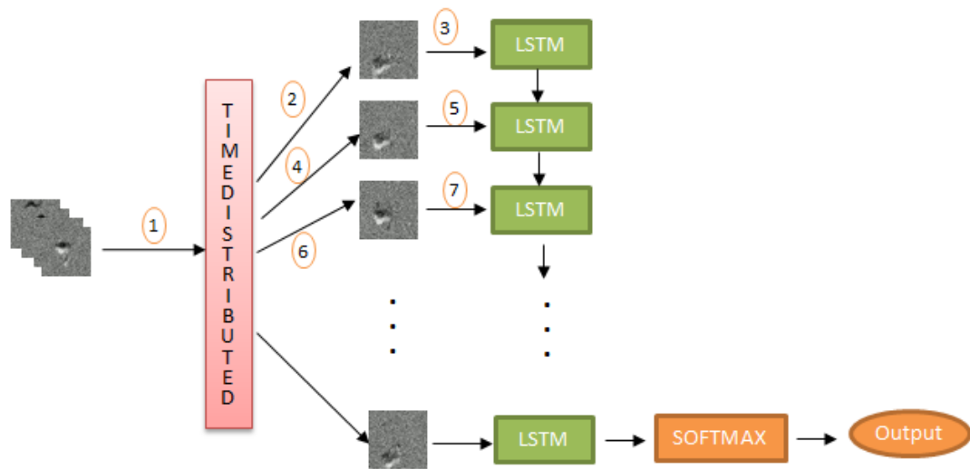
FIGURE 4.14 – Architecture LSTM
