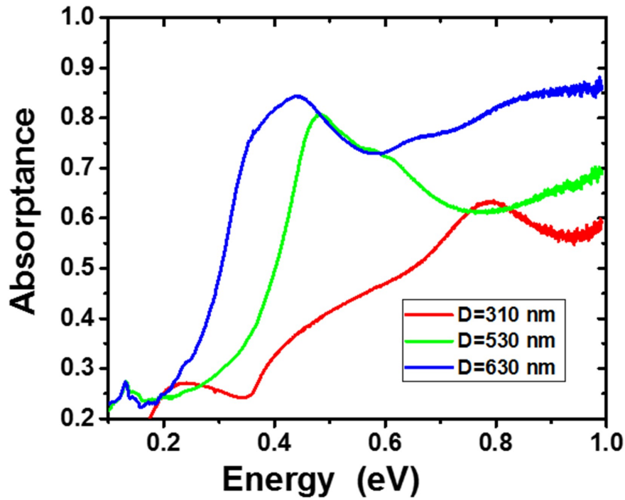
Figure II.16: Room temperature FTIR spectra of InAs NWs with different diameters ( D ) at constant pitch ( 4\ \mu\text{m} ).
