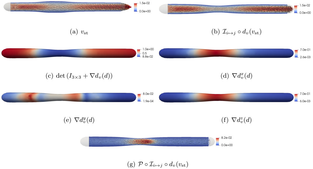
Figure 4.9: Full pipeline of field transport v_{st} from \Omega_i to \Omega_j .
