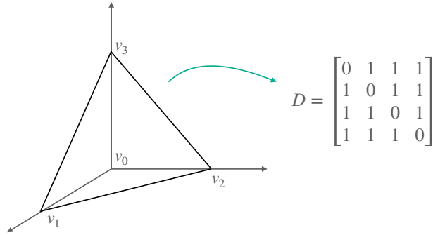
Figure 5.13: Input data set for toy MDS example.
