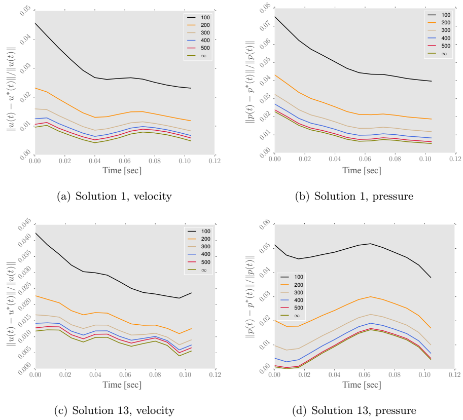
Figure 3.18: Relative errors in joint reconstruction for two time dependent solutions. Figure 3.17(b) suggests us to use 30 modes in the reconstruction.
