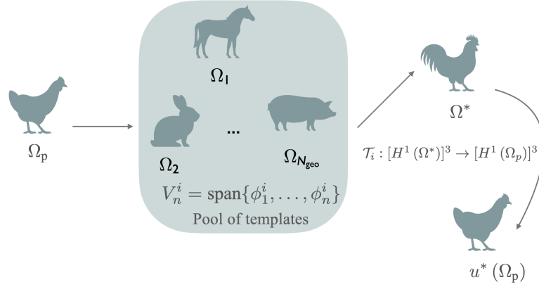
Figure 4.2: Multi-domain problem pipeline scheme.
