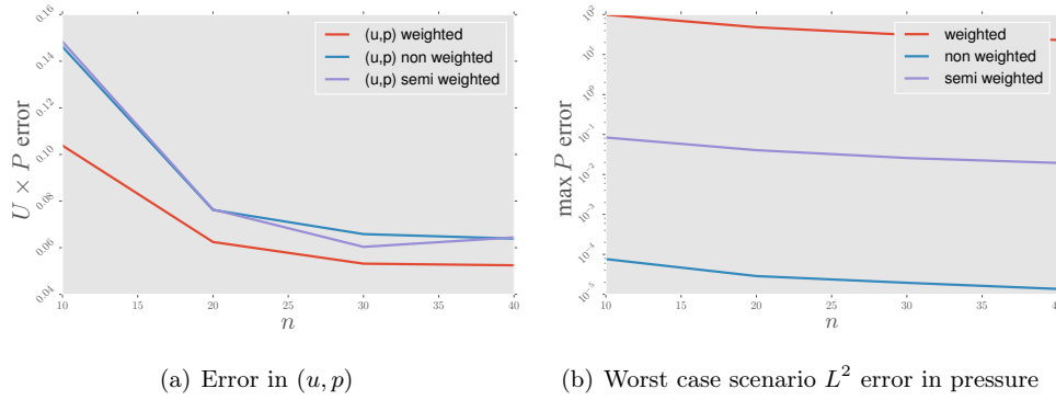
Figure 3.5: Impact of the weighting parameter in the inner product that defines the search space. In the legend, non weighted stands for \alpha = 1 , weighted stands for \alpha as expressed in (3.32) and semi-weighted stands for \alpha as the square root of (3.32)
