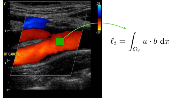
Figure 2.5: Schematic way of looking at the CFI measures as a set of elements in V^* .
