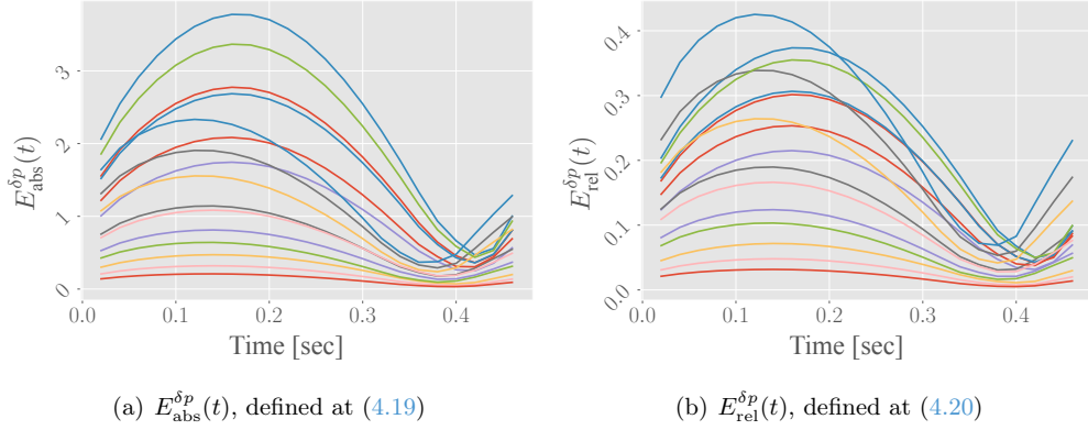
Figure 4.25: Average errors in pressure drop per target geometry.
