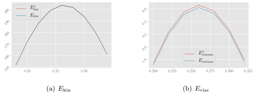
Figure 4.23: Reconstruction of quadratic forms E_{\text{kin}} and E_{\text{visc}} in a time window close to the velocity peak.
