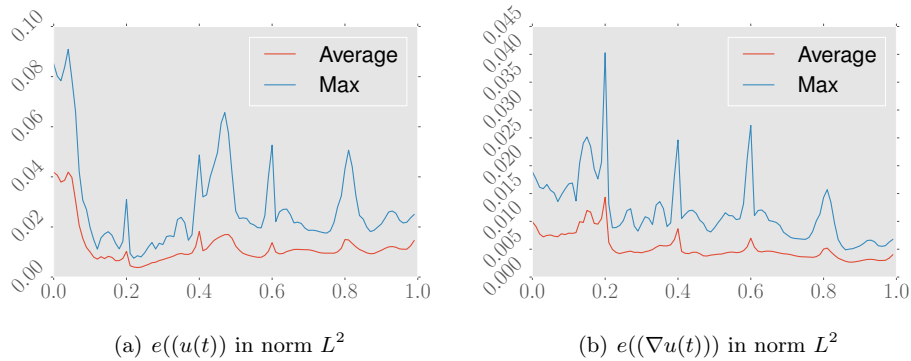
Figure 3.8: L^2 error in velocity reconstruction. We observe that the accuracy for both u^* and \nabla u^* stays in the same orders of magnitude. The vertical axis shows the error as expressed in (3.33). The horizontal axis shows the normalized time for one cardiac cycle.
