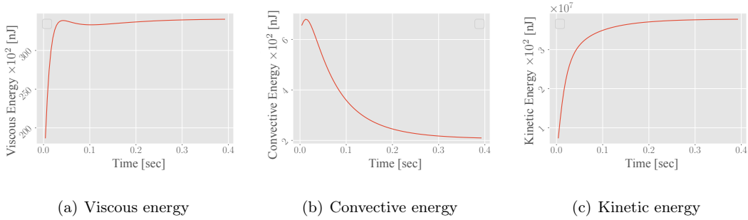
Figure 5.11: Time evolution of quadratic forms (5.13) of the velocity field.
