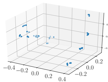
Figure 4.15: 3D representation of the full pool of geometries. In spite that the plot does not provide the same facility to interpret the data as it does for the two dimensional case, MDS indeed captures the intrinsic dimension of the parameter space in the sense that D_H \sim \hat{D} .
