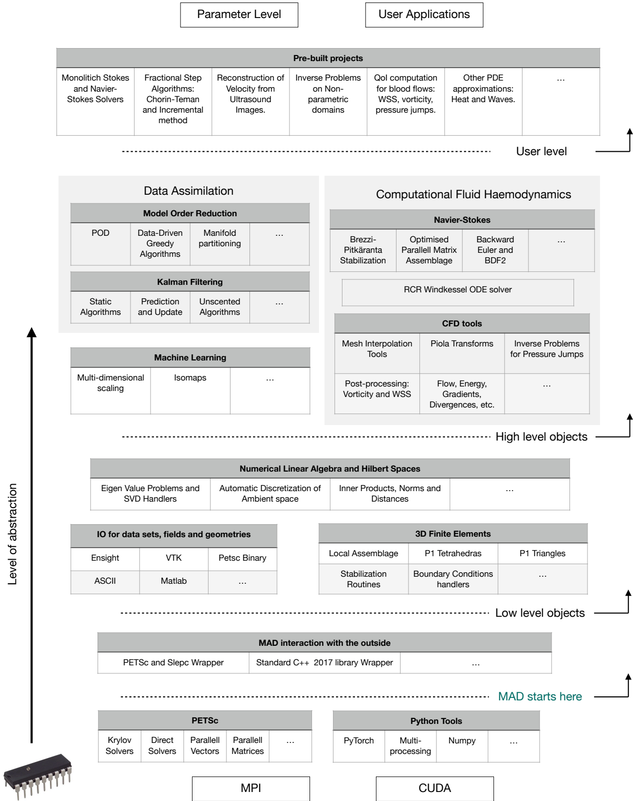
Figure 5.1: Map of MAD features.
