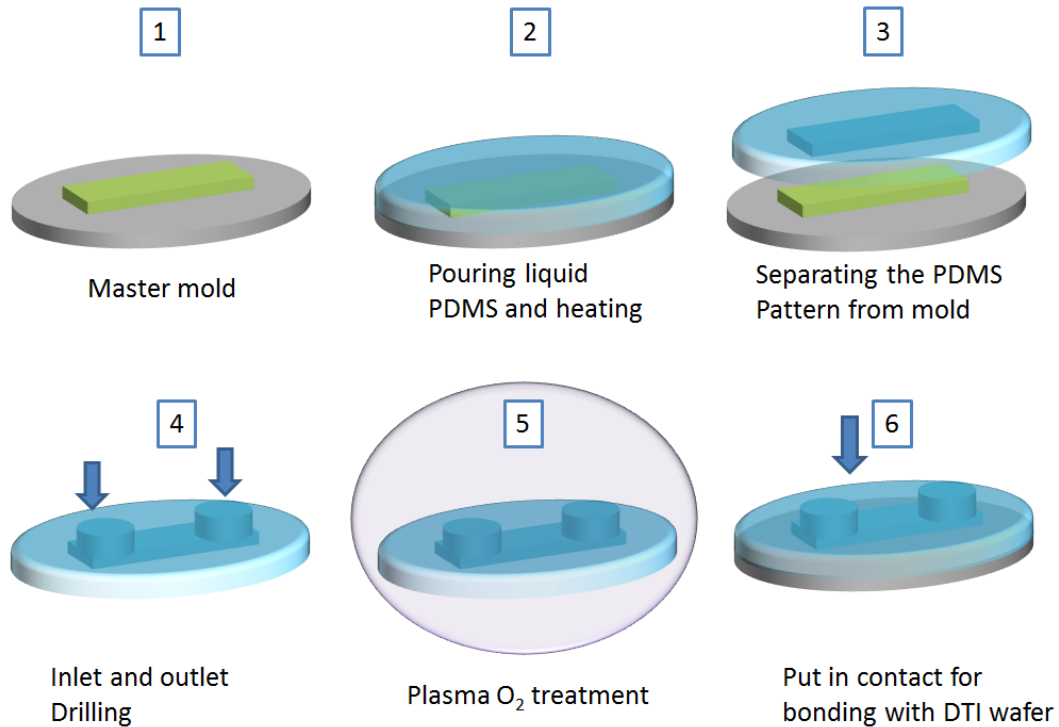
Figure III.26 Schematic of the different steps involved in making a PDMS micro-channel
