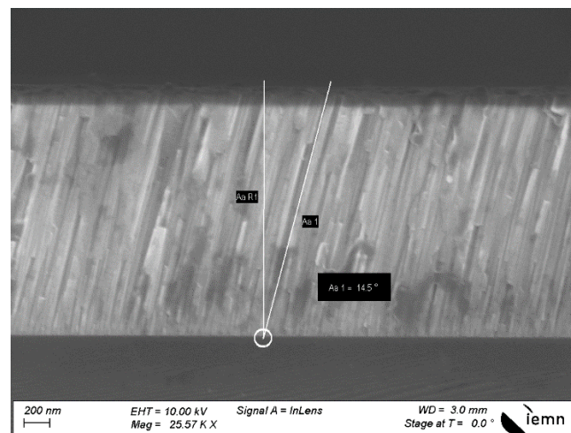
Figure III.11 Cross-section SEM image of the ZnO film with 14.5^\circ inclined c-axis [123]
