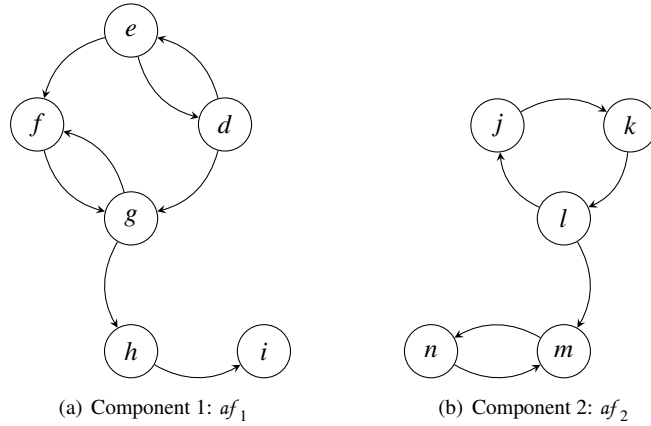
Figure 4.5: The connected components of \mathcal{AF}_{hard}
