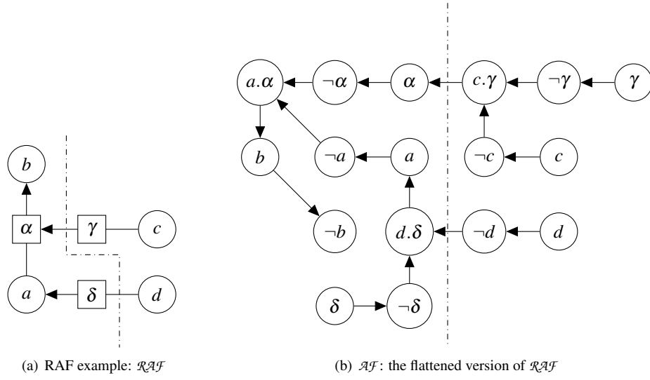
Figure 14.26: Decomposability illustration
