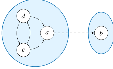
Figure 4.12: Same merge configuration for different labellings
