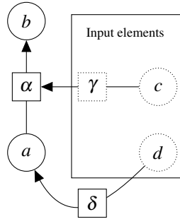
Figure 14.27: \widetilde{\mathcal{R}\mathcal{A}\mathcal{F}}_1
