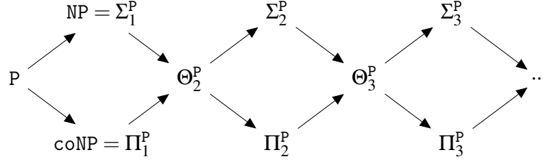
Figure 16.4: Polynomial hierarchy
