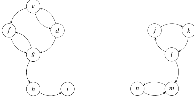
Figure 4.4: \mathcal{AF}_{hard}
