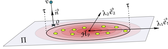
Figure 3.8: The likelihood that \varrho belongs into \Pi is estimated from \mathcal{N}_{\text{PDF}}(\varrho \mid \mathcal{H}_\mu^k, \Sigma) shown in red. The likelihood must be higher than \tau in order to consider \Pi as a valid plane for \varrho ( k indices dropped for clarity).
