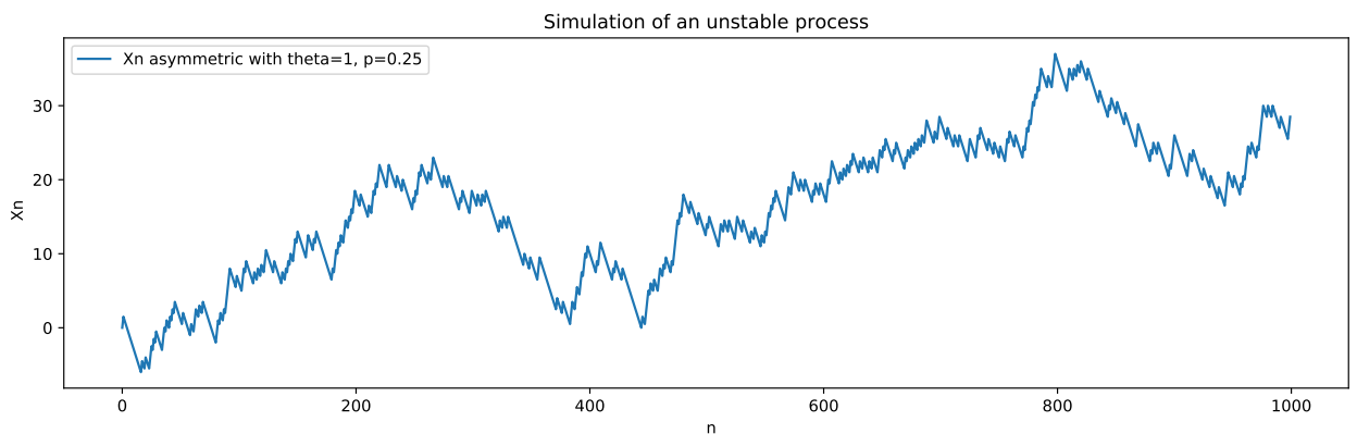
Figure 2.2 – Simulation of (X_n) ( p = 0.25, \theta = 1 )
