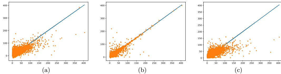
Figure 4.10: Voroni cell moment of inertia reconstruction; example and Q-Q points using (a) estimated scattering moments, (b) exact scattering moments, (c) benchmark.
