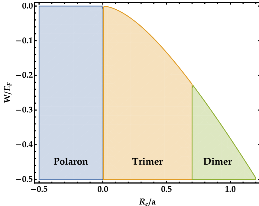
Figure 5.6: Phase diagram for an impurity immersed in a spin 1/2 Fermi sea. We distinguish three regimes depending on the ratio between the resonance range R_e and the interaction strength a . When the impurity is interacting weakly with the spin components ( a \rightarrow 0^- ), a Fermi polaron state is the ground-state of the system, this state is composed of the impurity dressed by the particle-hole excitations it creates in the Fermi sea. For increased interactions ( a \rightarrow 0^- ), around R_e/a = 0.0036 , the impurity binds to an existing Cooper pair and the polaronic branch connects to the resonant Cooper-like trimer states. In the strongly attractive regime R_e/a \approx 0.7 the Cooper pairing is overcome by the attraction between the impurity and the fermions and a dimer is formed.
