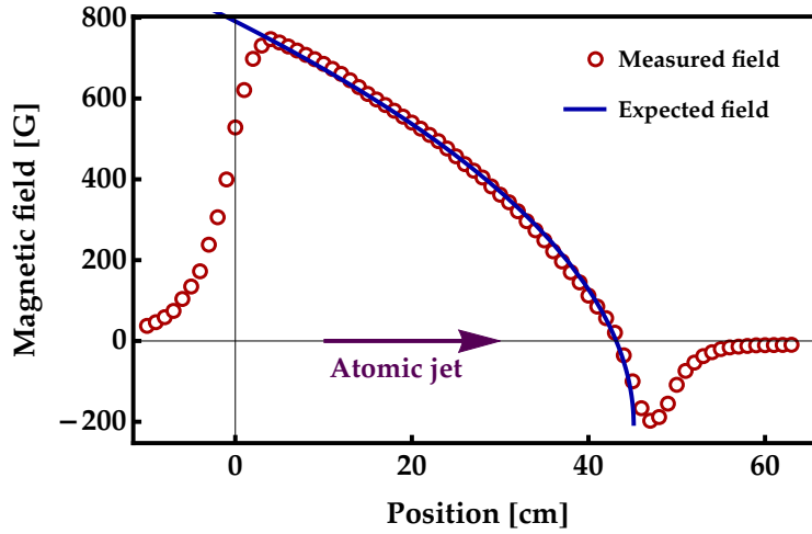
Figure 2.6: Magnetic field of the Zeeman slower. Measured magnetic field values at multiple positions of the Zeeman slower with a current I = 20A (red dots), and expected variation of the magnetic field calculated for the same current value (blue line). Here the position at 0 corresponds to the beginning of the Zeeman slower for atoms coming from the oven. The measured and expected values are in satisfactory agreement. Figure adapted from M. Delehaye’s thesis [237] and S. Jin’s thesis [227].
