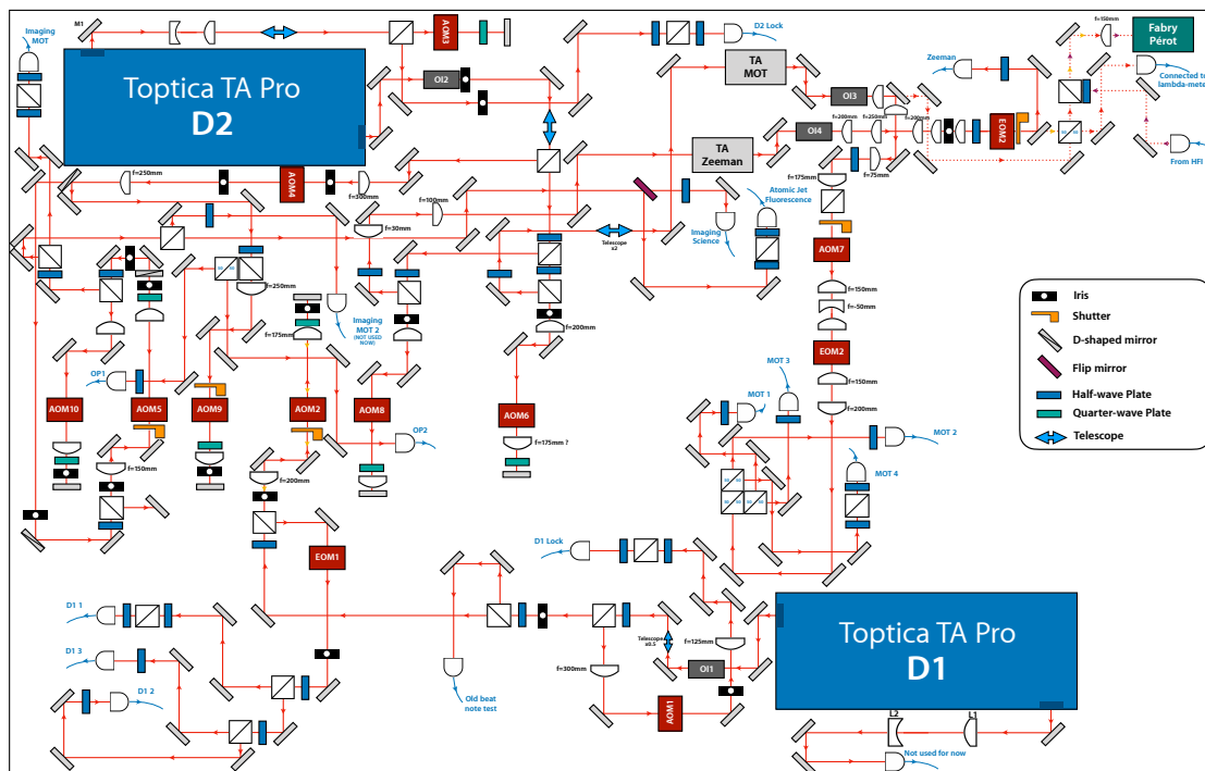
Figure 2.4: {}^6\text{Li} optical table. Detailed reconstruction of the {}^6\text{Li} optical table. The spectroscopy part is left out. We use two master lasers one for the cooling steps which use the D_2 transition (Zeeman, MOT, D_2 molasses), and the other is used solely for the D_1 gray molasses. To make up for the low power output of the Toptica lasers, we use two TA chips placed in the paths of the MOT and Zeeman beams.
