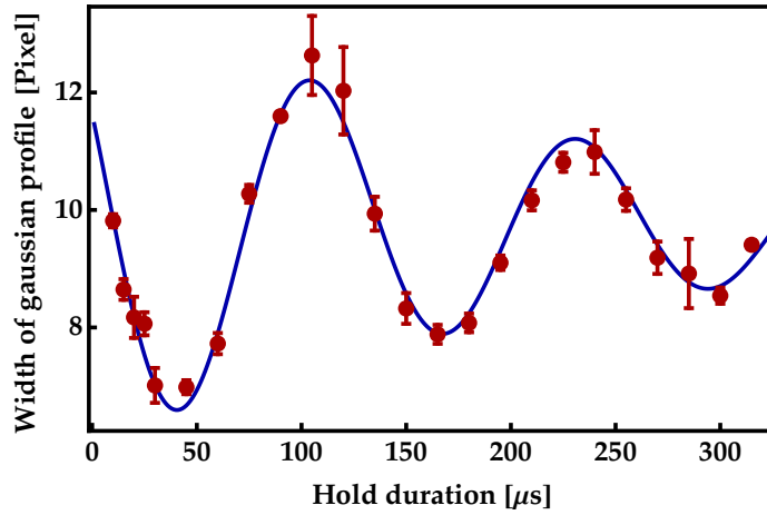
Figure 2.11: Radial frequency measurement. The breathing mode is triggered by deconfining the gas, leaving it to expand for a certain time (between 30 to 50 \mu\text{s} here) and then we hold the atoms inside the trap and measure the radial size of the cloud for different hold time durations. Figure adapted from S. Jin's thesis [227].
