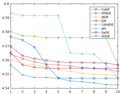
(a) 1CB3
