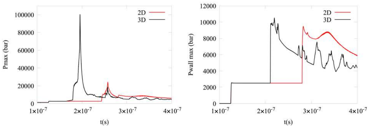
Figure 8.2: Time evolution of the maximum pressure inside the fluid (left) and near the wall (right). WENO3-Z, 2D, uniform mesh: 1500 \times 2500 ; 3D, stretched mesh: 1050 \times 850 \times 850 . P_{sh} = 1200 \text{ bar}
