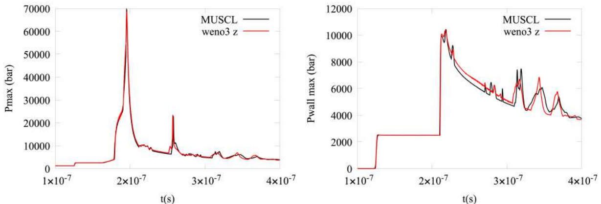
Figure 8.4: Time evolution of the maximum pressure inside the fluid (left) and near a wall (right). Comparison between MUSCL and WENO3-Z. P_{sh} = 1200 bar
