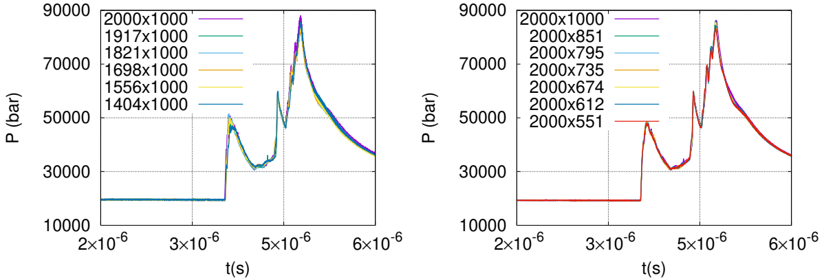
Figure 7.14: Water-air shock-bubble collapse, P_{max} (bar) solution, mesh stretching effect, sinh from a point in x -direction (left), tanh from bottom to top in y -direction (right)
