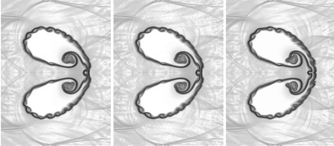
Figure 7.8: Air-helium shock-bubble interaction, HLLC Hancock WENO5-IS scheme, gradient of the density, comparison of mesh stretching strategies in X direction: uniform mesh (left), \tanh from the uniform mesh block (middle), \sinh from interior point (right)
