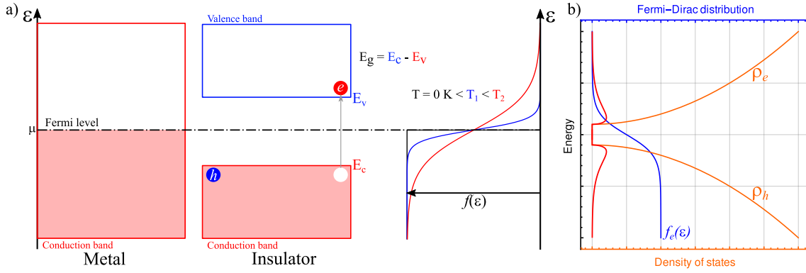
a) Fermi-Dirac distribution of metal for the different temperatures. Here, the chemical potential \mu is equaled to E_F , which is usually true for T = 0 K. For an insulator, \mu is chosen to lie equidistantly from the bottom of the valence and top of the conduction band. For an intrinsic semiconductor, if \epsilon = \mu , f(\epsilon) = \frac{1}{2} [7]. At k_B T_2 > E_g , the electron is promoted from the valence to conduction band, creating an electron-hole pair, resulting in conducting behavior. b) Electron and hole density of states (orange), Fermi-Dirac distribution f_e(\epsilon) for the electrons (blue). Hole distribution f_h(\epsilon) is inverse to the one of electrons. The product of the electron-hole density of states and Fermi-Dirac distribution for an insulator, in the parabolic band approximation, is shown in red. Adapted from Wikipedia.
