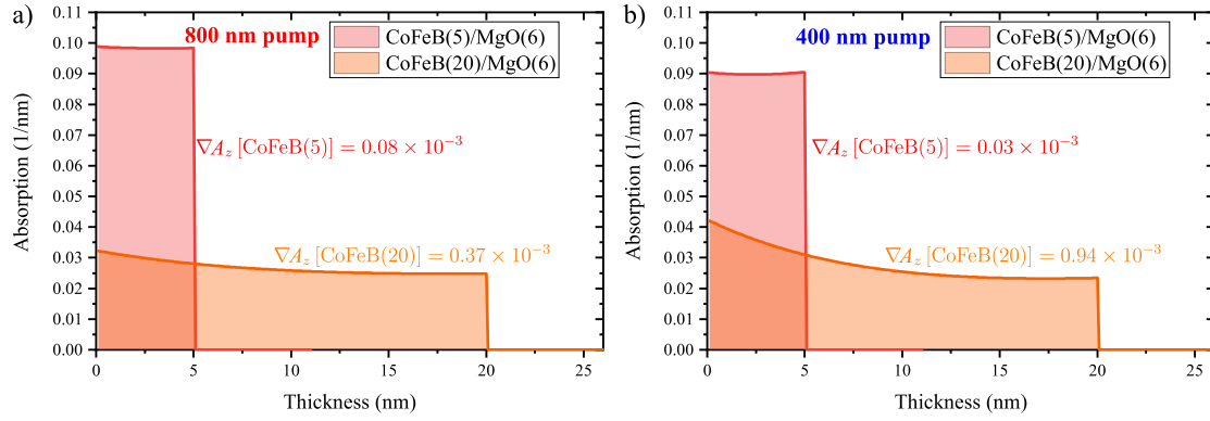
Figure 4.18 – Light absorption profiles: in the \text{CoFeB}(5)/\text{MgO}(6) and \text{CoFeB}(20)/\text{MgO}(6) bilayers, in Front Face configuration on the Glass substrate, for 800 and 400 nm pump wavelengths.
