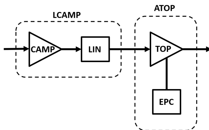
Figure 1.3 – HPA ATOP
