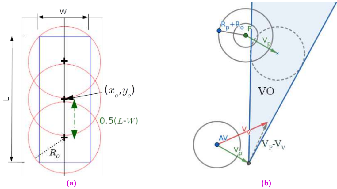
Fig. 6.2.: (a) Circular approximation of the AV footprint (Algorithm 2), (b) VO method applied to one part of the AV footprint
