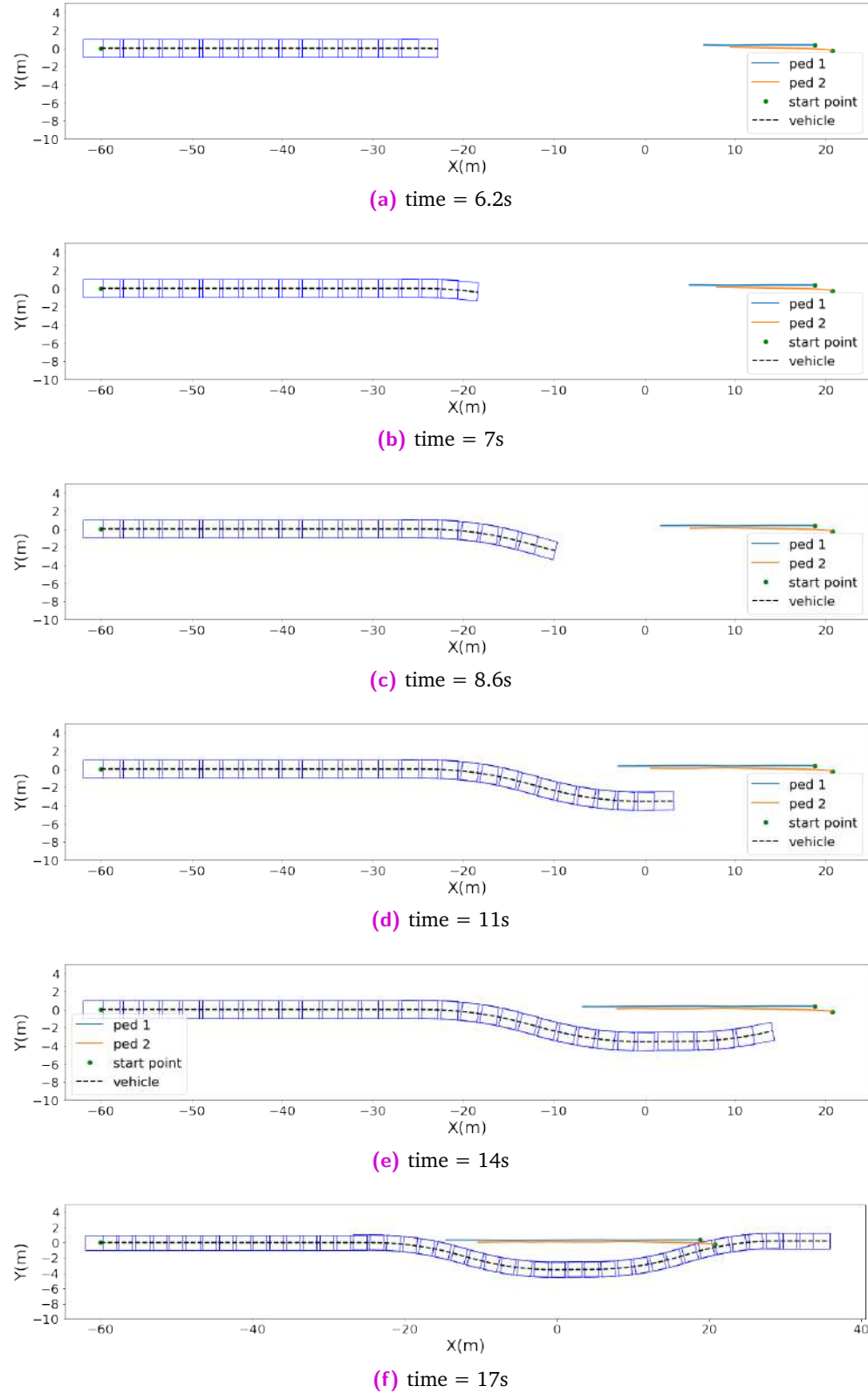
Fig. 5.17.: Resulting paths in the XY plane in a low-density frontal interaction scenario
