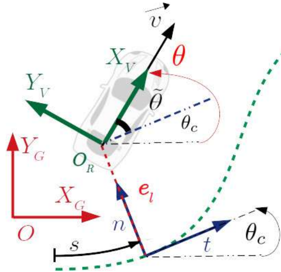
Fig. F.1.: Vehicle local frame and the Frenet frame
