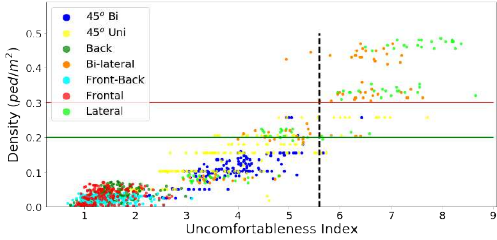
Fig. 7.11.: The pedestrian density Vs. average uncomfortableness index ( \bar{I}_{uf} ) across the test simulations
