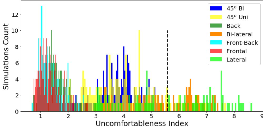
Fig. 7.10.: Histogram of the average uncomfortableness index ( \bar{I}_{uf} ) across the tests
