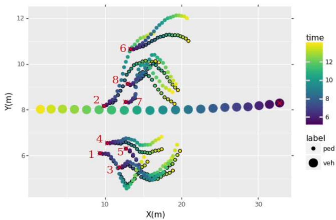
Fig. C.3.: Trajectory prediction model output in a frontal interaction scenario. Black contour: Real. No contour: Predicted. X: starting point
