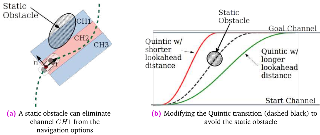
Fig. 8.4.: Targeting static obstacle in the PDC method
