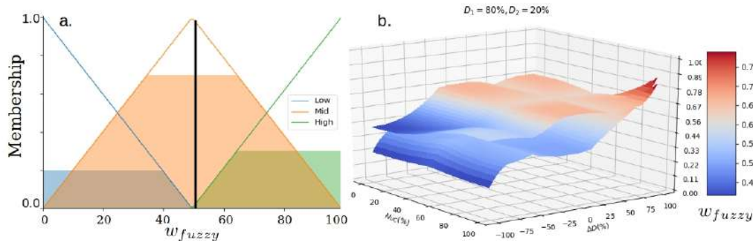
Fig. 5.7.: a: The membership functions of the channel fuzzy weight ( w_{fuzzy} ). b: The fuzzy model output with two different density levels
