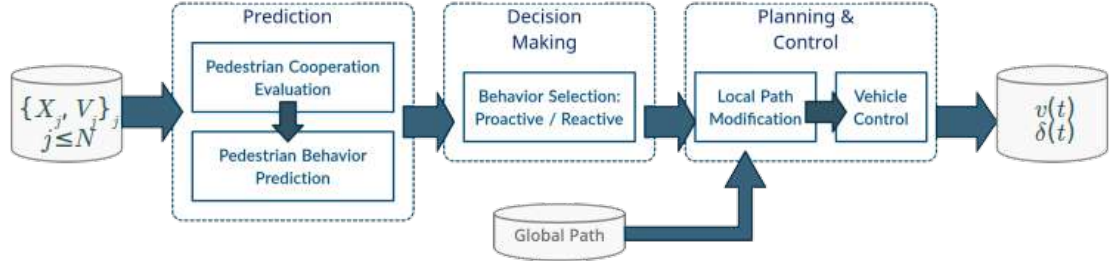
Fig. 1.7.: Suggested proactive navigation system components and information flow
