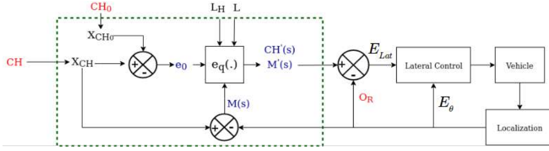
Fig. 5.12.: Lateral error computation using the Quintic path
