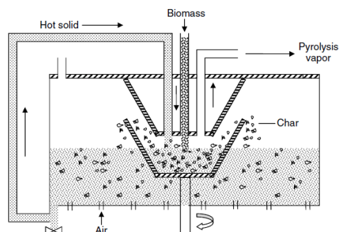
Figure 1.3-3 Rotating cone reactor
