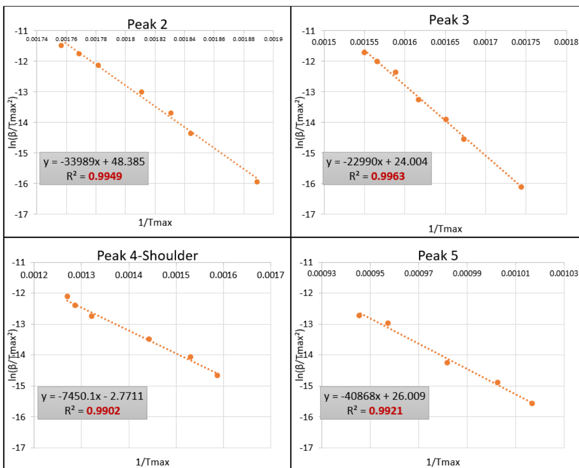
Figure 3.2-6. Sargassum linear regression graphics
