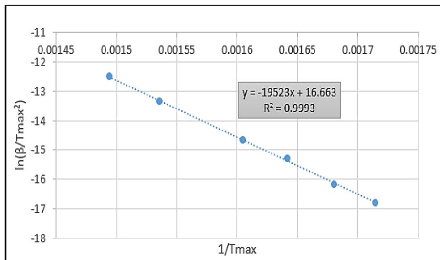
Figure 3.2-3. Kinetics parameters calculation using the Kissinger method
