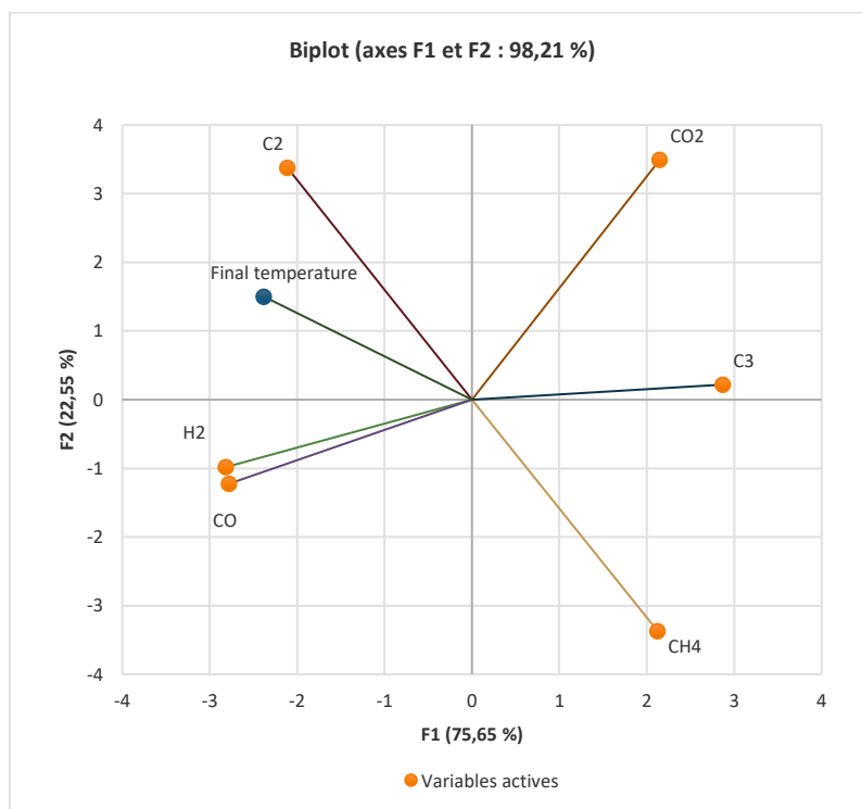
Figure 4.4-6 PCA Sargassum non -condensables chemical families
