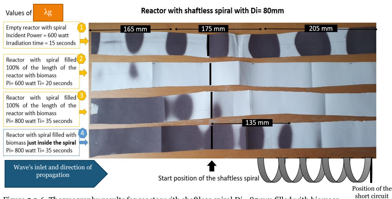
Figure 5.2-6. Thermography results for reactor with shaftless spiral Di= 80mm filled with biomass.
