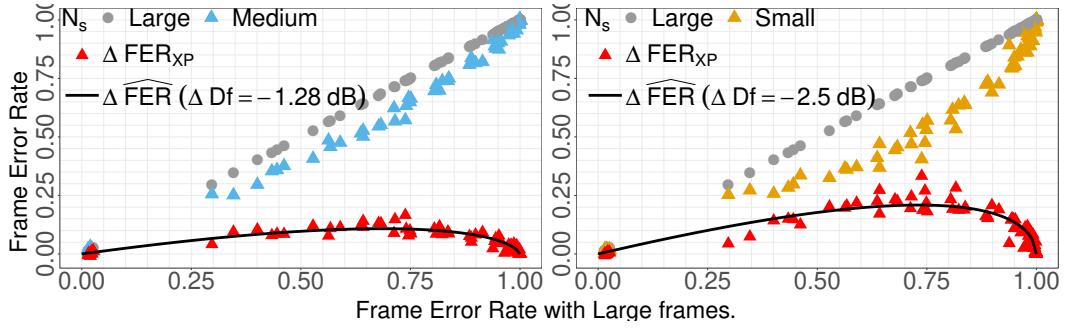
Figure 4.6: Comparison of the FER with N_s = 48 (Small) and N_s = 128 (Medium) against N_s \in [296..298] (Large). The black curve is the computed FER gain expected for sensitivity gain over a Rayleigh channel.
