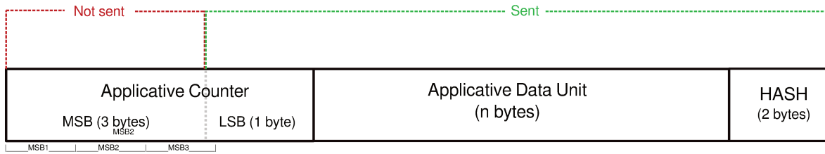
Figure 5.11: IDU structure.
