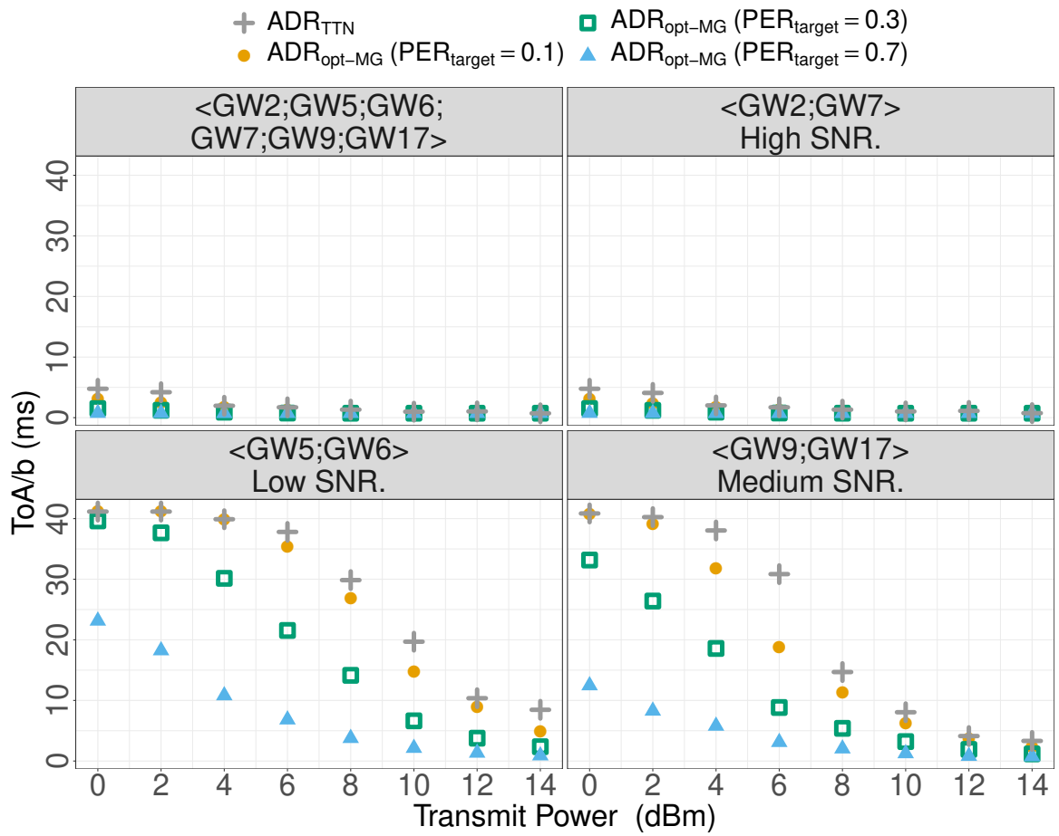
Figure 6.9: ToA/b as a function of P_{Tx} , for selected real world series of frames replays.
