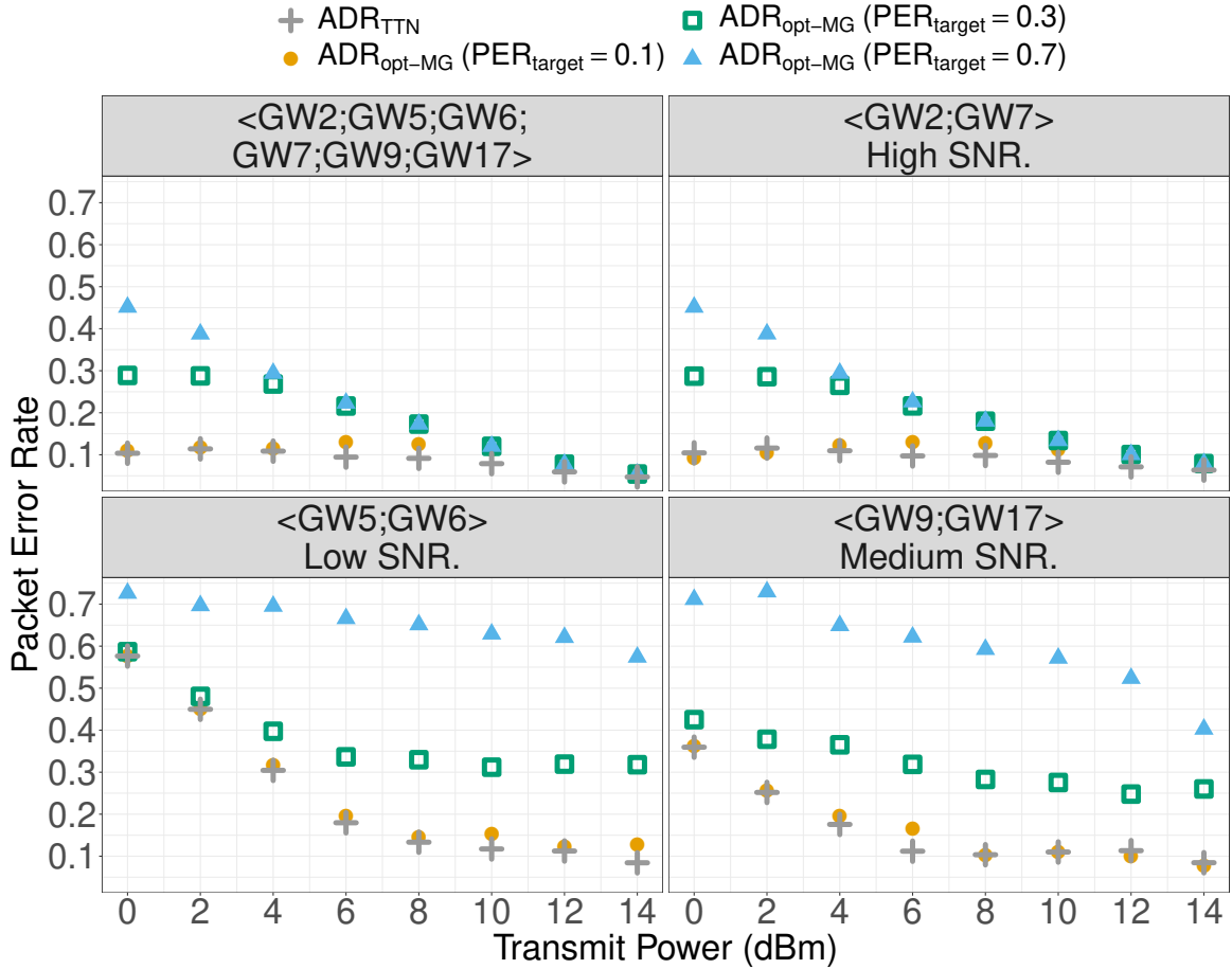
Figure 6.8: DER as a function of P_{\text{Tx}} , for selected real world series of frames replays.
