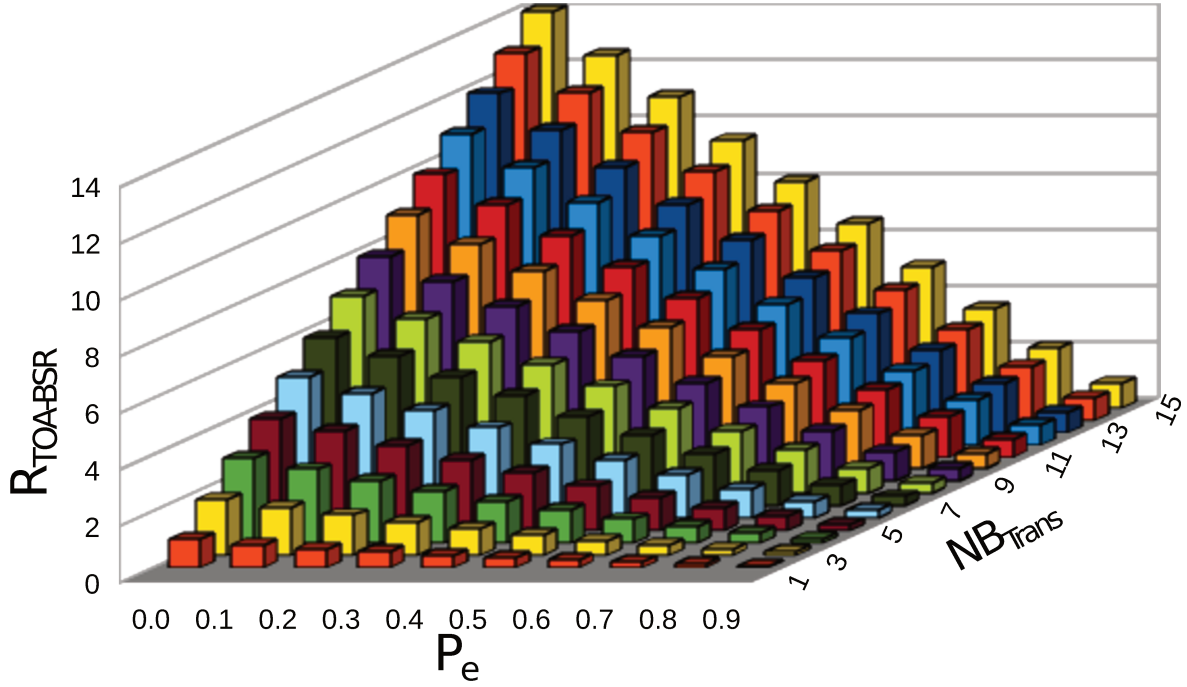
Figure 5.5: R_{TOA-BSR} as a function of P_e the failure probability and z = Nb_{Trans} .
