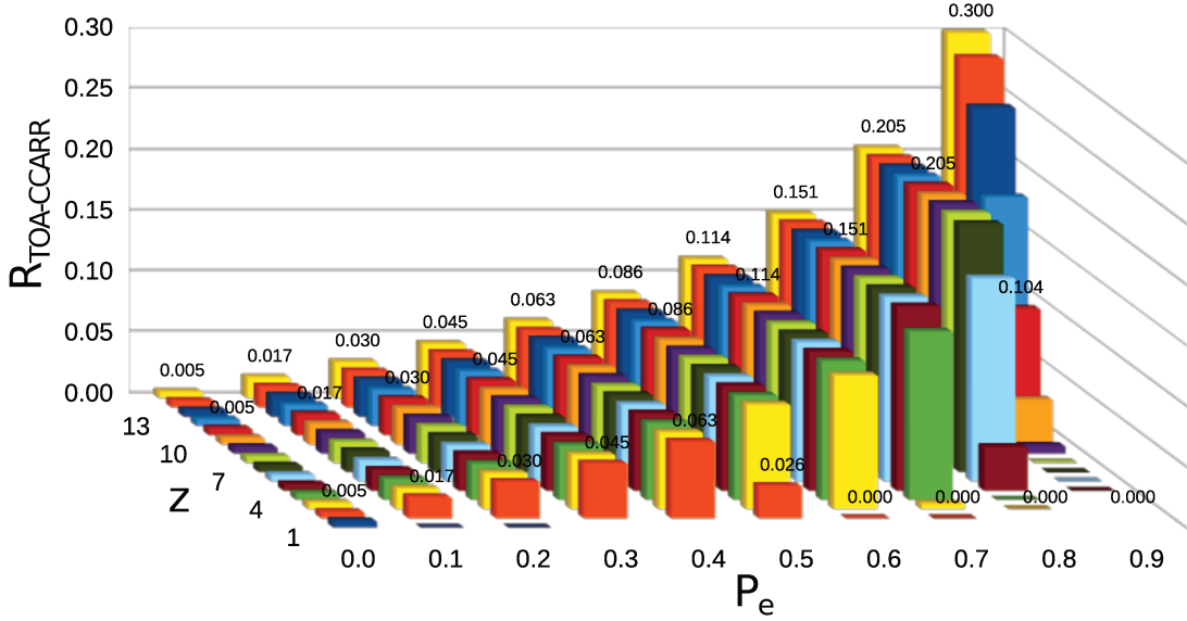
Figure 5.4: Probabilistic R_{TOA-CCARR} for CCARR (100,100×(z-1)), T=66.8\text{ms} and T'=46.3\text{ms} , as a function of z = \frac{1}{CR_{CCARR}} and P_e the error probability.
