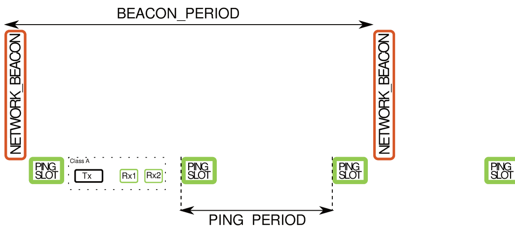
Figure 2.8: LoRaWAN class B network beaming and additional ED receive windows (PING SLOT).
