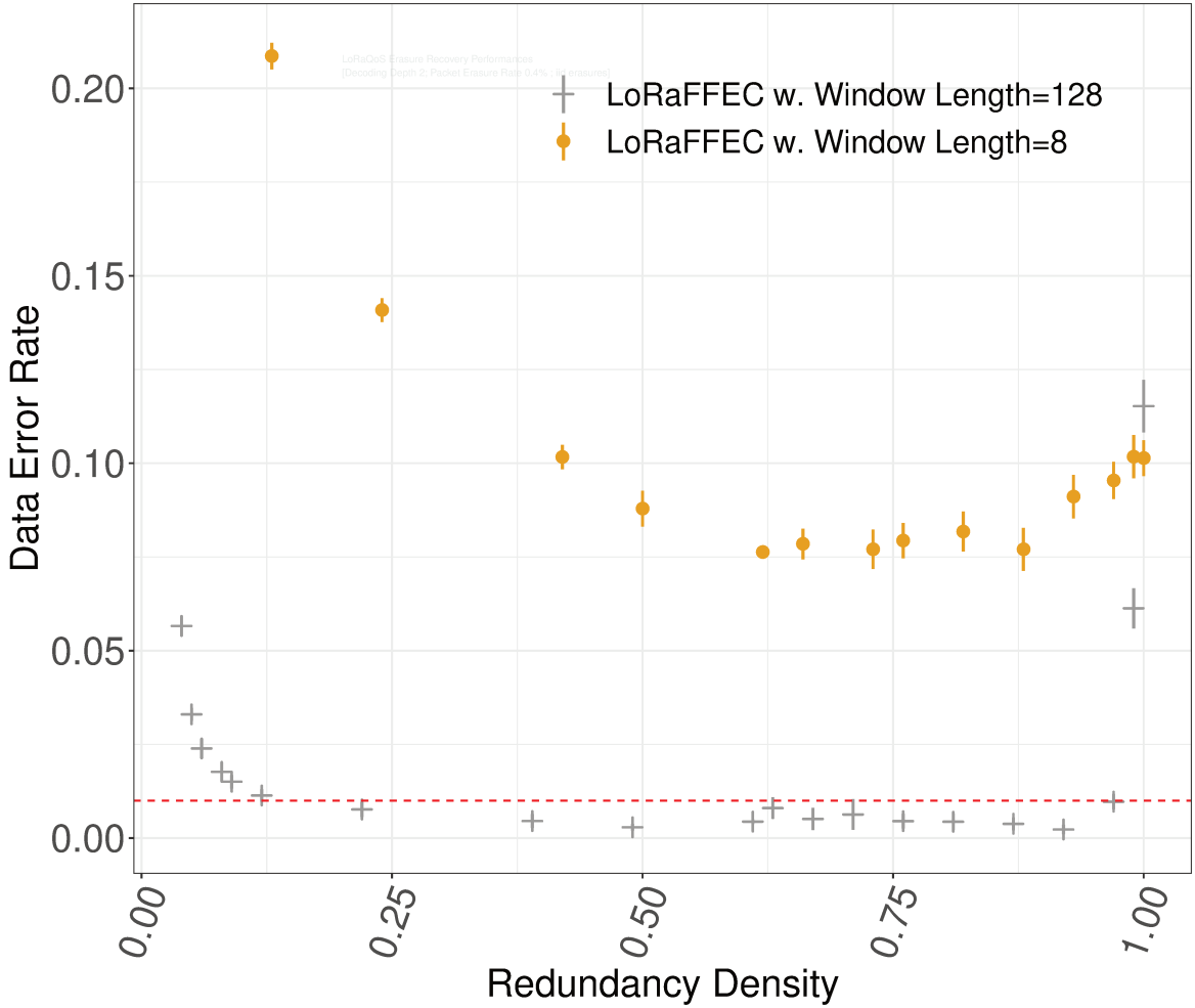
Figure 5.19: Simulated DER as a function of RD with LoRaFFEC (128; RD ; 2) and LoRaFFEC (8; RD ; 2) over a FER = 40 erasure channel. The red dashed line marks the DER = 0.01 threshold.
