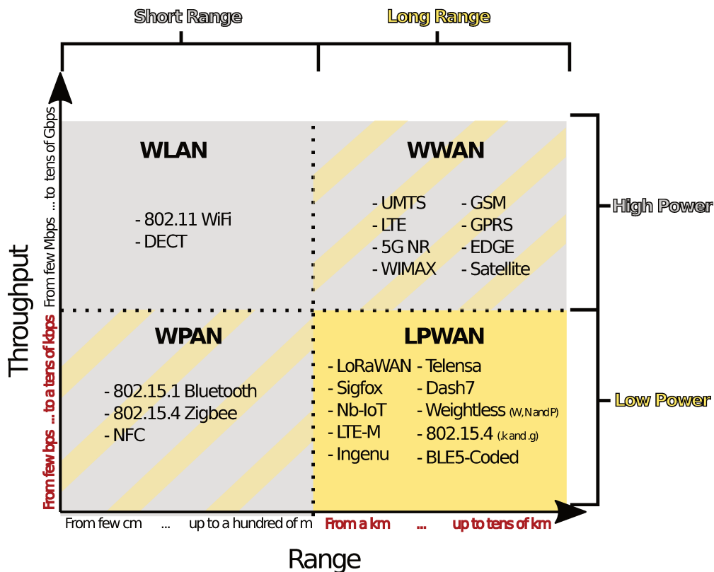
Figure 1.11: Wireless networks categorization by size and throughput. The long range and low power category is highlighted.
