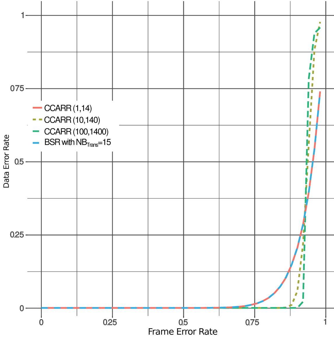
Figure 5.7: DER as a function of the FER for LoRaWAN BSR with Nb_{\text{Trans}} = 15 , CCARR (1,14), CCARR (10,140) and CCARR (100,1400).
