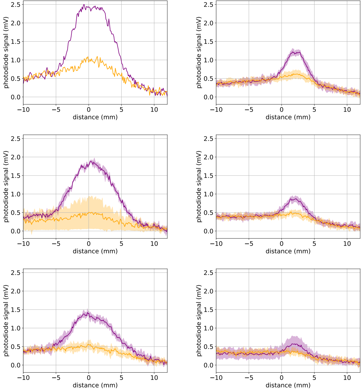
Figure 4.27 – Comparison of the diffracted atoms profiles for the two pulsing schemes. In purple are shown the profiles of the diffracted atoms after a \pi pulse labeled in the -nv_{\text{rec}} velocity class (from top to bottom, n = 1, 2 and 4 ), in yellow the same profiles are shown when no light is sent in the cavity. Distances along the x -axis correspond to vertical distances at the time of the pulse where the x = 0 corresponds to the apogee of the mean trajectory. This distance is reconstructed from the time of arrival knowing the launching velocity. The difference between the mean heights of the atoms for the two pulsing schemes is due to realignment of the cavity in between the two acquisition runs.
