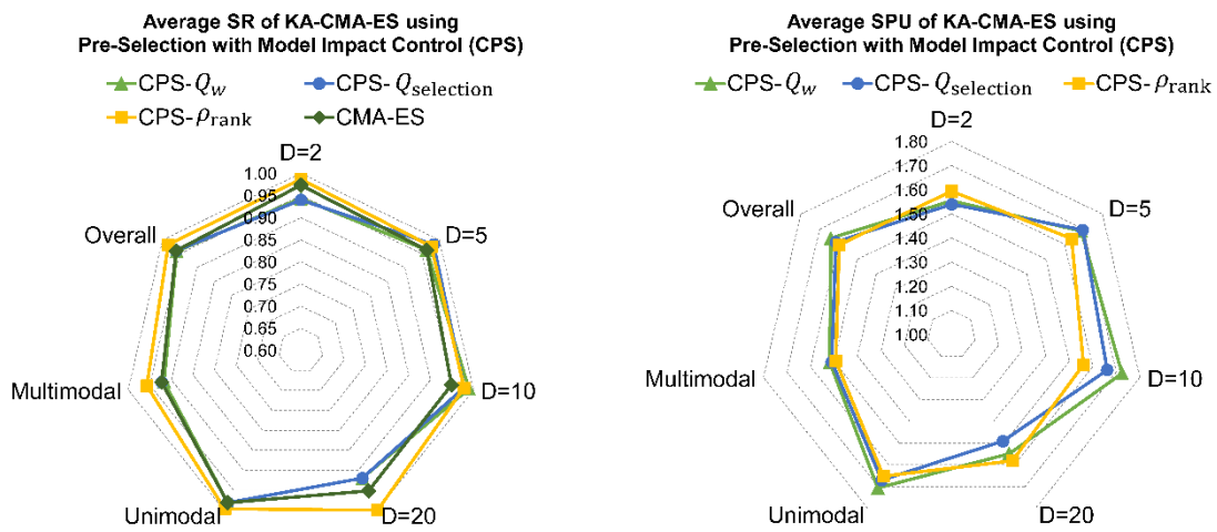
Figure 4.4 Average success rate and outperform rate of pre-selection with model impact control using different model quality measures.
