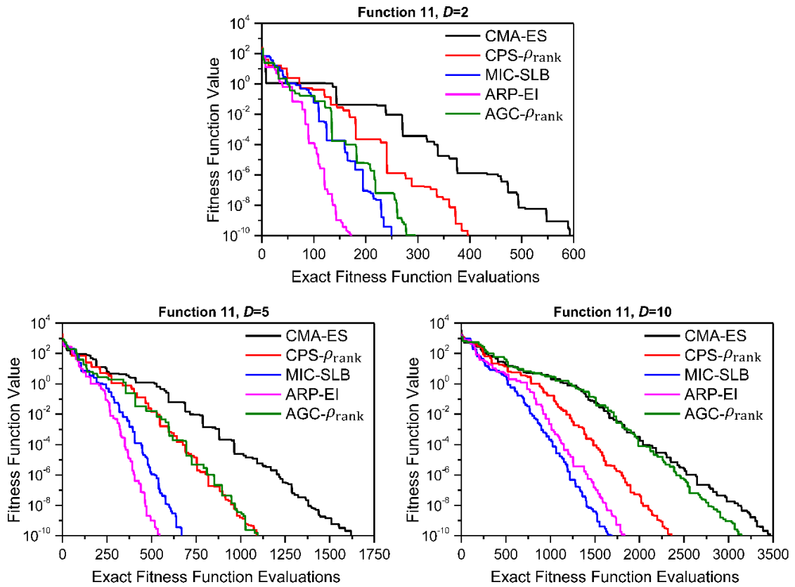
Figure 4.23 Convergence graphs of function 11
