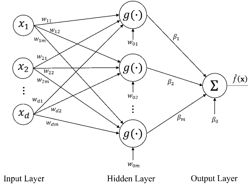
Figure 3.5 Structure of a three-layer MLP network
