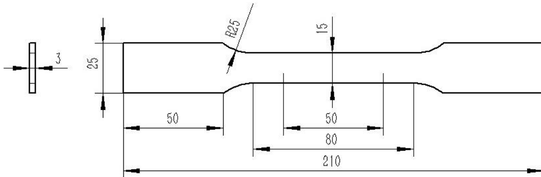
Figure 5.5 Geometry dimension of the test specimen
