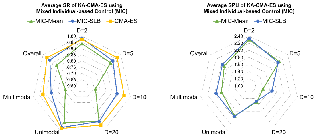
Figure 4.7 Average success rate (SR) and speedup performance (SPU) of KA-CMA-ES using mixed individual-based control (MIC).
