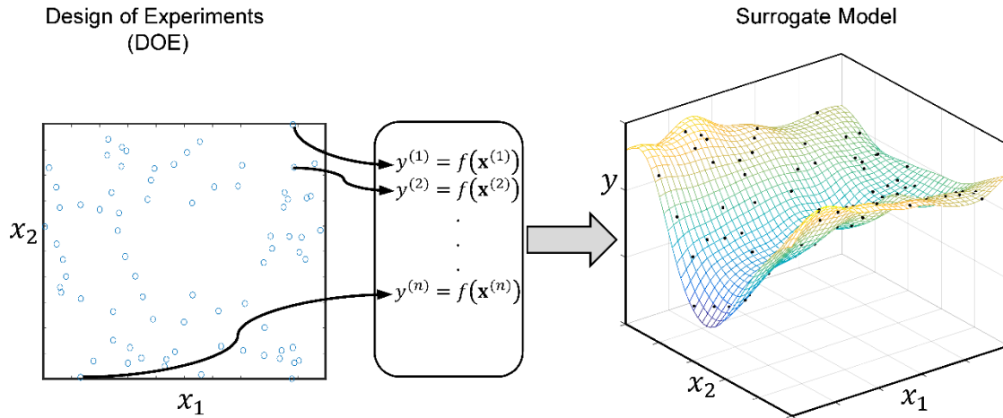
Figure 3.1 Process of surrogate modeling
