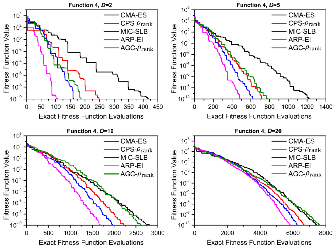
Figure 4.16 Convergence graphs of function 4
