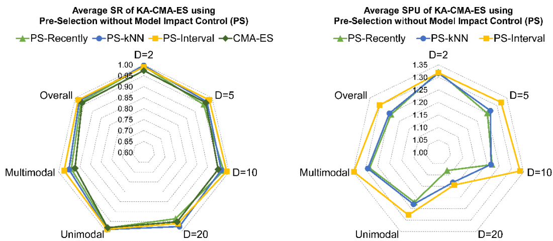
Figure 4.3 Radar charts of average success rate and speedup performance of KA-CMA-ES using pre-selection without model impact control (PS).
