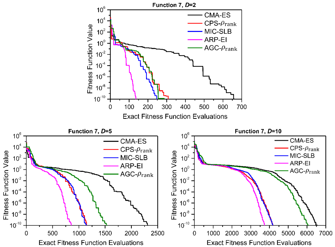
Figure 4.19 Convergence graphs of function 7
