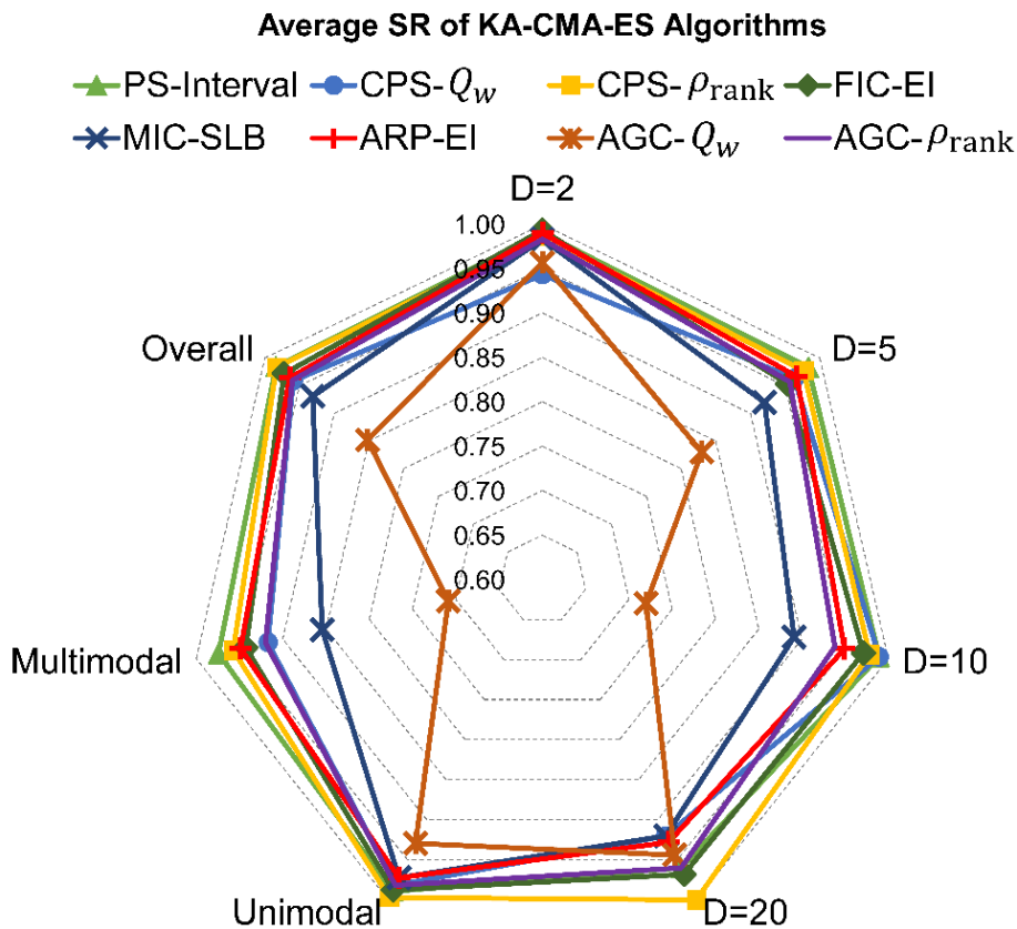
Figure 4.11 Comparison of average success rate (SR) of KA-CMA-ES algorithms.
