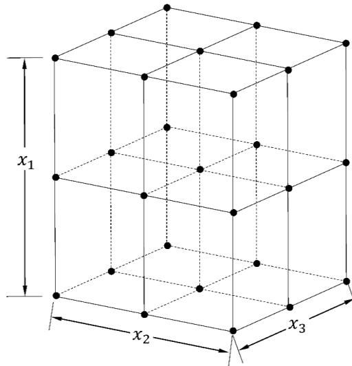
Figure 3.2 A 3-level and 3-dimensional full factorial design (27 points)
