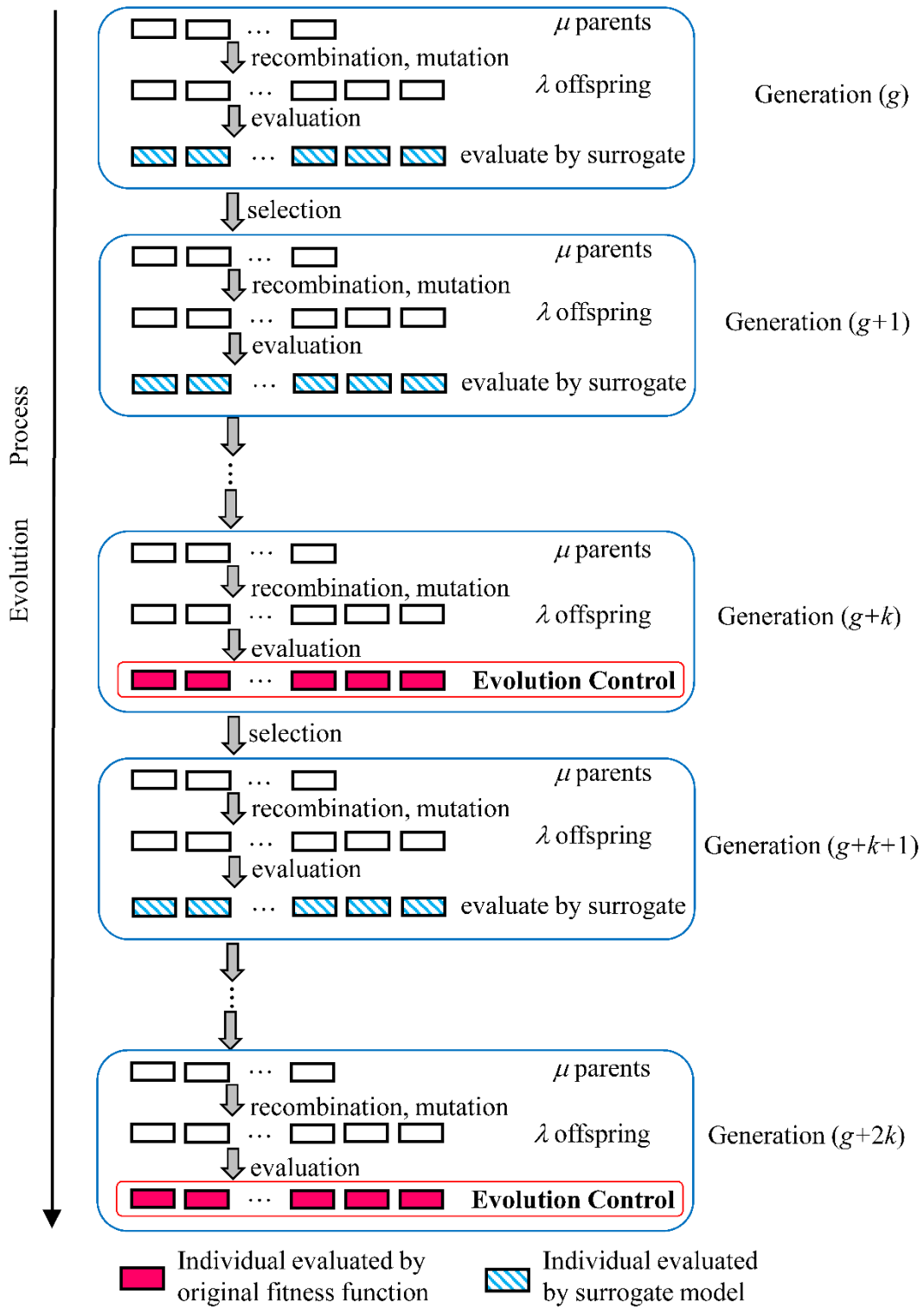
Figure 1.4 Illustration of fixed generation-based control
