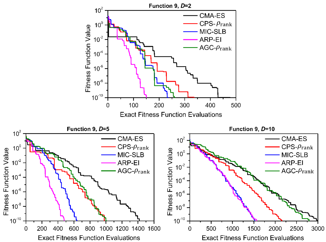
Figure 4.21 Convergence graphs of function 9
