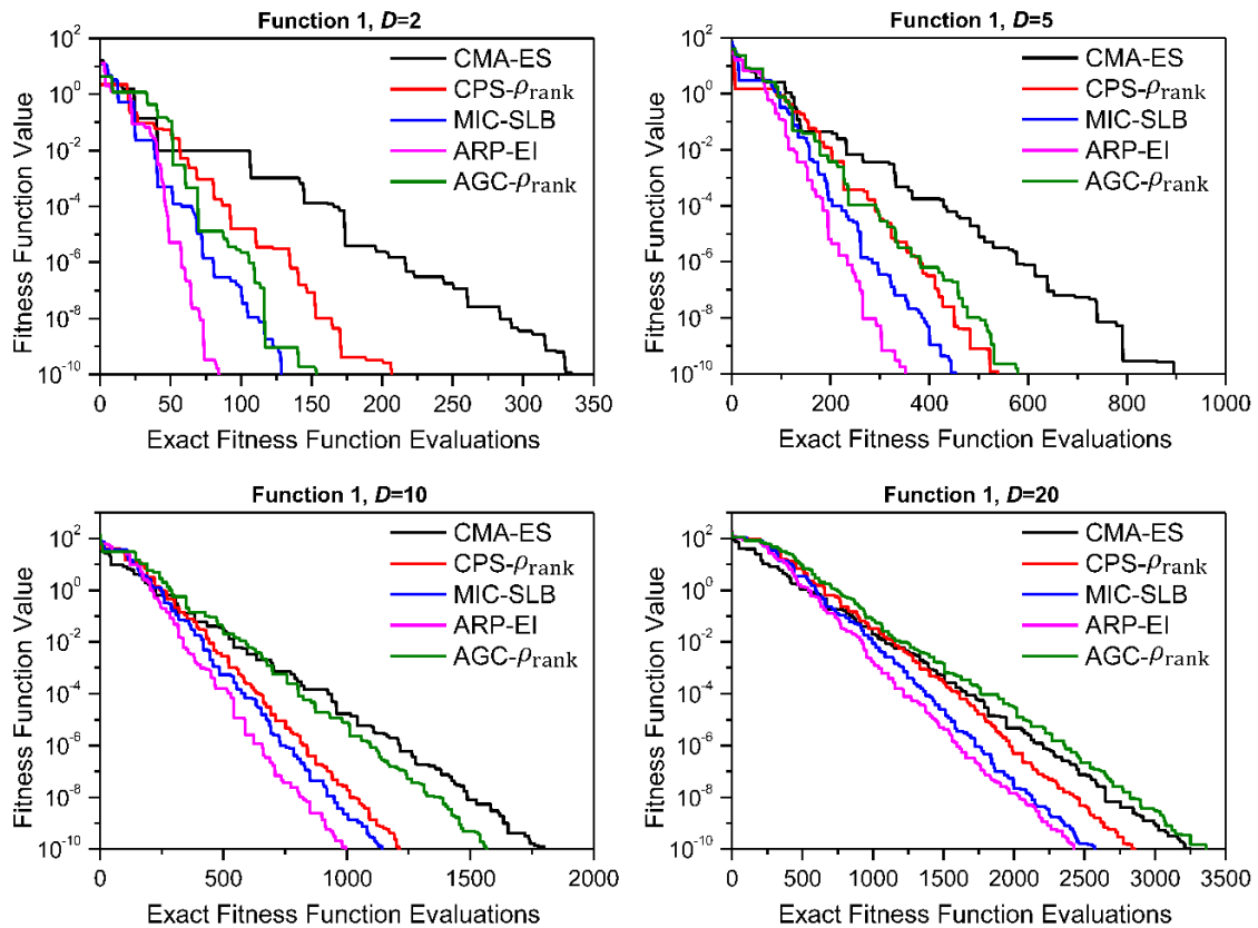
Figure 4.13 Convergence graphs of function 1
