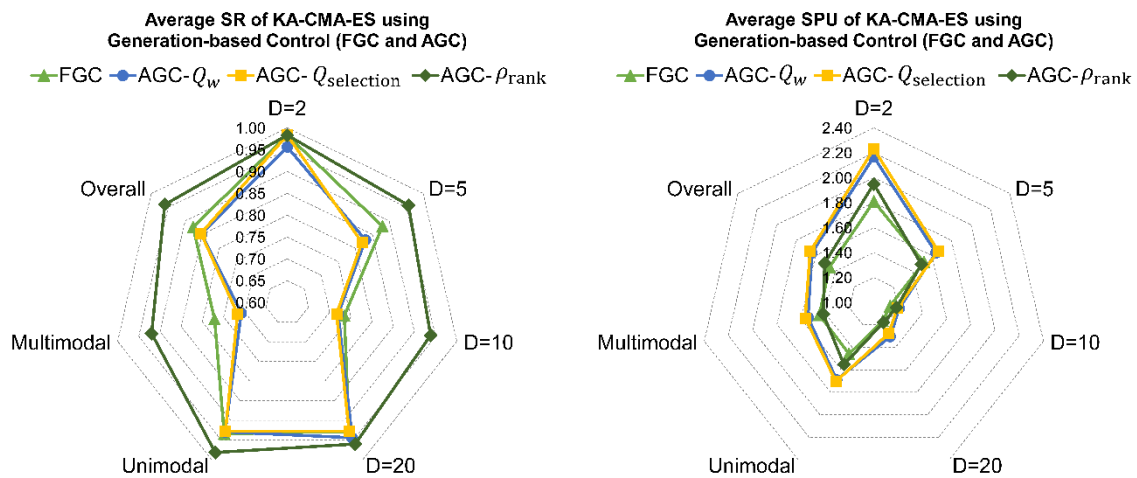
Figure 4.10 Average success rate and speedup of KA-CMA-ES using FGC and AGC.
