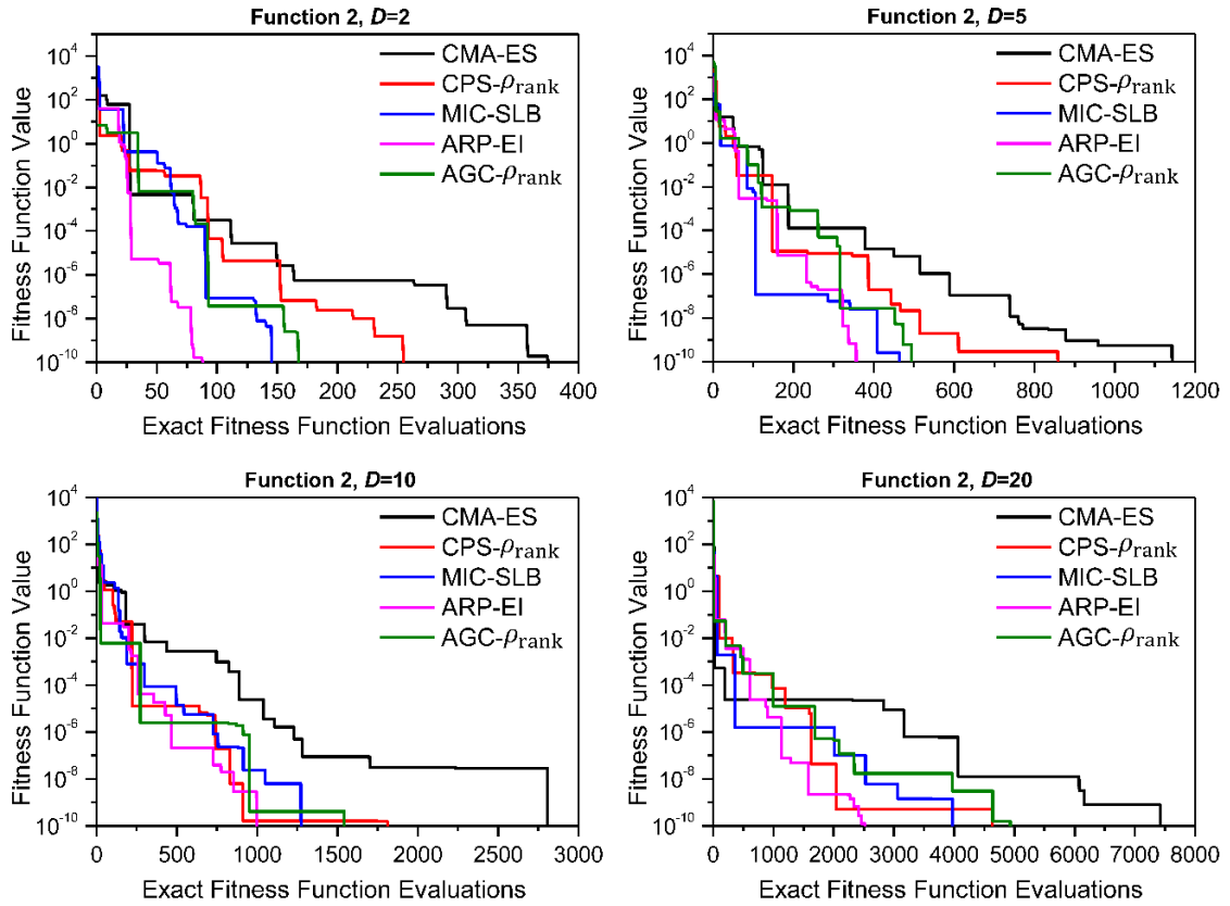
Figure 4.14 Convergence graphs of function 2
