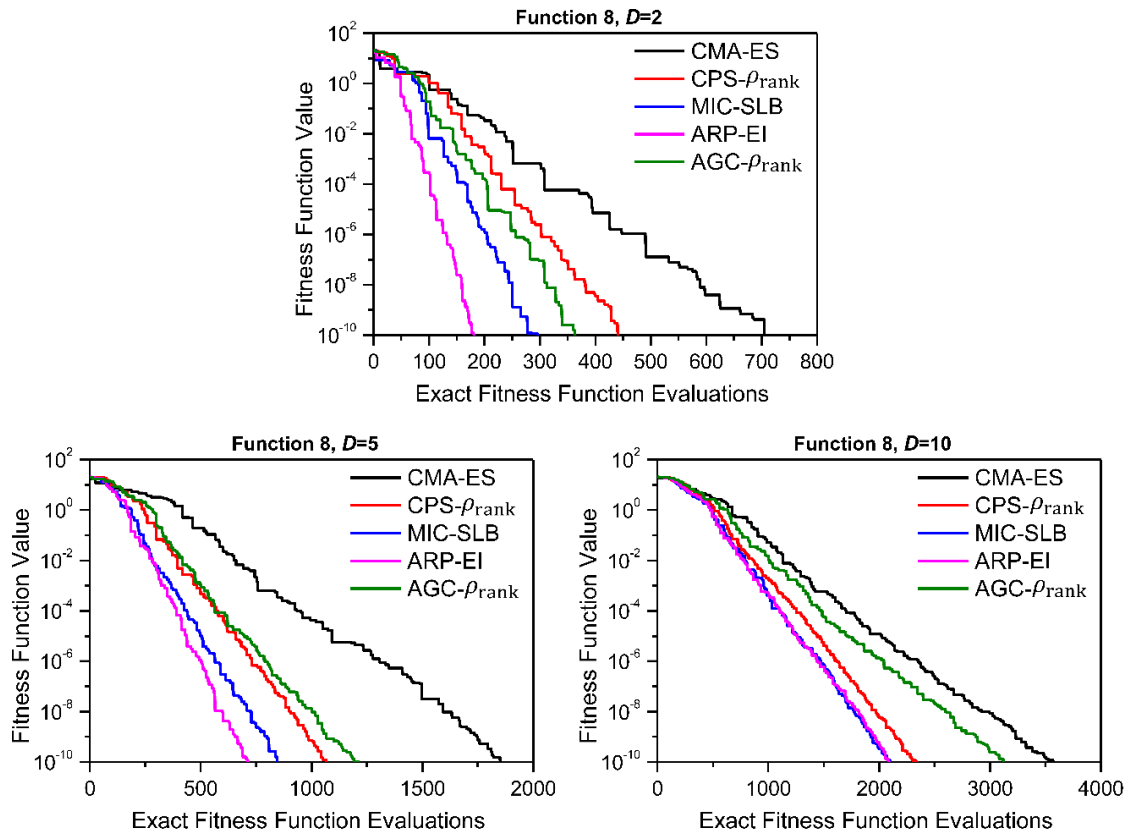
Figure 4.20 Convergence graphs of function 8
