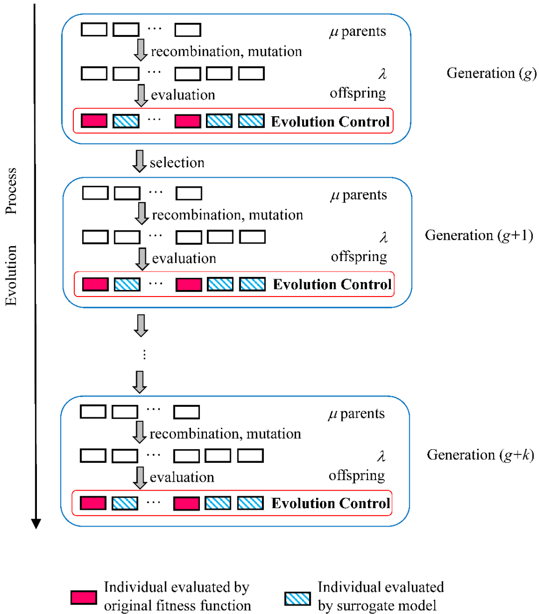
Figure 1.3 Illustration of fixed individual-based control
