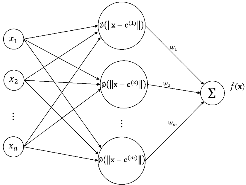
Figure 3.4 Structure of RBF network models
