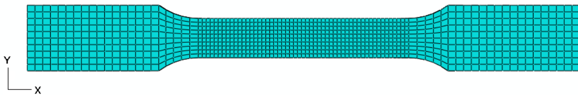
Figure 5.6 FEM model of tensile specimen
