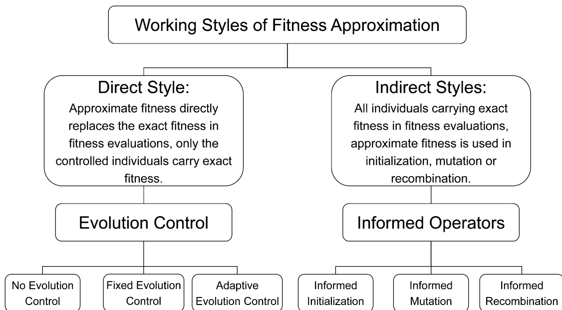
Figure 1.2 Working styles of fitness approximation
