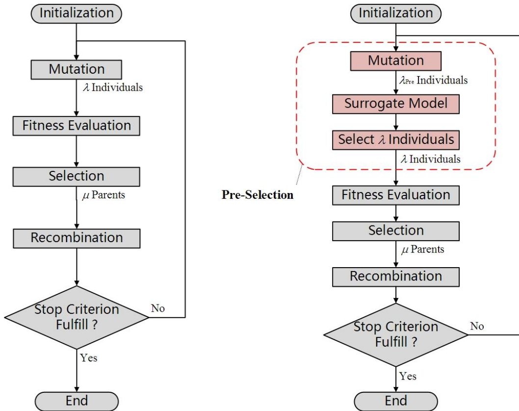
Figure 4.1 Illustration of standard (\mu, \lambda) -ES and the surrogate-assisted ES using pre-selection.
