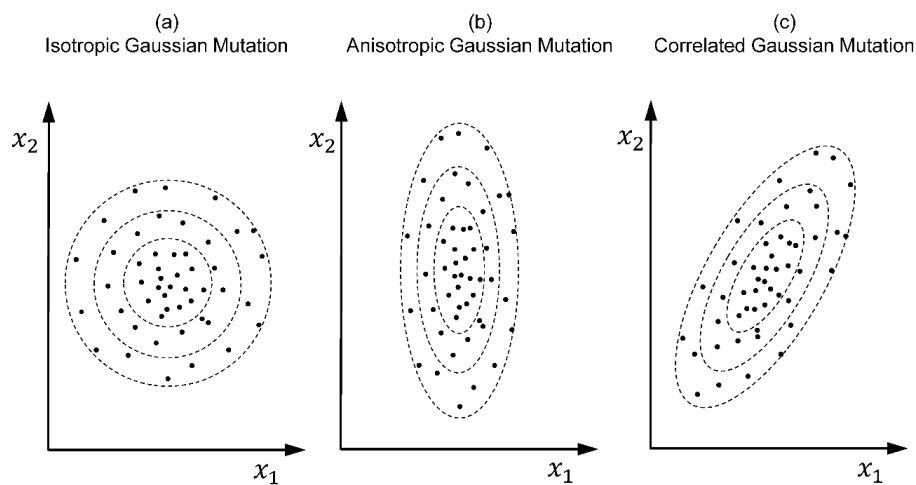
Figure 2.1 Gaussian mutation operators in evolution strategies
