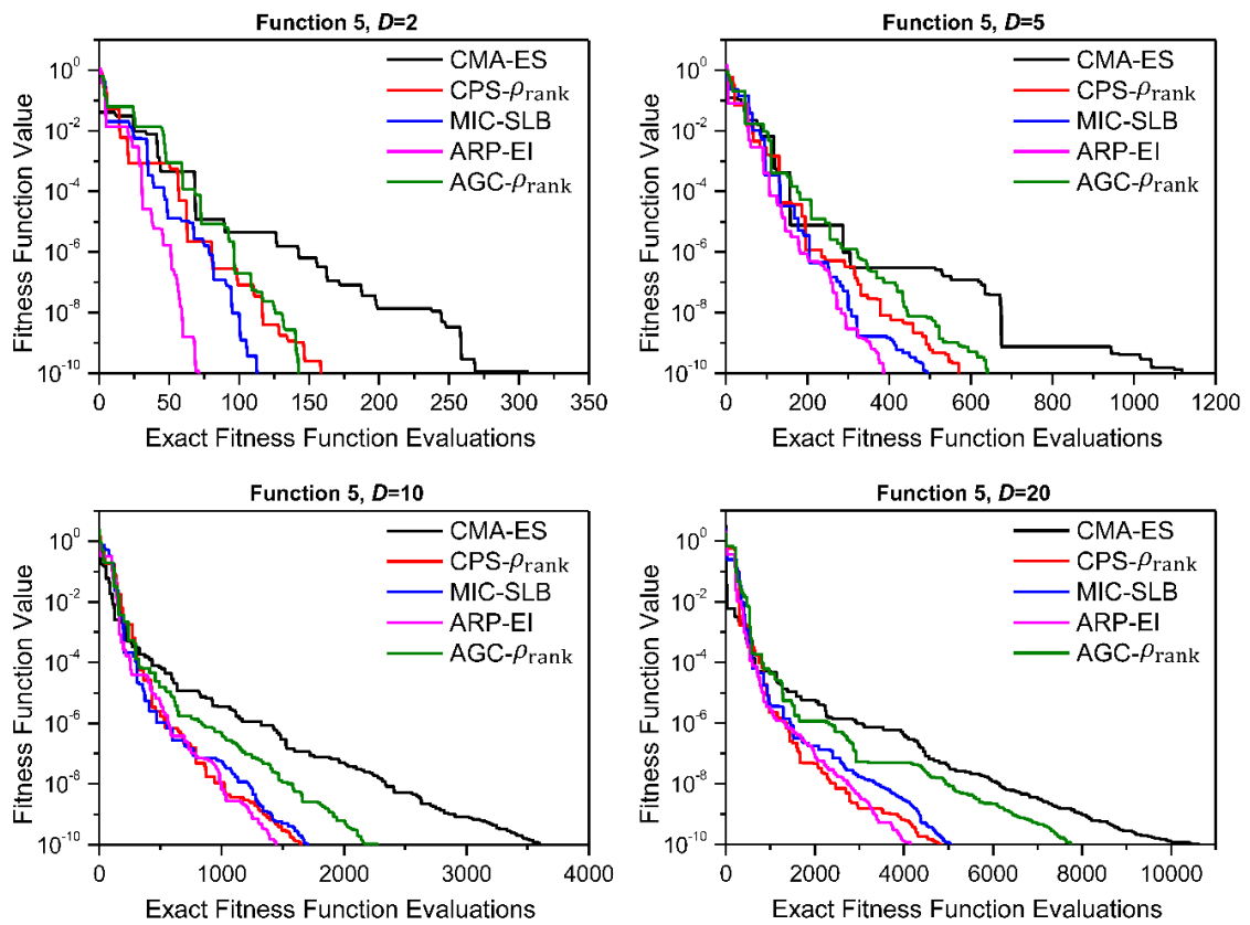
Figure 4.17 Convergence graphs of function 5
