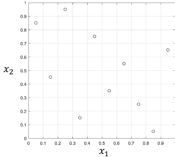
Figure 3.3 LHS realization of 10 samples in a two-dimensional design space
