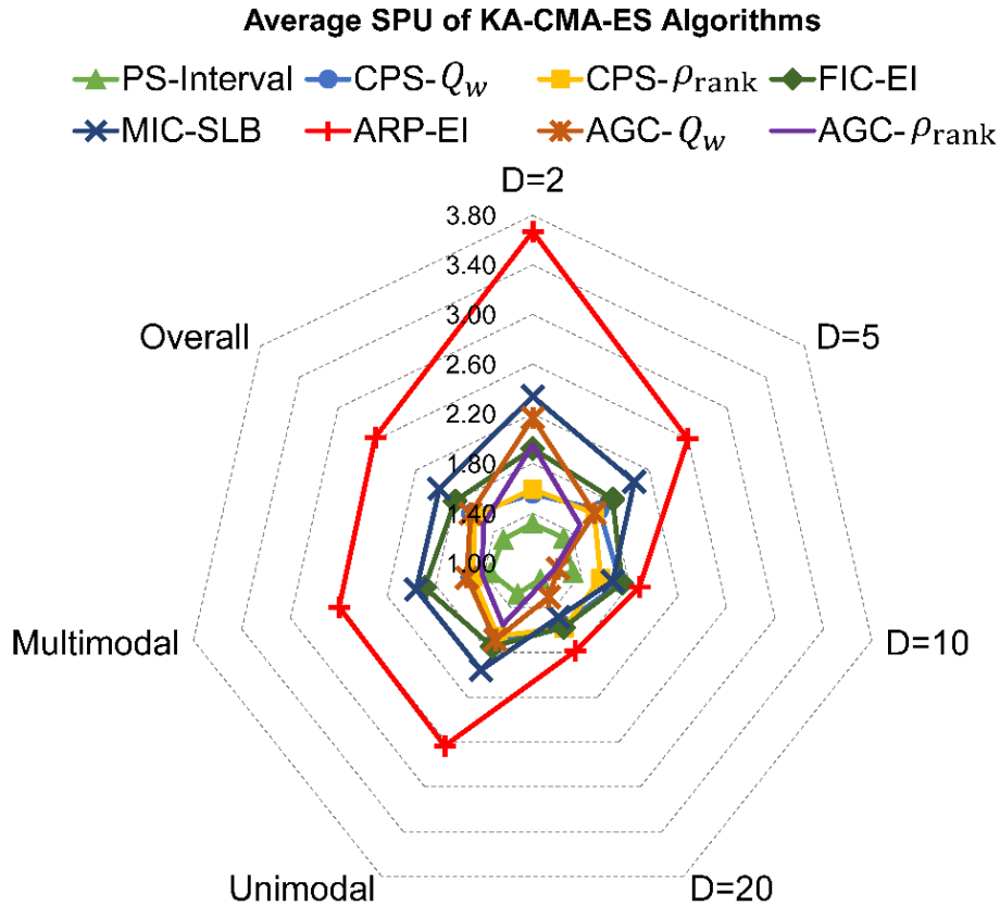
Figure 4.12 Comparison of average speedup performance (SPU) of KA-CMA-ES algorithms.
