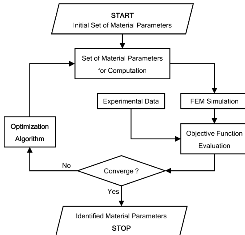
Figure 5.2 Framework of inverse method for parameter identification
