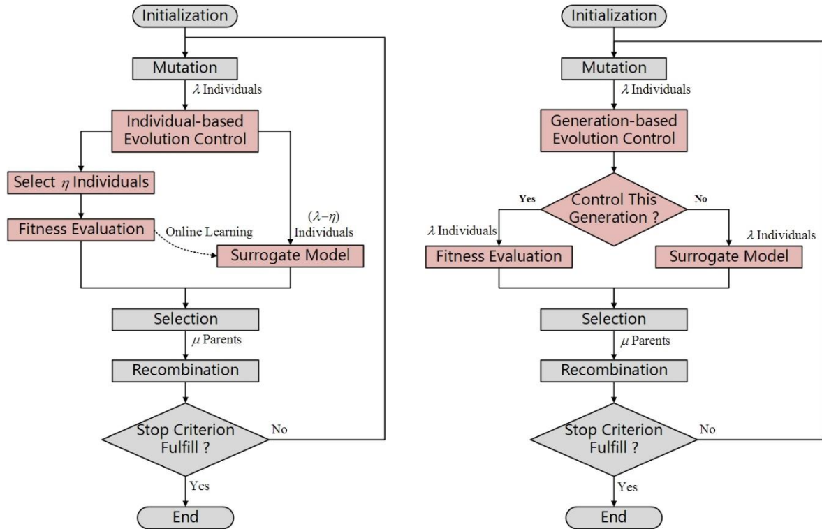
Figure 4.2 Individual-based generation-based evolution control in surrogate-assisted ES
