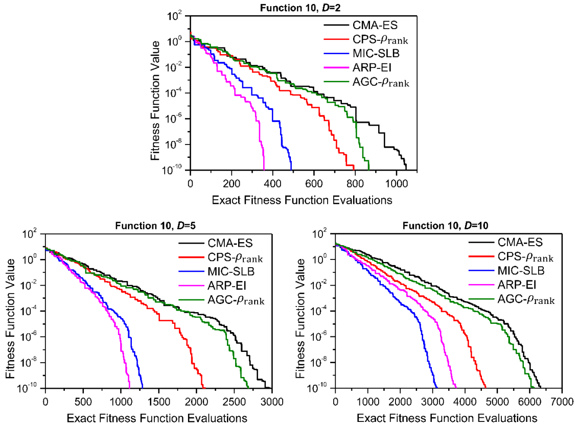
Figure 4.22 Convergence graphs of function 10
