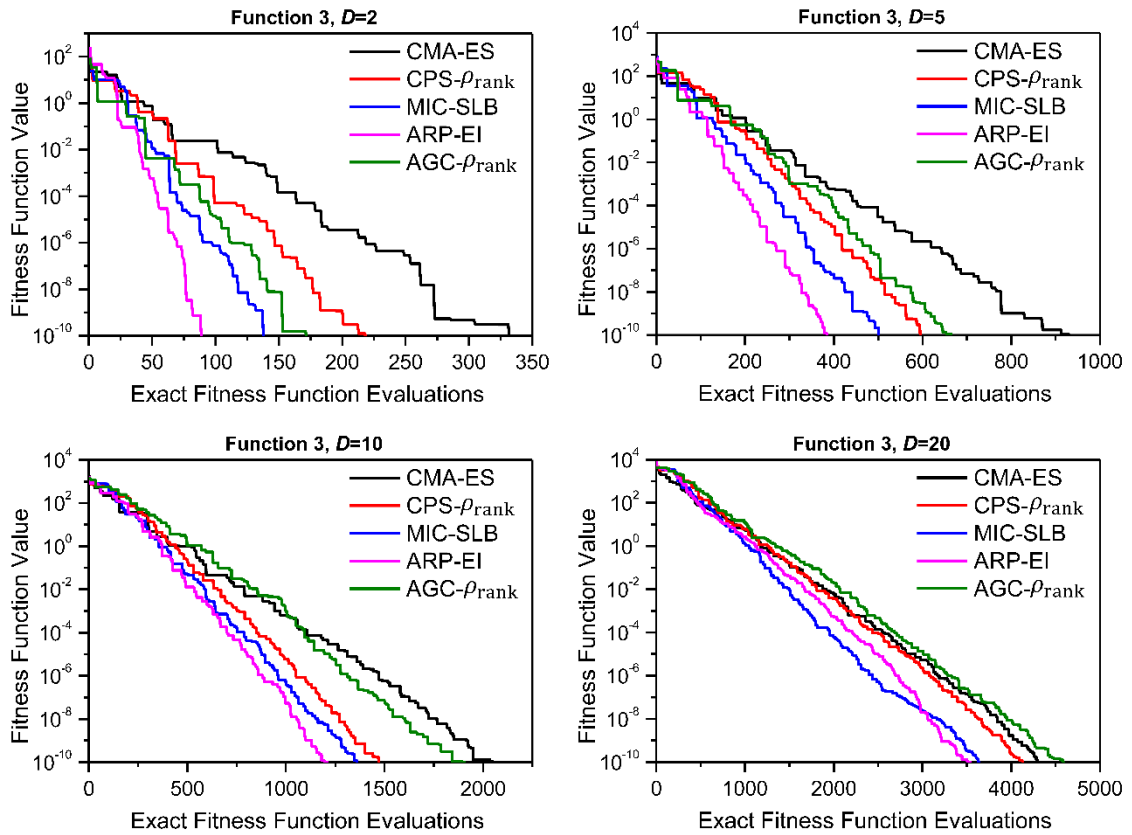
Figure 4.15 Convergence graphs of function 3
