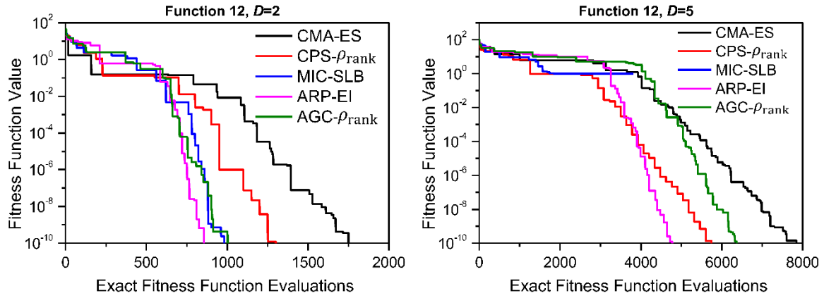
Figure 4.24 Convergence graphs of function 12
