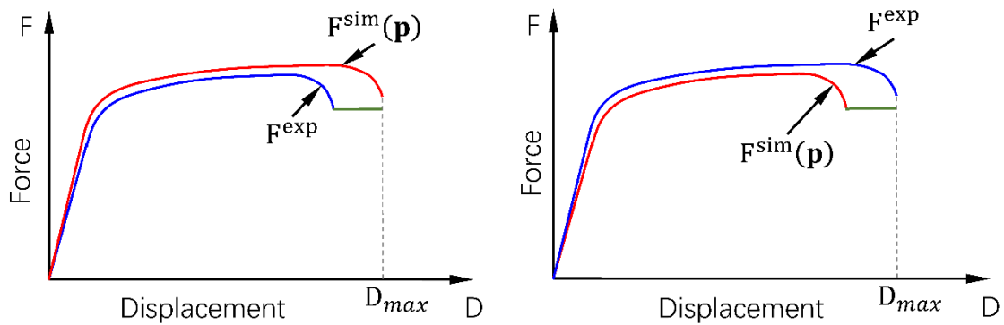
Figure 5.4 Tensile test force-displacement curve, Left: simulation fracture appears for a larger displacement than the experimental fracture displacement; Right: numerical fracture appears for a smaller displacement than the experimental fracture displacement.
