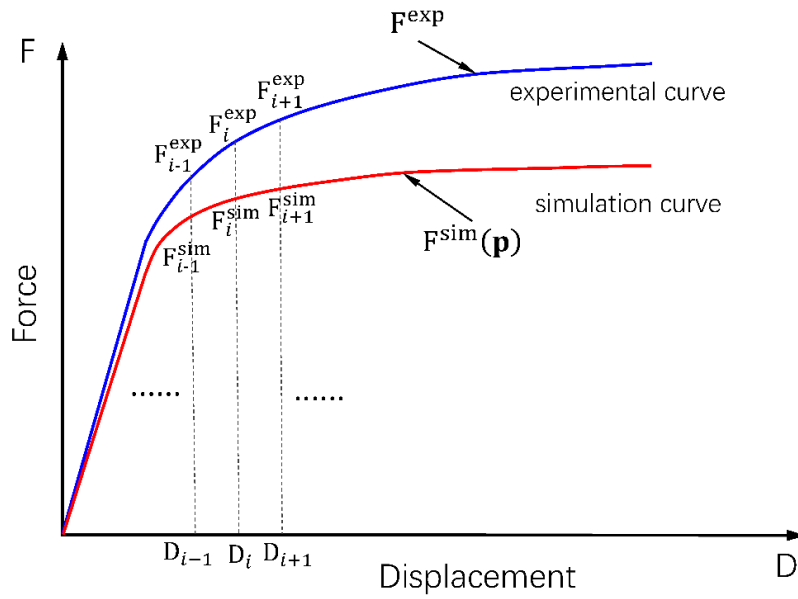
Figure 5.3 Illustration of the difference between experimental and simulation results
