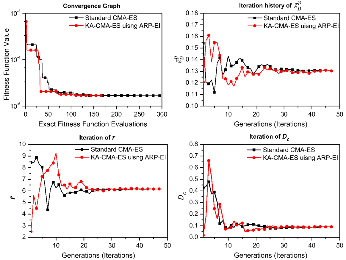
Figure 5.9 Convergence and iteration graphs of damage parameter identification
