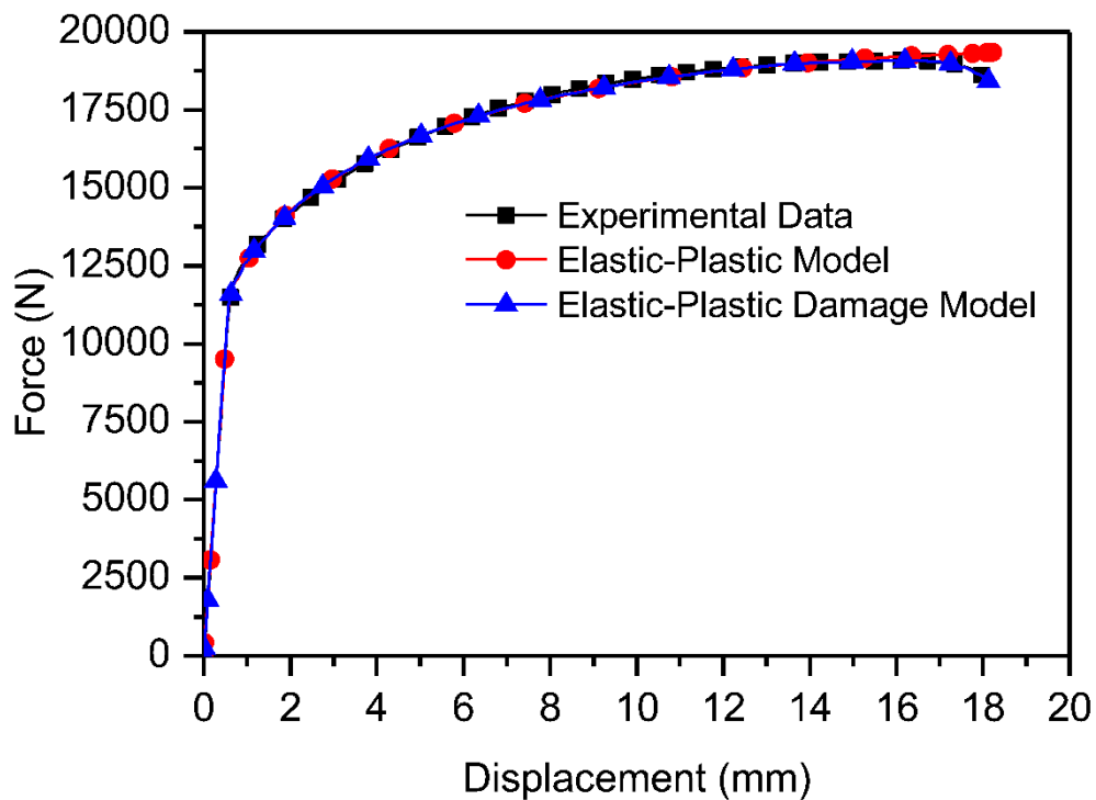
Figure 5.11 Comparison of force-displacement curves of elastic-plastic and elastic-plastic damage models with the identified parameters.
