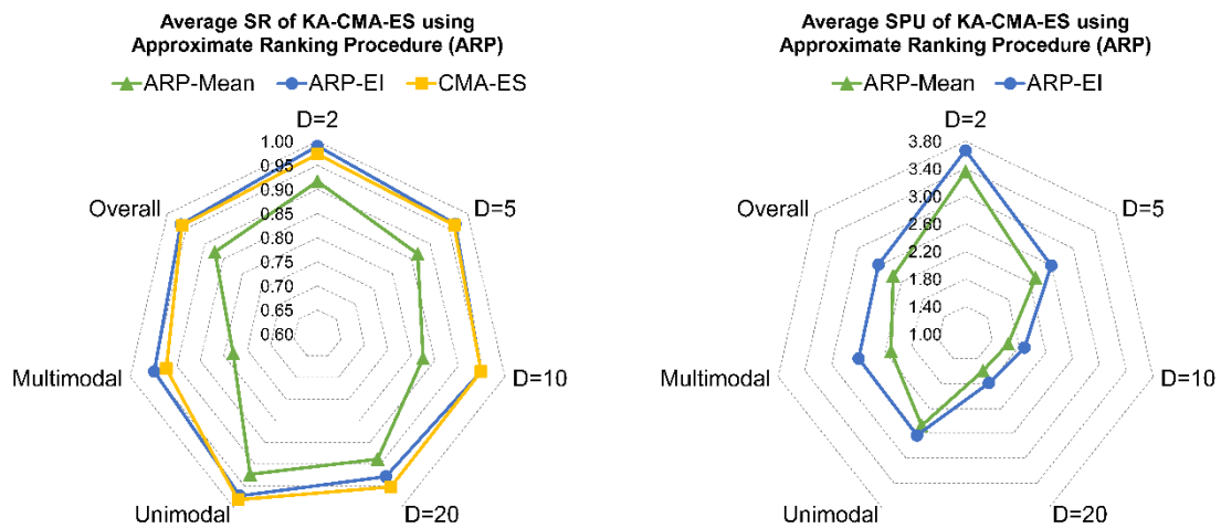
Figure 4.9 Average success rate and speedup performance of KA-CMA-ES using ARP.
