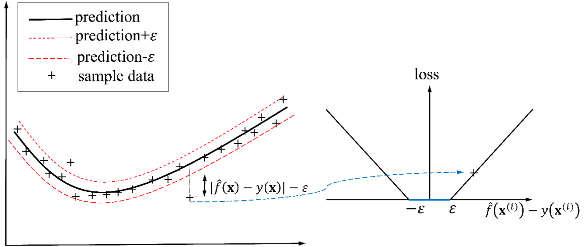
Figure 3.6 The \varepsilon -insensitive loss function for SVR
