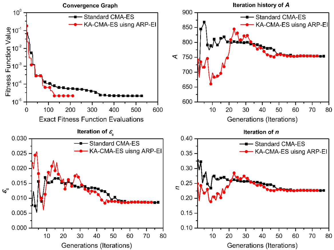
Figure 5.7 Convergence and iteration graphs of strain hardening parameter identification
