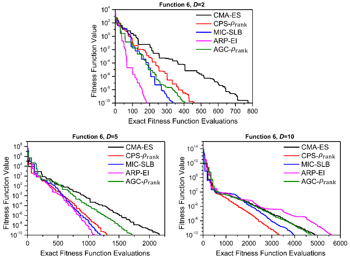
Figure 4.18 Convergence graphs of function 6
