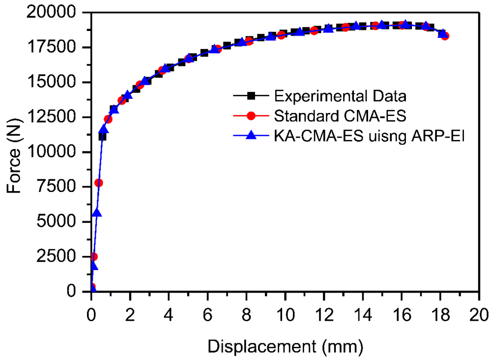
Figure 5.10 Force-displacement curves corresponding to identified damage parameters and experimental data.
