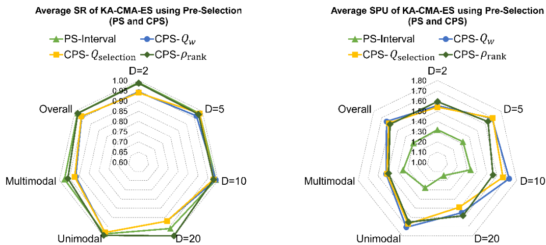
Figure 4.5 Average success rate and speedup of pre-selection without and with model impact control.
