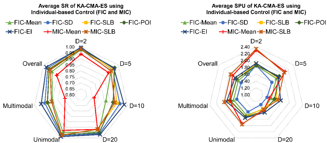
Figure 4.8 Average SR and SPU of KA-CMA-ES using fixed and mixed individual-based control (FIC and MIC).
