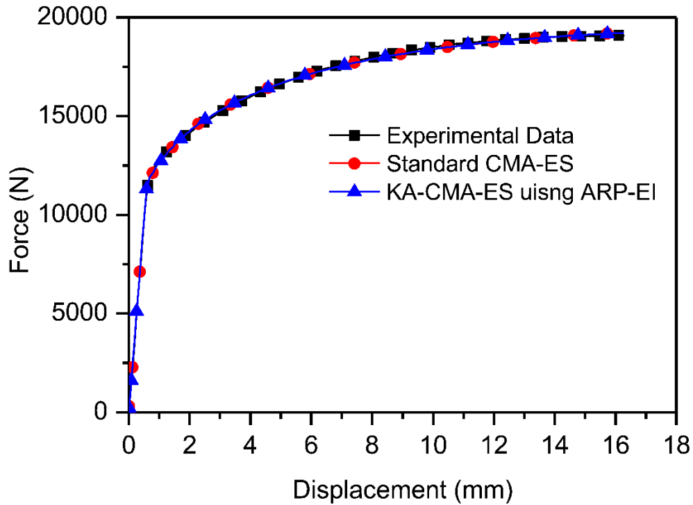
Figure 5.8 Force-displacement curves (before necking) corresponding to identified strain hardening parameters and experimental data
