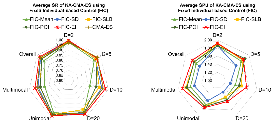
Figure 4.6 Average success rate (SR) and speedup performance (SPU) of KA-CMA-ES using fixed individual-based control with different metrics.
