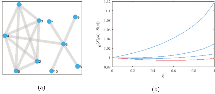
Figure 5.5: Complete-Star connected graph of size 10, (a) is the original unweighted graph, (b) Curves representing changes of the entropy according to different perturbation values introduced to edges. Each curve corresponds to a particular edge, 15 in total. The red curves indicate a decrease of the entropy after the perturbation, compared to its initial value.
