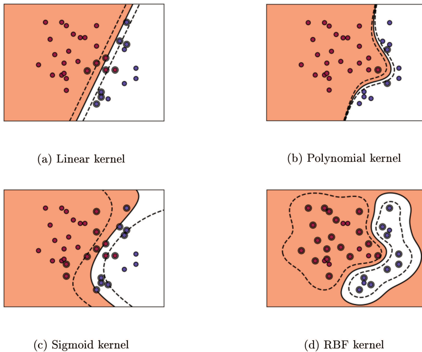
Figure 2.7: The margin and the separation boundary obtained by integrating some kernels in the SVM algorithm.
