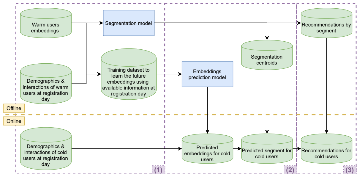
Figure 12.1: The semi-personalized user cold start recommendation framework available for online requests in our production environment, and described throughout Section 12.3. (1) Demographics and user-item interactions of a new user are concatenated, as described in Section 12.3.2, to (2) predict a user embedding vector from warm user embeddings described in Section 12.3.1. From the estimated user preferences, the new user is assigned to a segment of warm users. (3) Combining the online predicted segment with the pre-computed top items by segment, cold users benefit from semi-personalized recommendations.
