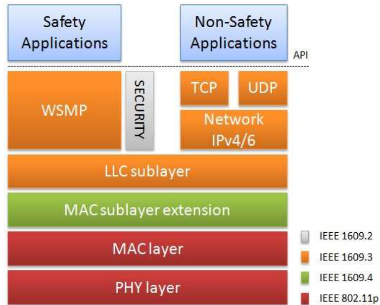
Figure 2.6: The IEEE802.11p protocol stack, according to [54].
