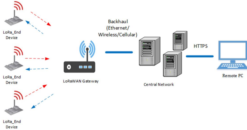
Figure 2.3: LoRaWAN network architecture.
