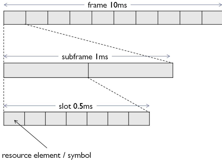
Figure 5.6: LTE frame structure: one frame consists of ten 1 ms subframes. Each subframe has 14 symbols/resource elements. Transmission time interval in legacy LTE is based on one subframe i.e. 1 ms.
