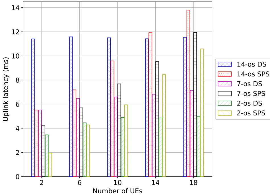
Figure 4.13: Uplink latency comparison of different TTI for V2X use case with different number of LTE-M UEs sending data periodically to eNB. 2-os TTI is clearly a better choice over legacy 14-os TTI. The short TTI can further reduce the latency to 2 ms with help of SPS but only for a very small number of devices.
