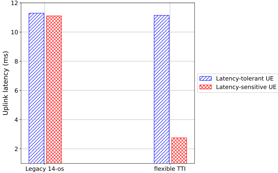
Figure 5.8: Scenario 1: Comparison of flexible TTI approach with legacy 14-os TTI. On the left side, with 14-os TTI, both UEs have almost similar latency of around 11.5 ms. However, in case of flexible TTI, the latency-sensitive UE has a latency of around 3 ms, which is achieved by using 2-os TTI.
