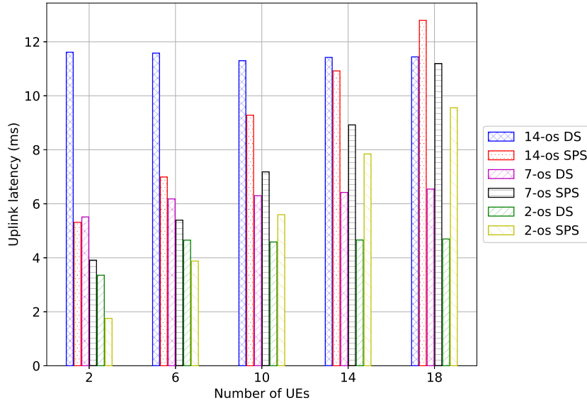
Figure 4.8: Uplink latency comparison of different TTI for industry automation use case with different number of LTE-M UEs sending data periodically to eNB. 2-os TTI is clearly a better choice over legacy 14-os TTI. The short TTI can further reduce the latency to 2 ms with help of SPS but only for a very small number of devices.
