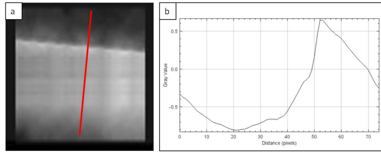
FIGURE 6.3: a) 2D wavefront reconstruction of the polycarbonate tube filled with oil b) single line plot of the wavefront performed perpendicularly to the tube surface.
