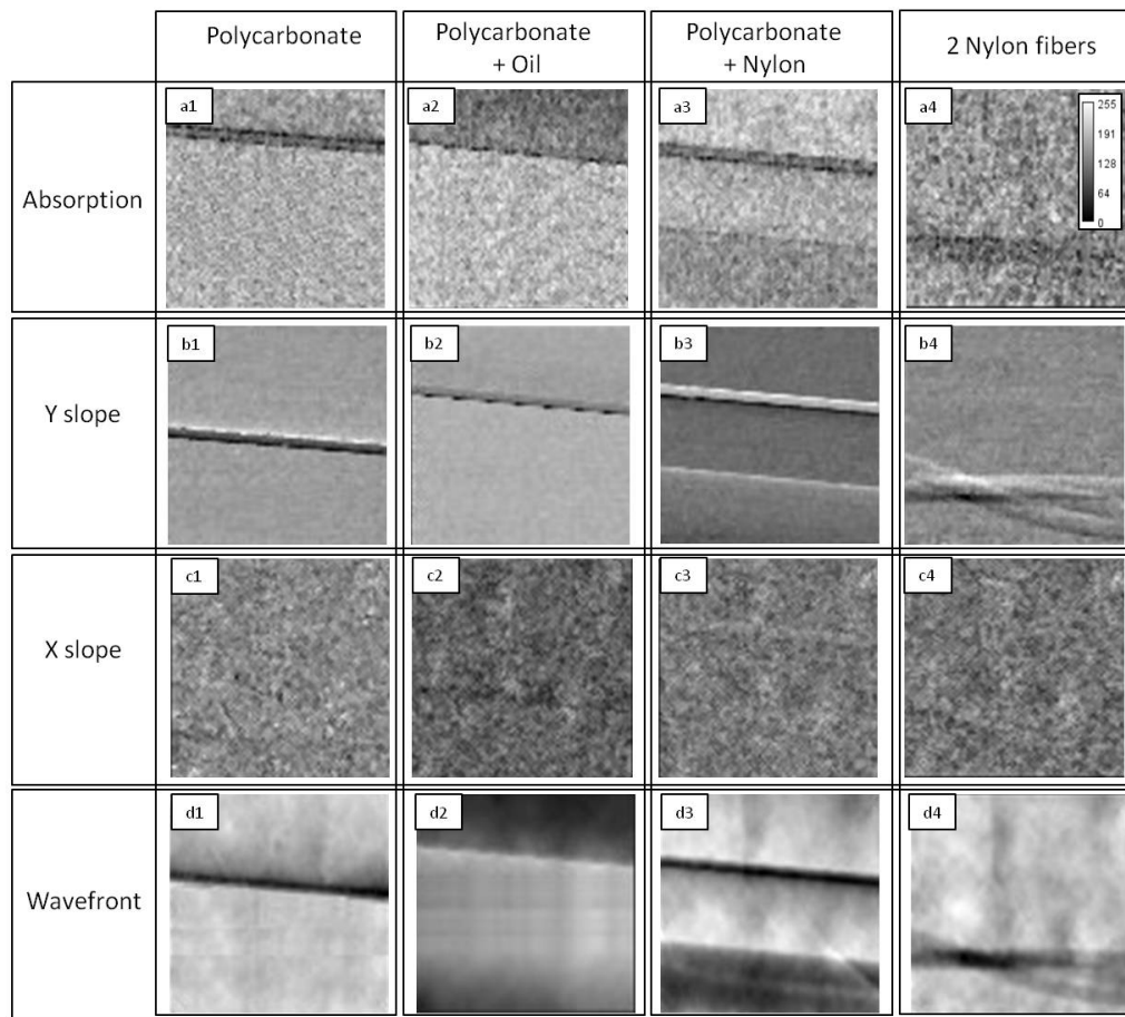
FIGURE 6.2: Images acquired with the HASO HXR Hartmann wavefront sensor from Imagine Optic. Four samples (columns) were imaged (columns): empty polycarbonate tubes (wall thickness= 50\mu\text{m} ), tube filled with oil, tube with one nylon fiber (diameter= 500\mu\text{m} ) and two nylon fibers braided together (diameter= 120\mu\text{m} ). For each sample, the absorption, the deflection in the two directions X and Y and the wavefront were reconstructed (rows). The grey scale is the same for all the images and it is shown in the panel a4).
