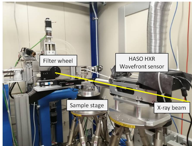
FIGURE 7.1: Picture of the set-up on Synchrotron beamline. A filter wheel was used to mount six different filters in front of the beam. The sample stage was the combination of an Hexapod and a rotational stage to allow tomographic measurements. The wavefront sensor was placed on a second Hexapod stage to allow the alignment of the Hartmann mask.
