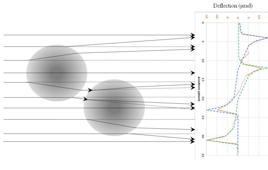
FIGURE 7.7: Explanation of the deflection profile along the x-axis for the superposition of the \text{SiO}_2 \mu spheres 7 and 8 shown in fig.7.5. The blue line corresponds to one sphere and the green to the other sphere alone. The orange line is the resulting deflection considering the two spheres.
