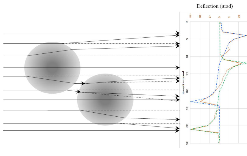
FIGURE 7.7: Explanation of the deflection profile along the x-axis for the superposition of the \text{SiO}_2 \mu\text{spheres} 7 and 8 shown in fig.7.5. The blue line corresponds to one sphere and the green to the other sphere alone. The orange line is the resulting deflection considering the two spheres.
