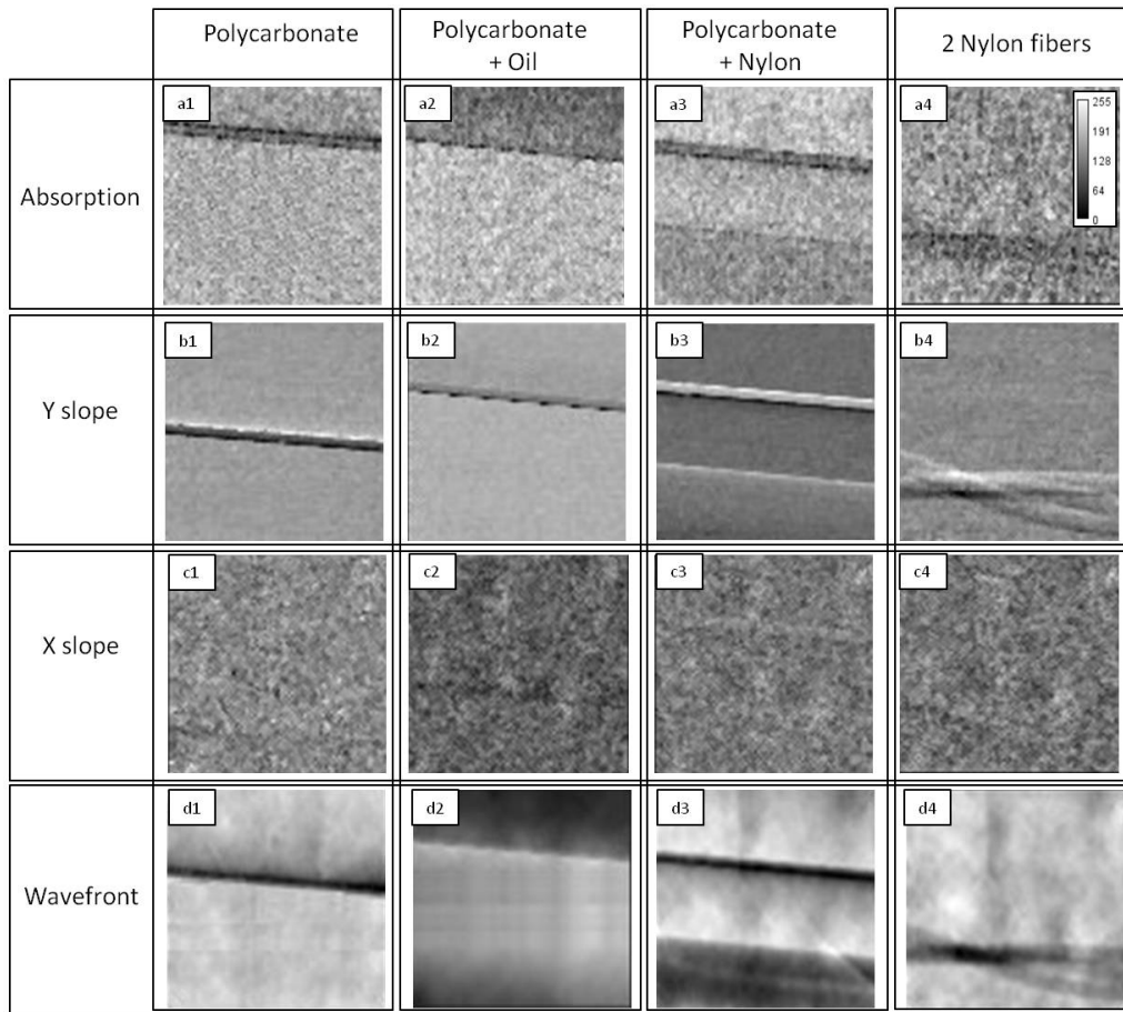
FIGURE 6.2: Images acquired with the HASO HXR Hartmann wavefront sensor from Imagine Optic. Four samples (columns) were imaged (columns): empty polycarbonate tubes (wall thickness = 50\mu\text{m} ), tube filled with oil, tube with one nylon fiber (diameter = 500\mu\text{m} ) and two nylon fibers braided together (diameter = 120\mu\text{m} ). For each sample, the absorption, the deflection in the two directions X and Y and the wavefront were reconstructed (rows). The grey scale is the same for all the images and it is shown in the panel a4).
