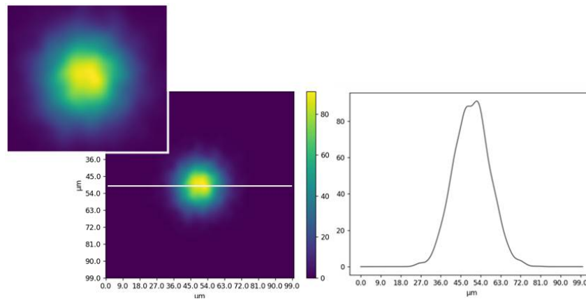
FIGURE 5.17: Simulation of an incoherent source (left) and a single line plot corresponding to the white line (right). Screen size L=100 \mu\text{m} , \lambda = 1.38 \times 10^{-10} \text{ m} , M \times M samples with M=1000 , propagation distance z=20 \text{ cm} .
