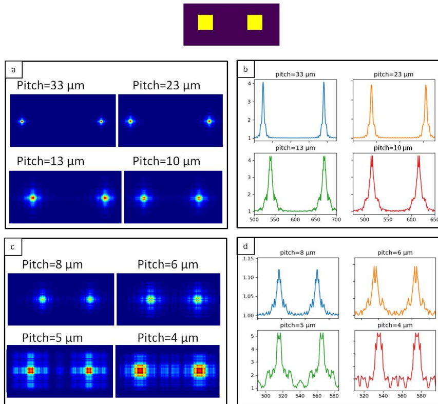
FIGURE 5.34: Top: Design of two square apertures with side= 3\ \mu\text{m} . a) Images obtained varying the pitch, putting the apertures progressively closer. Pitch from 33\ \mu\text{m} to 10\ \mu\text{m} . b) Single line plot corresponding to the images shown in a). c) Images obtained varying the pitch: pitch from 8\ \mu\text{m} to 4\ \mu\text{m} . d) Single line plot corresponding to the images shown in c). The scale is different for plots in b) and d), since varying the pitch will change the relative distance of the peaks.
