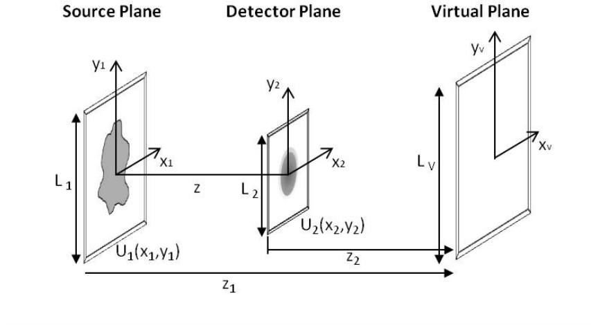
FIGURE 5.13: Fresnel two-step propagation concept
