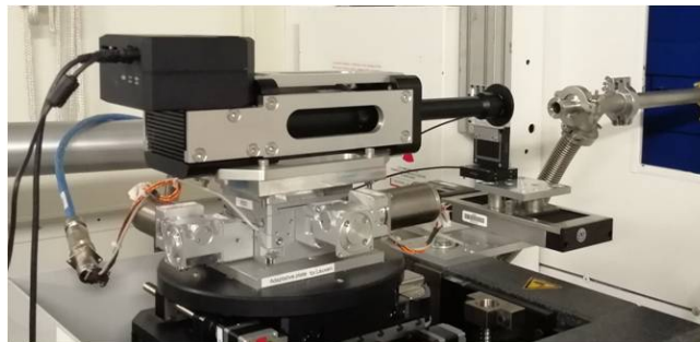
FIGURE 7.19: Picture of the Hartmann X-ray phase imaging system as installed in the BM05 beamline of ESRF.
