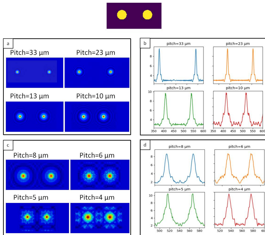
FIGURE 5.35: Top: Design of the two circular apertures with diameter= 3 \mu\text{m} . a) Images obtained varying the pitch, putting the apertures progressively closer. Pitch from 33 \mu\text{m} to 10 \mu\text{m} . b) Single line plot corresponding to the images shown in a). c) Images obtained varying the pitch: pitch from 8 \mu\text{m} to 4 \mu\text{m} . d) Single line plot corresponding to the images shown in c). The scale is different for plots in b) and d), since varying the pitch will change the relative distance of the peaks.
