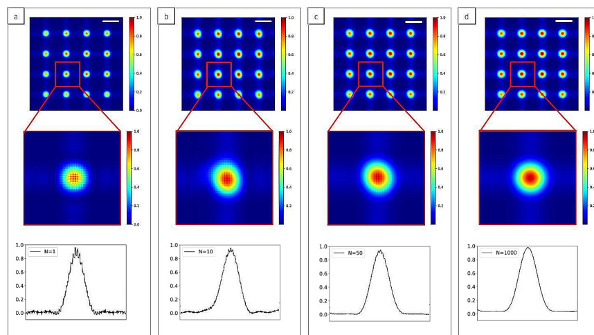
FIGURE 5.24: 2D Intensity map of Hartmann mask with 3 \mu\text{m} square apertures and 25 \mu\text{m} pitches for different illuminating sources. The number of Gaussians N inside the source are N = 1 (a), N = 10 (b), N = 50 (c) and N = 1000 (d). Oscillations can be seen in the detected spots with coherent illumination (a) while they become quite smooth in the incoherent case (d). White scale bars are 38 \mu\text{m} .
