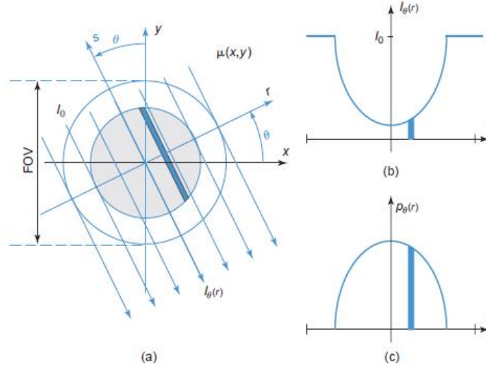
FIGURE 4.2: a) Parallel-beam geometry with coordinate systems. The X-ray beams make an angle \theta with the y-axis and are at distance r from the origin. b) An intensity profile I_\theta(r) is measured for every view (defined by an angle \theta ). I_0 is the unattenuated intensity. c) The attenuation profiles p_\theta(r) , obtained by log-converting the intensity profiles I_\theta(r) , are the projections of the function \mu(x, y) along the angle \theta . Image adapted from (Flower, 2012).
