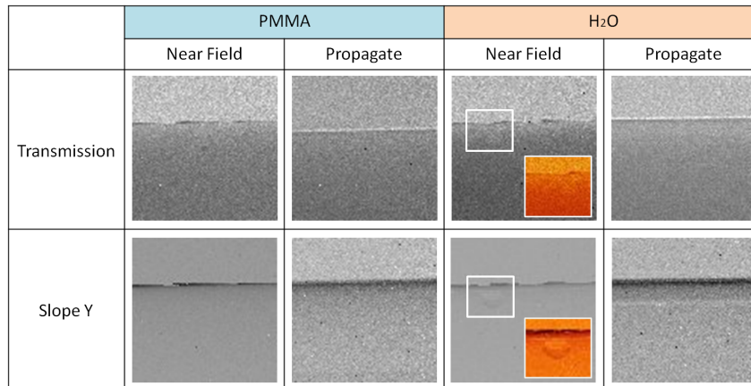
FIGURE 6.11: Images acquired with the HASO HXR Hartmann wavefront sensor from Imagine Optic varying the relative distance between the sample and the wavefront sensor. We defined as near field image the one acquired with distance sample-detector is 6 cm, while for the propagate field the distance sample-detector is 27 cm. Both the transmission and the deflection on the Y axis are presented. Magnification: it was possible to see the presence of an air bubble inside the tube in the deflection image that cannot be resolved in the corresponding transmission image.
