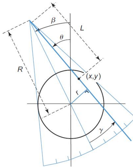
FIGURE 4.7: Cone beam geometry with detector placed on a circular arc: \beta is the angle between the center line of the cone and the y-axis, \gamma is the angle between the center line and the ray through point (x, y) . L is the distance from the source to (x, y) . Image from Suetens, 2009.
