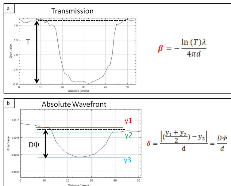
FIGURE 7.9: Example of the profile plot of the \mu spheres used to calculate the \beta and \delta components of the refractive index. a) The value of \beta was calculated from the transmission image, obtained as the ratio between the intensity recorded with the sample and the reference intensity without the sample. The formula used is reported on the right, where T is the transmission, \lambda the wavelength and d is the sphere diameter. b) The value of \delta was calculated from the experimental phase difference ( D\Phi ) divided by the sphere diameter d .
