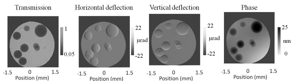
FIGURE 7.20: False color maps of the transmission, horizontal and vertical deflection, and phase measured at 12 keV for the set of 8 spheres.
