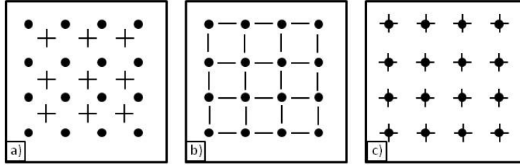
FIGURE 5.9: Slope measurement sampling geometry and wavefront mesh points. The horizontal lines indicate positions of x -slope sampling. The vertical lines are the y -slope sampling positions. The dots are the estimated phase points. Configuration (a) is from Southwell, (b) is from Hudgin and (c) is from Fried.
