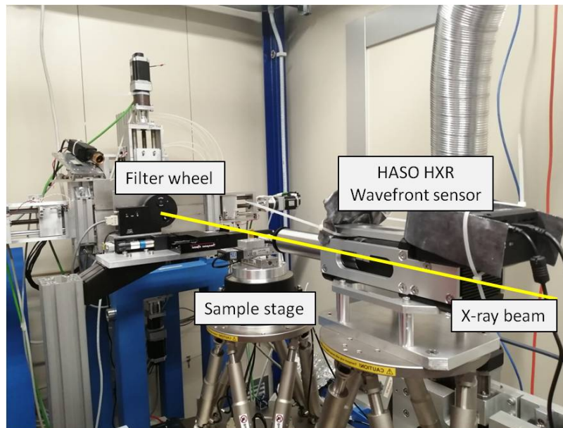
FIGURE 7.1: Picture of the set-up on Syrmep beamline. A filter wheel was used to mount six different filters in front of the beam. The samples stage was the combination of an Hexapod and a rotational stage to allow tomographic measurements. The wavefront sensor was placed on a second Hexapod stage to allow the alignment of the Hartmann mask.
