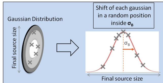
FIGURE 5.15: Description of source architecture: each Gaussian beam is first shifted to a random position chosen inside a larger Gaussian distribution (with standard deviation \sigma_B ) that defines the final source size.
