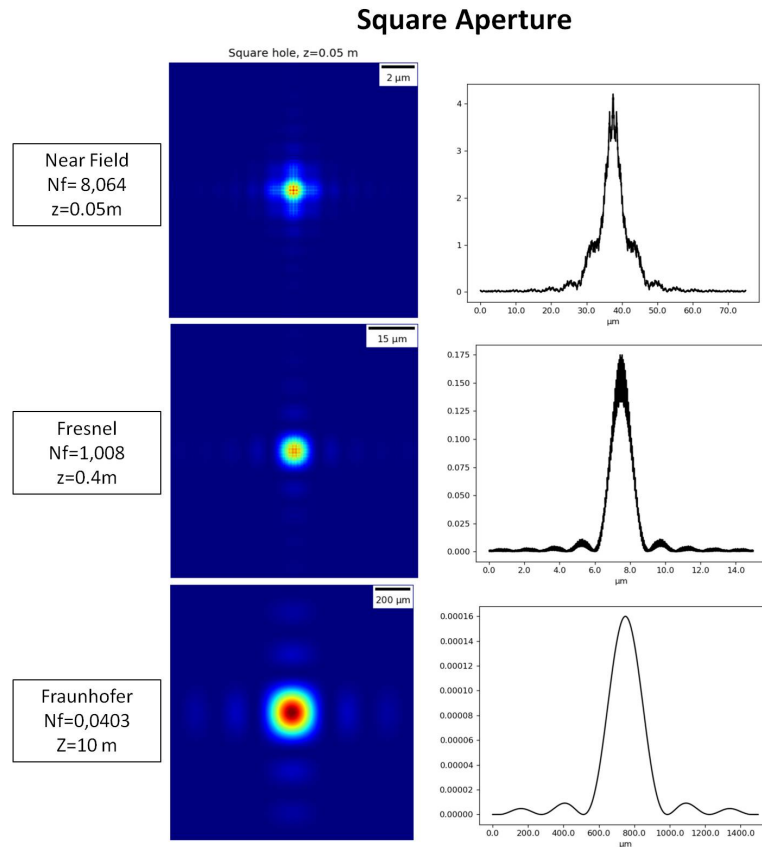
FIGURE 5.30: Diffraction patterns from a square aperture a=3\mu m , considering a wavelength \lambda = 6.2 \times 10^{-11} and different propagation distances z=0.05, 0.4, 10 m. The 2D images and the corresponding line plots are reported for three diffraction regimes: for the near field regime ( N_f = 8.064 ), the Fresnel diffraction regime ( N_f = 1.008 ) and the Fraunhofer regime ( N_f = 0.0403 ).
