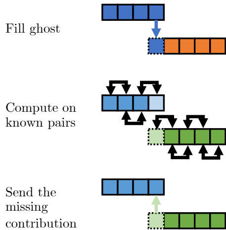
Figure 3.2: Schematic representation of the half-ghost communication pattern
