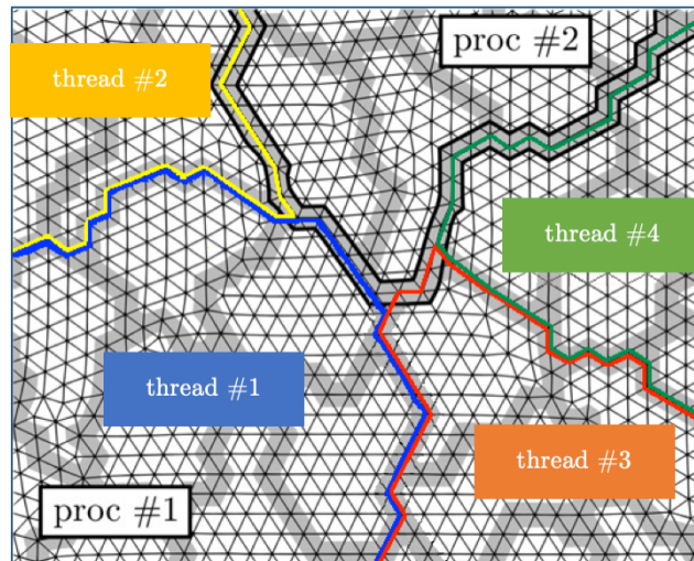
Figure 4.1: Work distribution with OpenMP fine grain model: each thread is in charge of a subset of EIGrps during computation.
