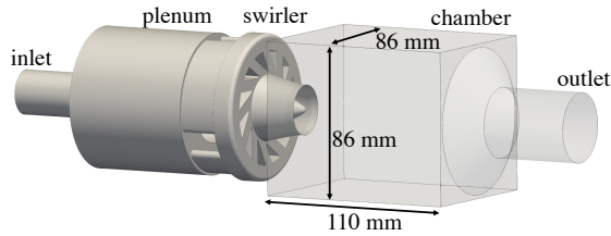
Figure 2.12: PRECCINSTA burner
