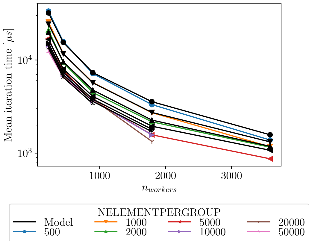
Figure 2.45: Model for the fine grid iteration cost of Preccinsta 110M on MYRIA
