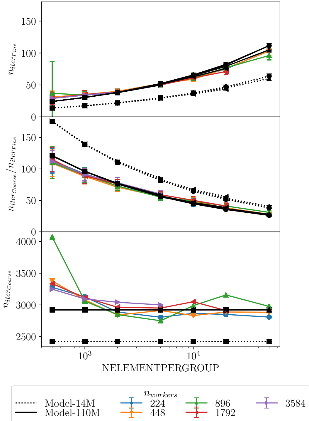
Figure 2.44: Model for the number of iterations applied to Preccinsta 110M
