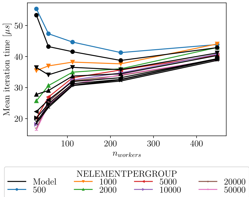
Figure 2.41: Resulting model for the deflation iteration for Preccinsta 14M on MYRIA
