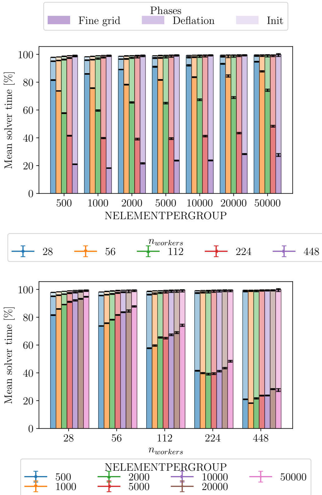
Figure 2.28: Breakdown of the DPCG solver time into fine grid, deflation and initialisation for Precinsta 14M on MYRIA. The error bars represent the standard deviation of the measured time across the different workers
