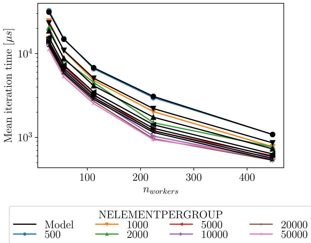
Figure 2.39: Resulting model for the iteration on the fine grid for Preccinsta 14M on MYRIA
