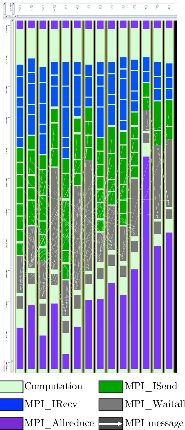
Figure 3.9: TAU trace of a deflation iteration with the graph data structure
