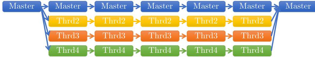
Figure 5.1: OpenMP coarse grain mechanism. The entire code is into one parallel region and all threads both compute and communicate.
