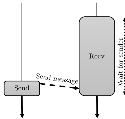
Figure 1.6: Blocking communication: late sender
