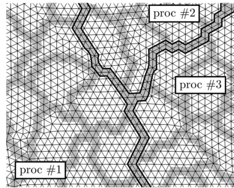
Figure 2.3: Double domain decomposition
