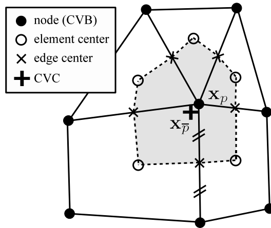
Figure 2.1: Control Volume in YALES2: x_p is the point around which it is built and \bar{x}_p is its barycentre.
