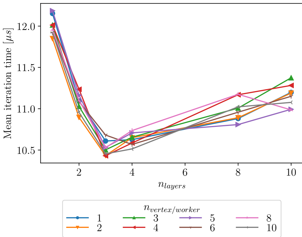
Figure 3.15: Average deflation iteration time with multiple ghost layers on channel benchmark
