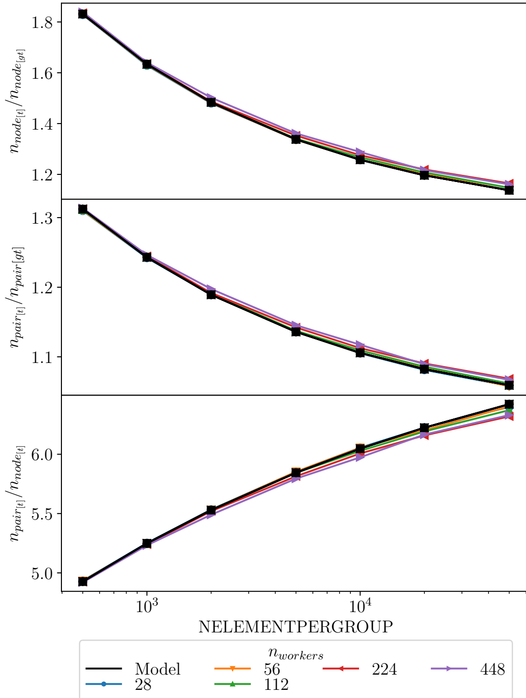
Figure 2.36: Models of the grid size variation with NELEMENTPERGROUP for Precinsta 14M
