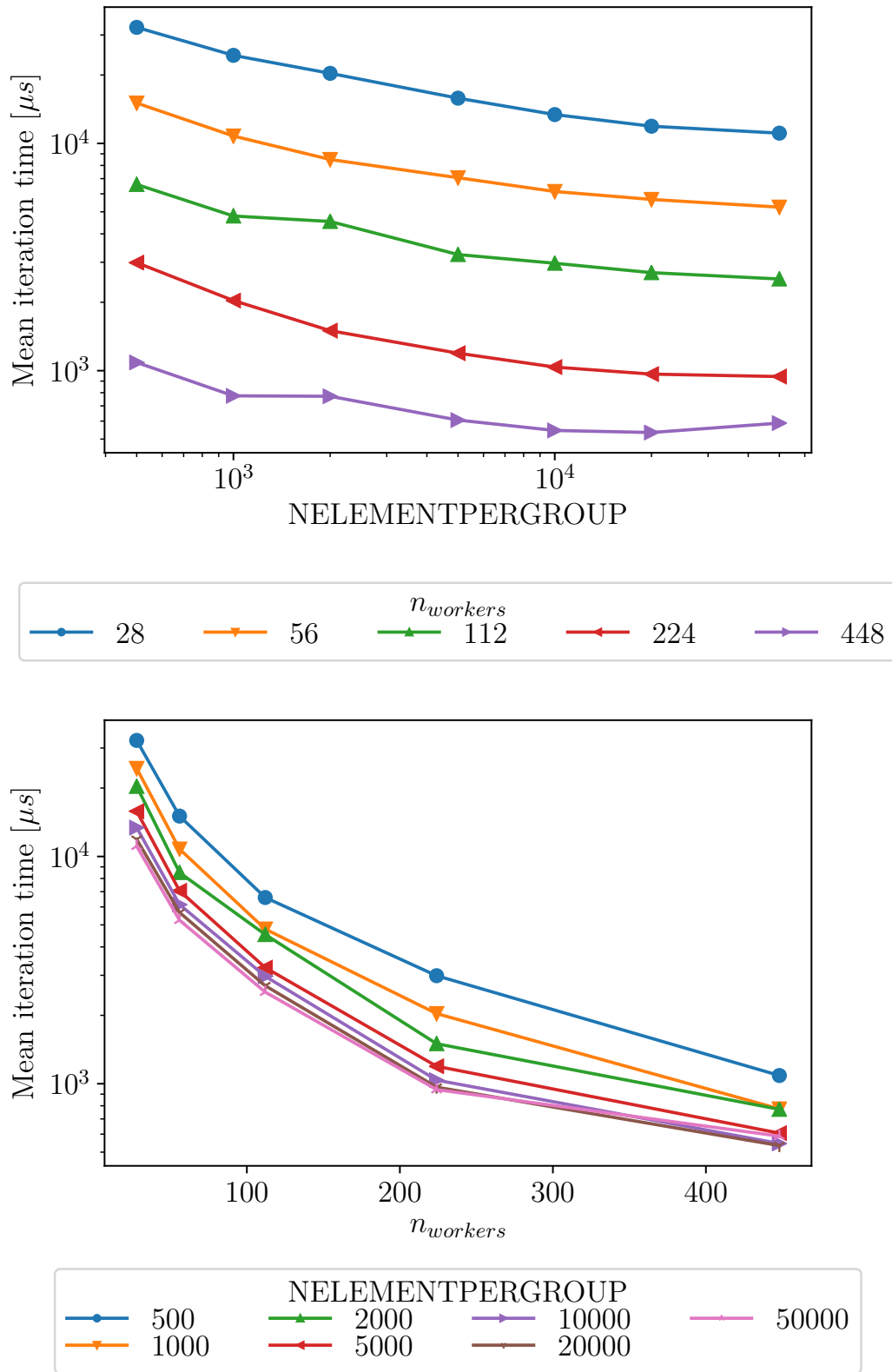
Figure 2.30: Fine grid iteration time as a function of NELEMENTPERGROUP and n_{workers} for Preccinsta 14M on MYRIA
